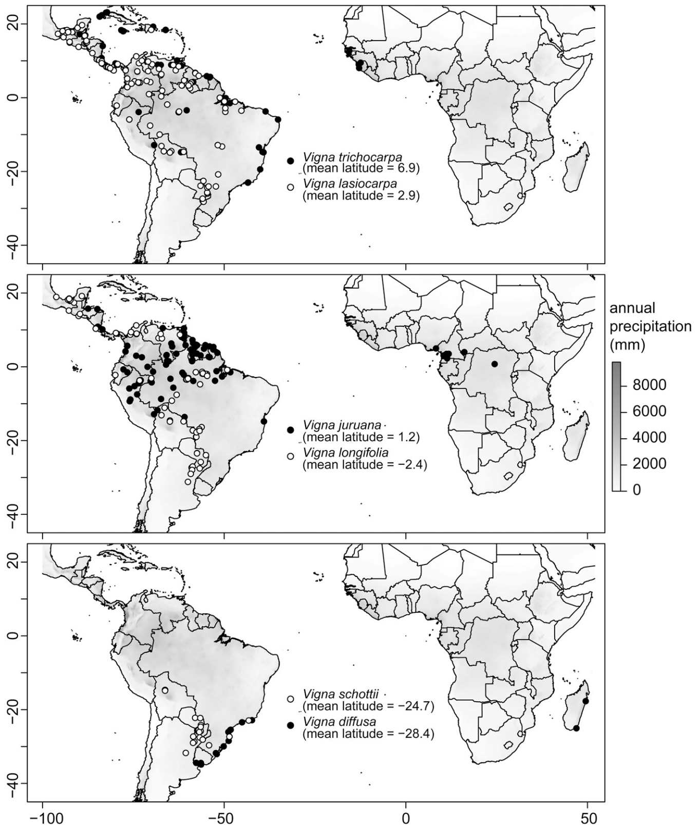
FIG. 3. Geographic distributions of the six species of Vigna subg. Laiospron , which are ordered, top to bottom, by mean latitude. Filled circles indicate species with an amphiatlantic distribution.
