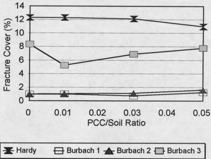
Figure 2. Fracture cover as a percentage of soil area.
