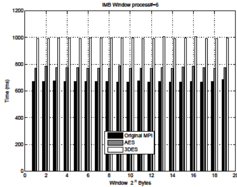
Fig. 12: Intel Micro Benchmark Window 6 nodes
