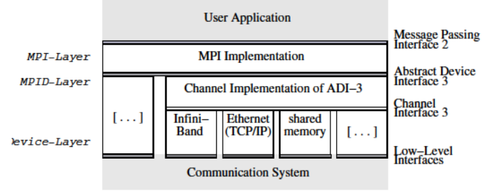
Fig. 1: Hierarchical Structure of MPICH2 [14]
