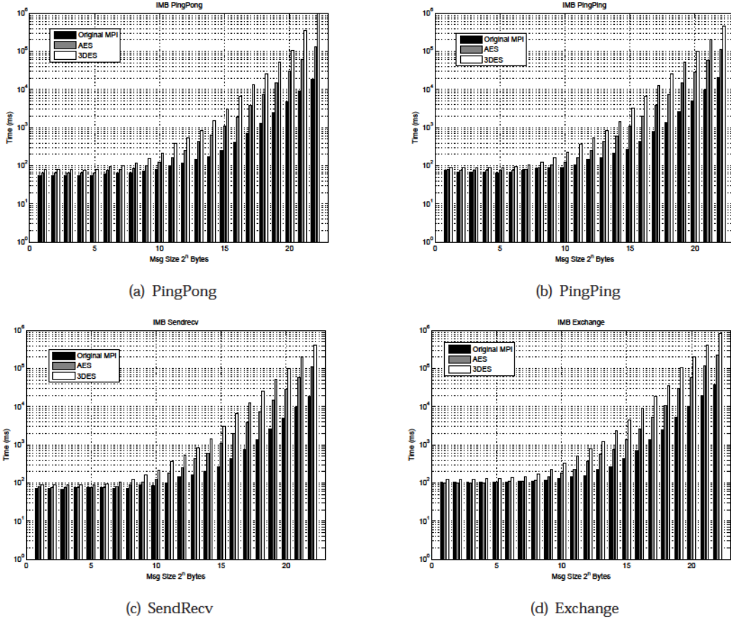
Fig. 9: Intel MPI Benchmarks, PingPong and PingPing are Single Transfer Benchmarks, SendRecv and Exchange are Parallel Benchmarks on 6-node Cluster of Intel Celeron
