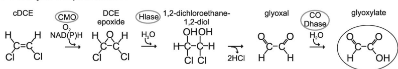
FIG. 6. Proposed cDCE degradation pathways.
