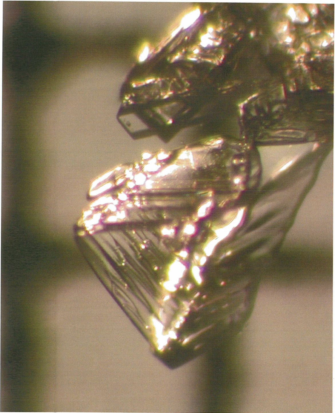
Figure 4.28: A 1.5 mm near-surface faceted crystal harvested from the south-facing study site on 13 January 2004. This crystal is classified by Colbeck et al. (1990) as type 5a, cup shaped crystal.
