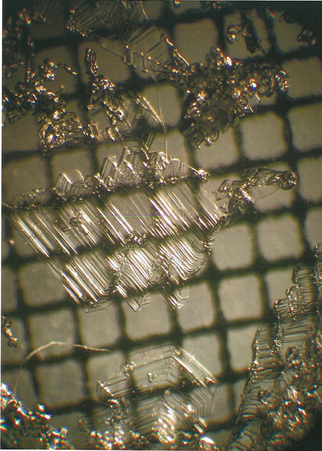
Figure 4.1: A 6mm surface hoar crystal harvested from the north-facing site on 10 January 2004. This crystal is classified by Colbeck et al. (1990) as type 7a.
