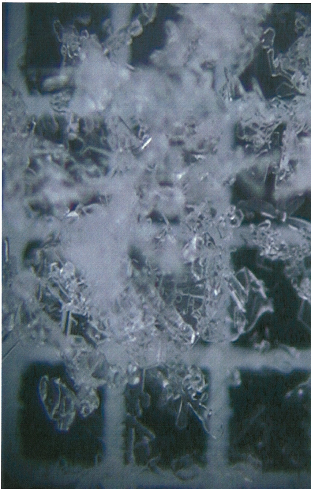
Figure 4.50: One to two mm stellar and broken particle crystals harvested from the east-facing study site on 9 February 2004. The crystals are classified by Colbeck et al. (1990) as type 1d, stellar dendrite, and 2a, broken.
