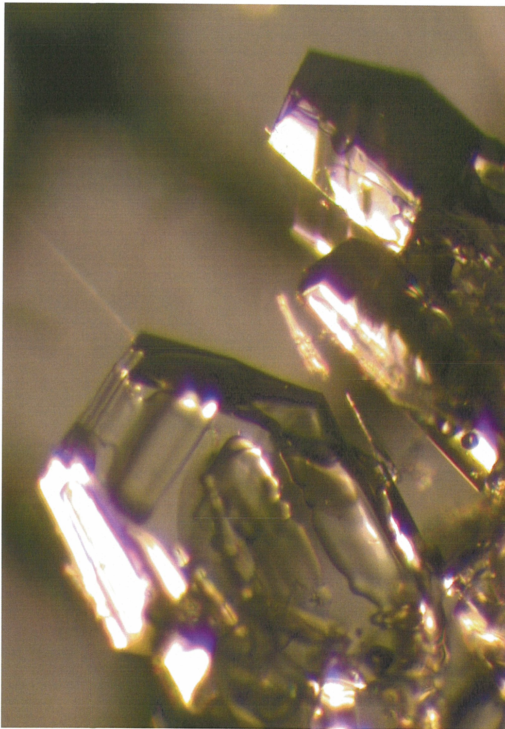
Figure 4.30: A few 1 mm near-surface faceted crystal harvested from the east-facing study site on 13 January 2004. These crystals are classified by Colbeck et al. (1990) as type 4a, solid faceted particles.
