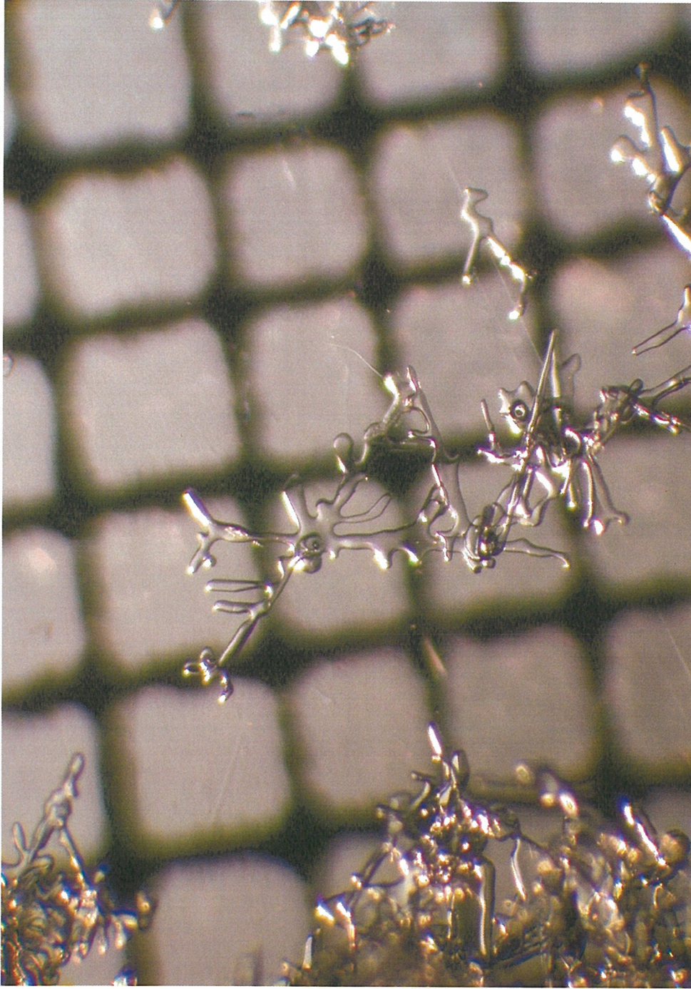
Figure 4.5: A 2 mm broken precipitation particle harvested from the surface of the south-facing study site on 10 January 2004. This crystal is classified by Colbeck et al. (1990) as type 2a/b.
