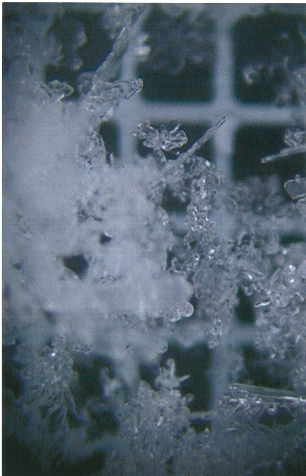
Figure 4.49: One to two mm stellar and broken particle crystals harvested from the north-facing study site on 9 February 2004. The crystals are classified by Colbeck et al. (1990) as type 1d, stellar dendrite, and 2a, broken.
