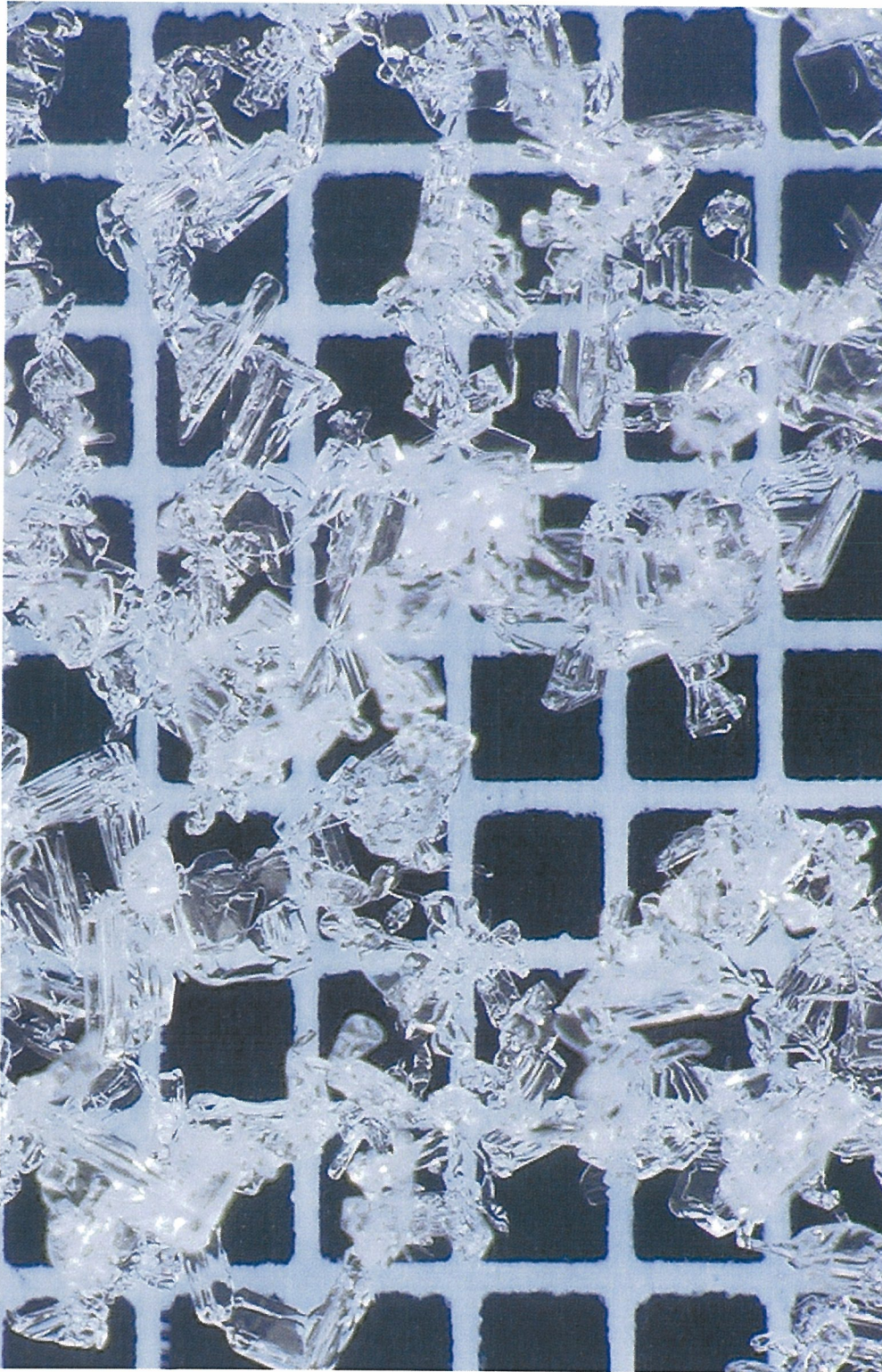
Figure 4.35: A to 1.5 mm near-surface faceted crystal, type 4a, solid faceted particles and 5a, cup shaped crystal, as classified by Colbeck et al. (1990), harvested from the south-facing study site on 22 January 2004.
