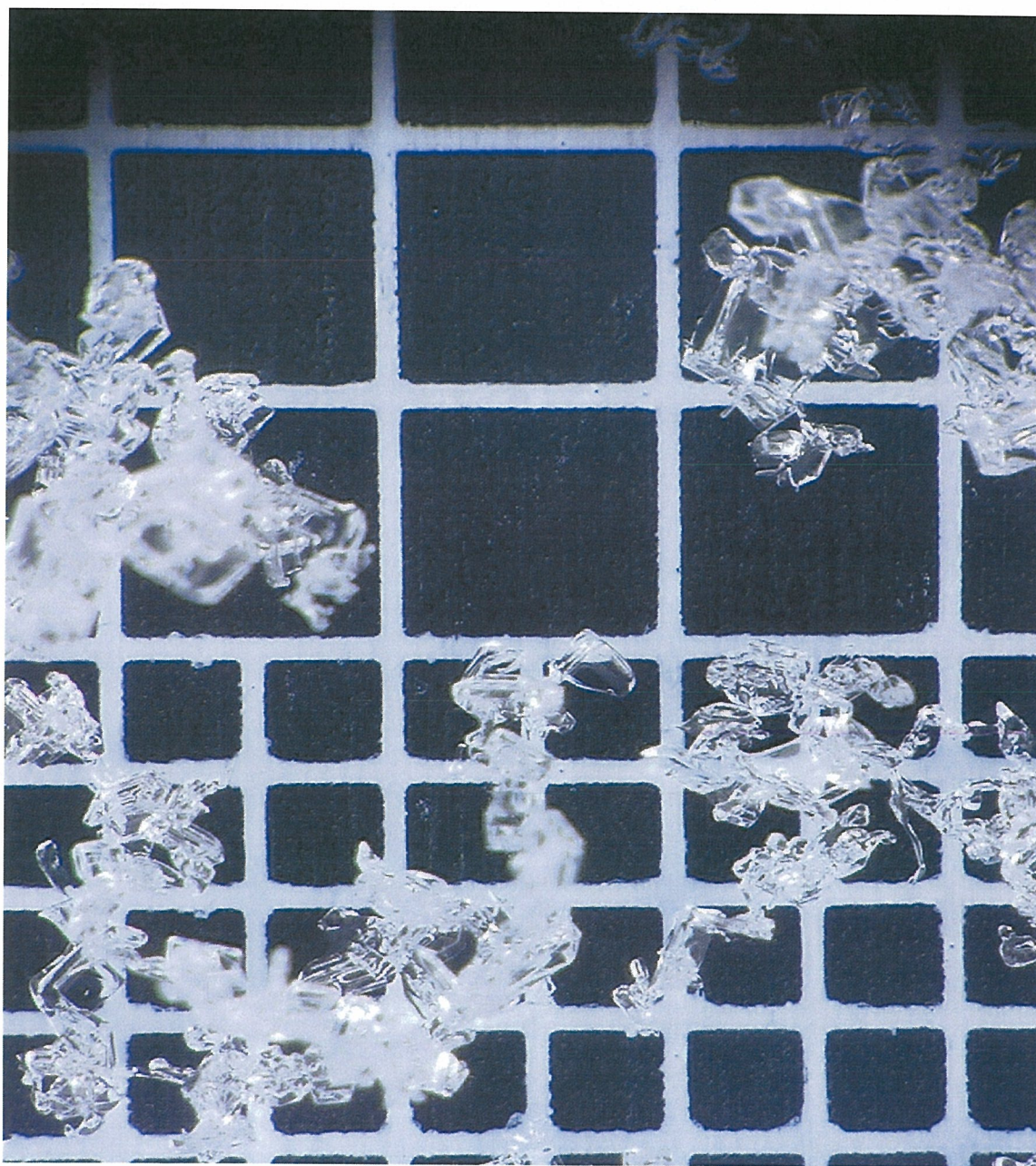
Figure 4.37: A few 1 mm near-surface faceted crystal harvested from the east-facing study site on January 22, 2004. These crystals are classified by Colbeck et al. (1990) as type 4a, solid faceted particles.
