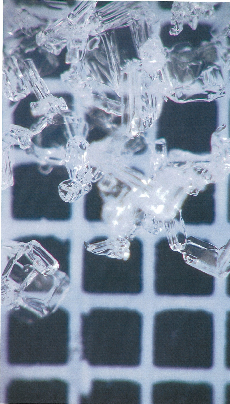
Figure 4.44: One mm near-surface faceted crystals harvested from the east-facing study site on 13 March 2004. These crystals would be classified by Colbeck et al. (1990) as type 4a, solid faceted particles.
