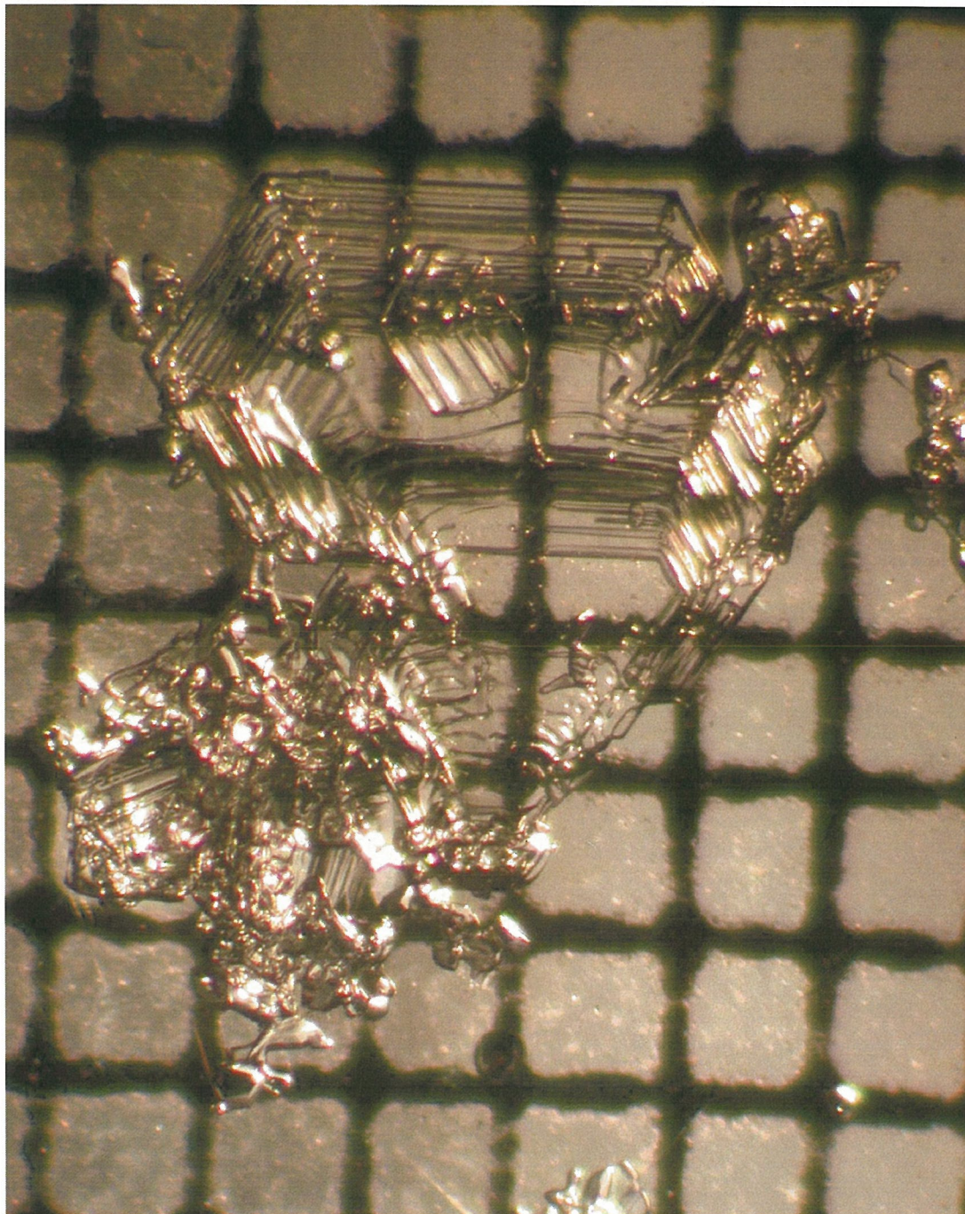
Figure 4.15: A 5.5 mm surface hoar crystal harvested from the south-facing study site on 13 January 2004. This crystal is classified by Colbeck et al. (1990) as type 7a.
