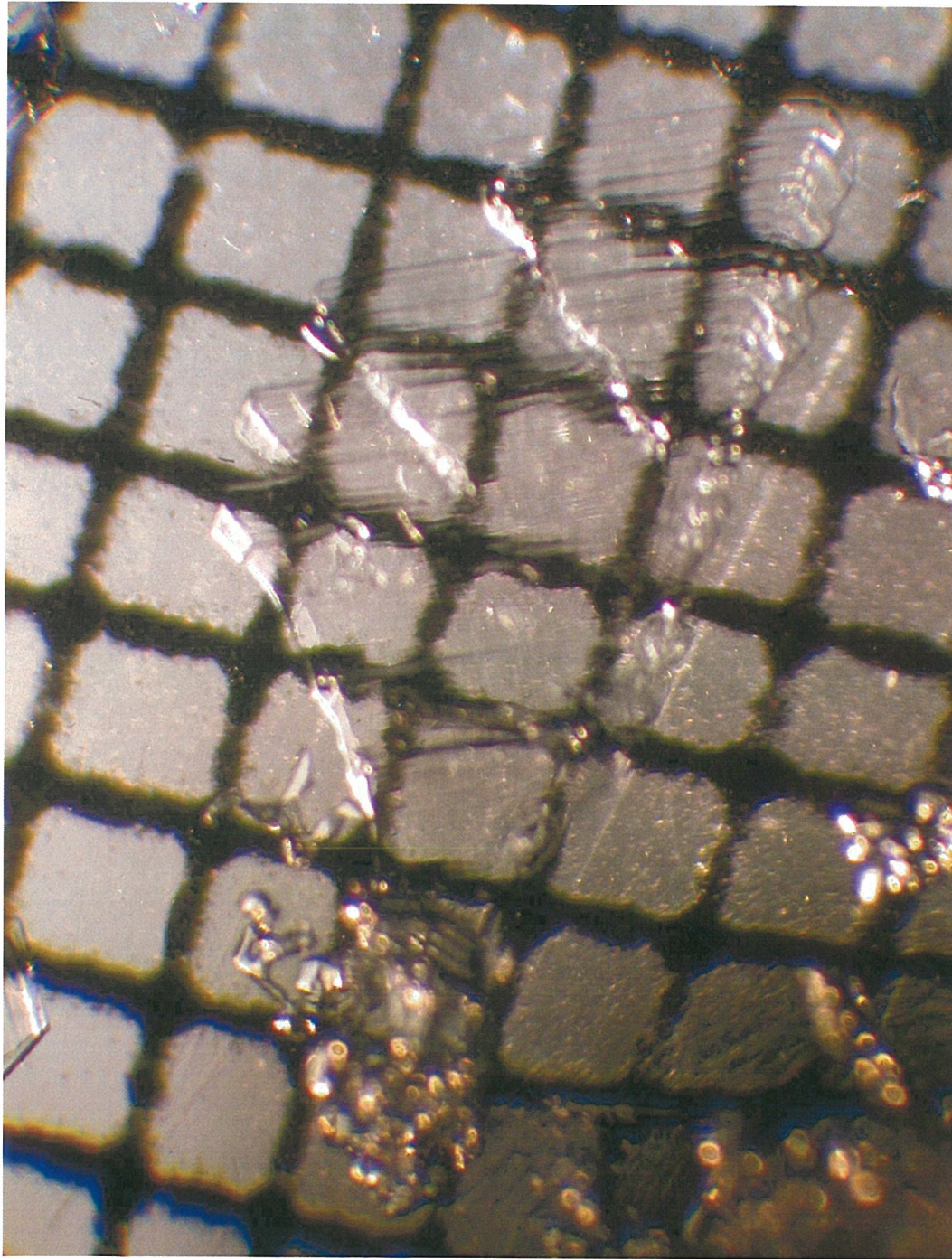
Figure 4.2: A 7mm surface hoar crystal harvested from the north-facing study site on 10 January 2004. This crystal is classified by Colbeck et al. (1990) as type 7a.
