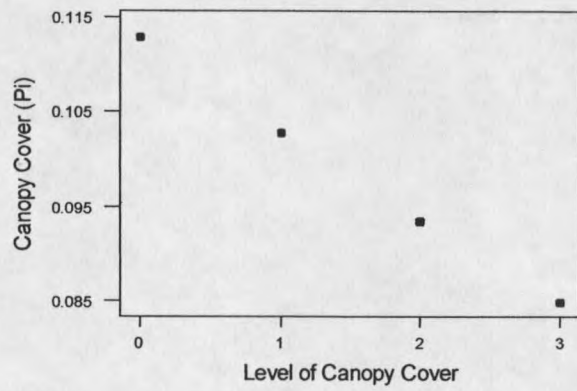
Figure 23. The fitted probability of success for canopy cover.
