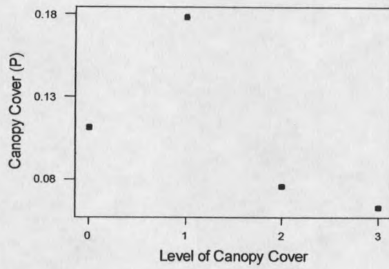
Figure 22. Observed Probability of Success for Canopy Cover.
