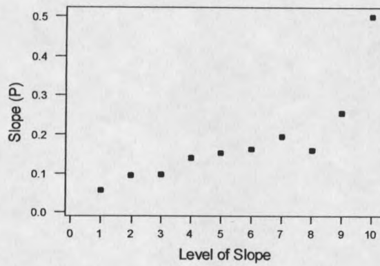
Figure 18. The observed probability of success for slope.
