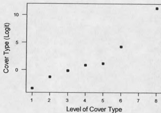
Figure 17. The logit for cover type.
