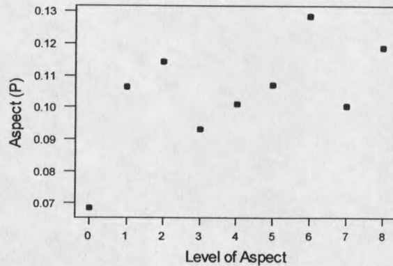
Figure 21. The observed probability of success for aspect.
