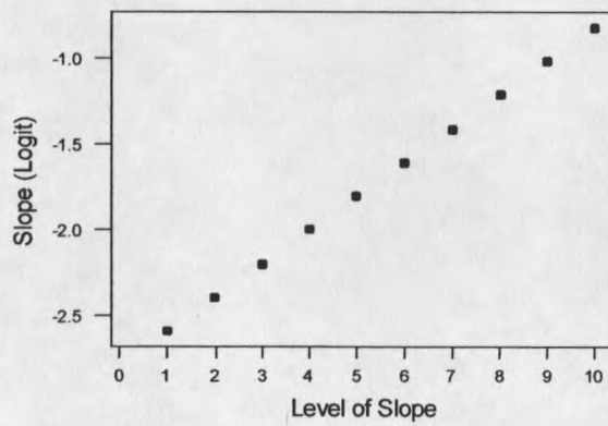
Figure 20. The logit for slope.
