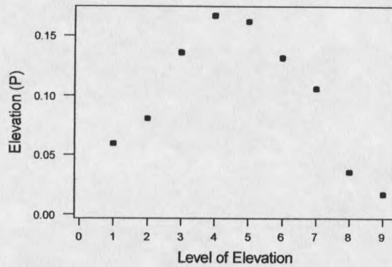
Figure 25. The observed probability of success for elevation.
