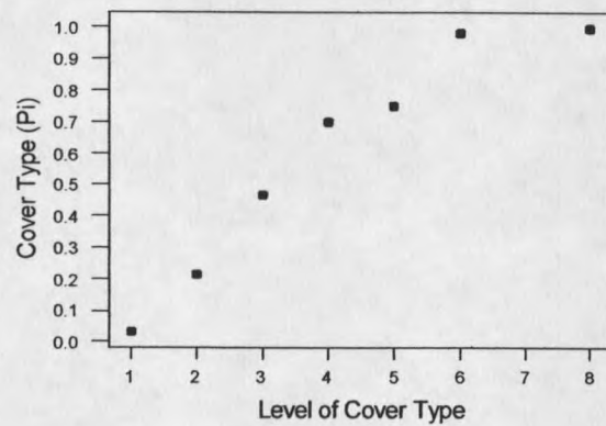
Figure 16. The fitted probability of success for cover type
