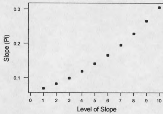
Figure 19. The fitted probability of success for slope.
