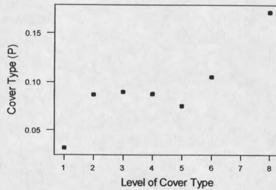
Figure 15. The observed probability of success for cover type.
