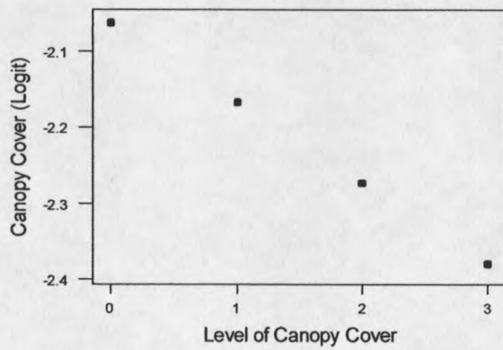
Figure 24. The logit for canopy cover.
