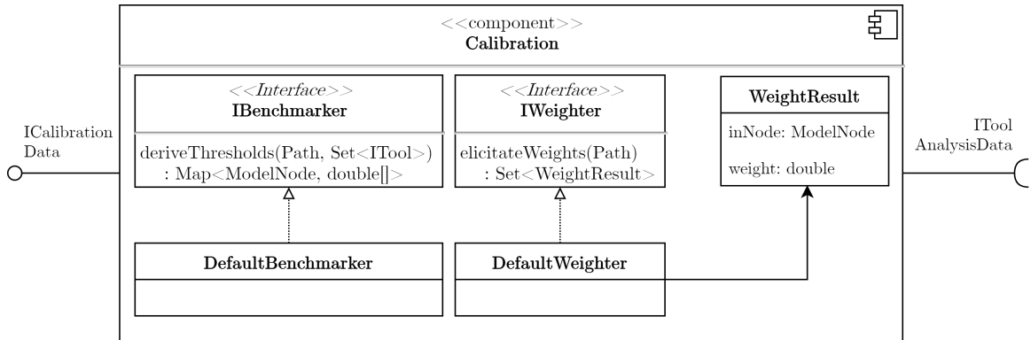
Figure 4.7: PIQUE Calibration Component
