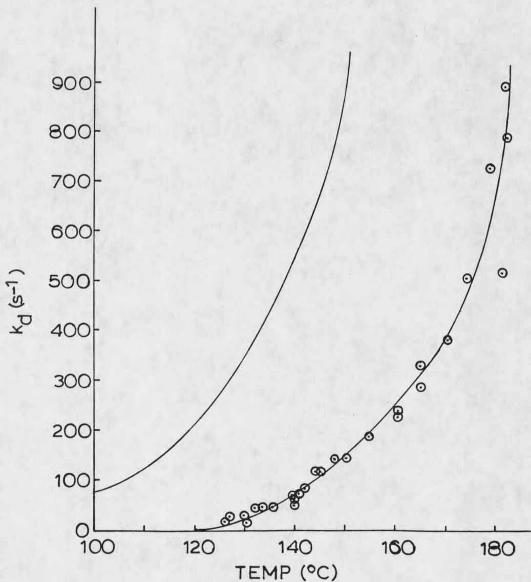
Figure 35. Autodetachment rate coefficient, k_d , for azulene as a function of temperature, determined with the PDM-ECD (circles). k_d values were obtained by combining the data from Figures 32 and 34. Also shown (line) are the values determined by Grimsrud, Chowdhury, and Kebarle (78).
