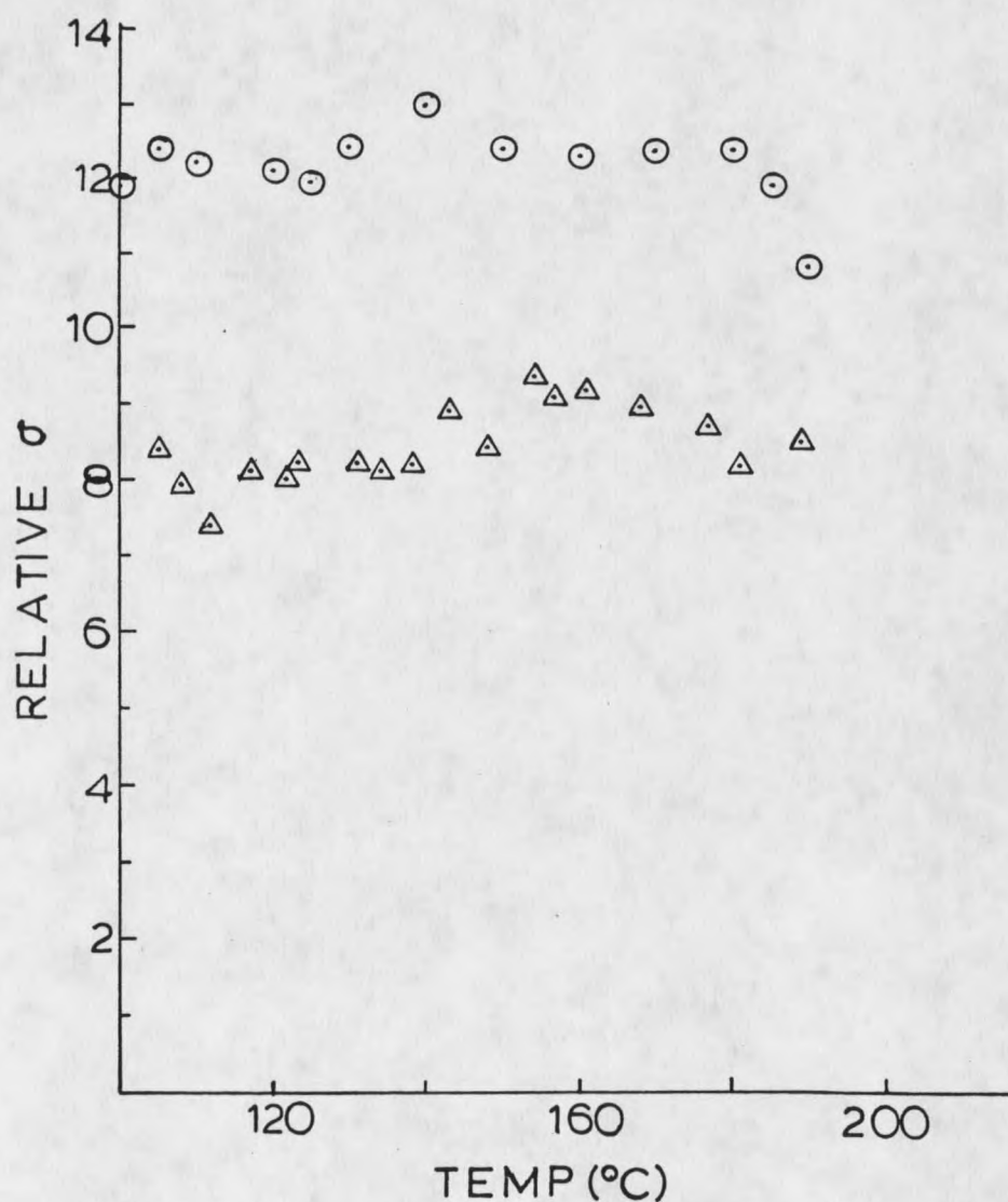
Figure 33. The relative PD cross-sections for I - and p-fluoronitrobenzene anion as a function of temperature. For I - , measurements for σ were obtained at 360 and 370 nm and averaged. For p-fluoronitrobenzene, σ was obtained at 525 nm, the long wavelength peak in its spectrum (see Figure 19F).
