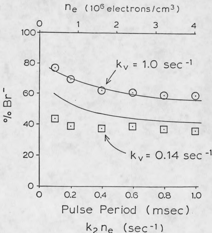
Figure 40. Relative abundance of \text{Br}^- produced by electron capture of \text{CBrCl}_3 at 50^\circ\text{C} observed by the PDM-ECD. Detector gas flow rates of 115\text{ cm}^3\text{ min}^{-1} (circles) and 16\text{ cm}^3\text{ min}^{-1} (squares) have been used and each data set is assigned a rate coefficient for ventilation, k_v = \text{flow rate} / \text{ECD volume} . For each ECD pulse period used, the average electron density, n_e , is shown on the upper x-axis. The pseudo-first-order rate constant, k_2 n_e , for EC by \text{CCl}_3 is also indicated by the lower x-axis where k_{19} = 2.4 \times 10^{-7}\text{ cm}^3\text{ s}^{-1} (from reference 87) has been used. The two curves shown are predictions of \%\text{Br}^- based on the coefficients for k_{18} , k_{19} , and k_{21} given in reference 87 and assuming the branching ratios for Reactions 18a/b and 21a/b are 4 to 1 and 0 to 1, respectively.
