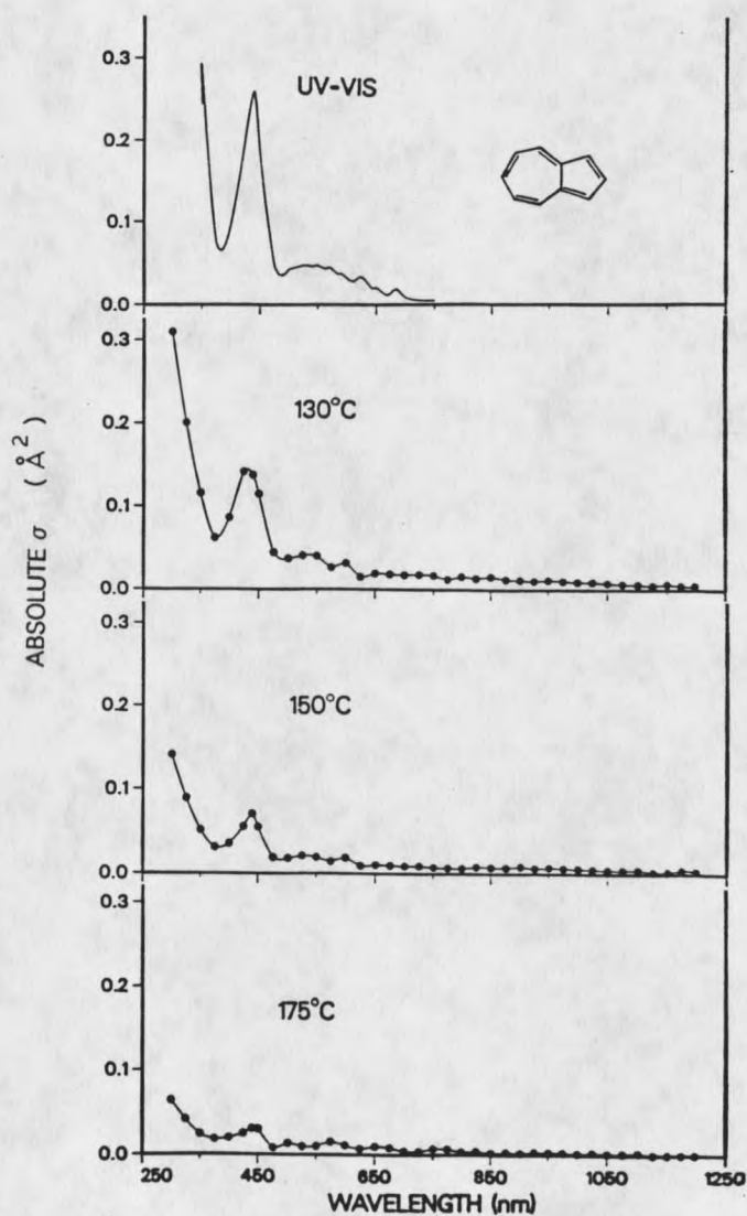
Figure 31. PD spectrum of azulene at three different temperatures. The apparent decrease in the cross-section at higher temperatures is due to autodetachment of the electron from the anion. Also shown is the UV-Vis absorption spectrum for azulene obtained in a frozen organic glass by Shida (81).
