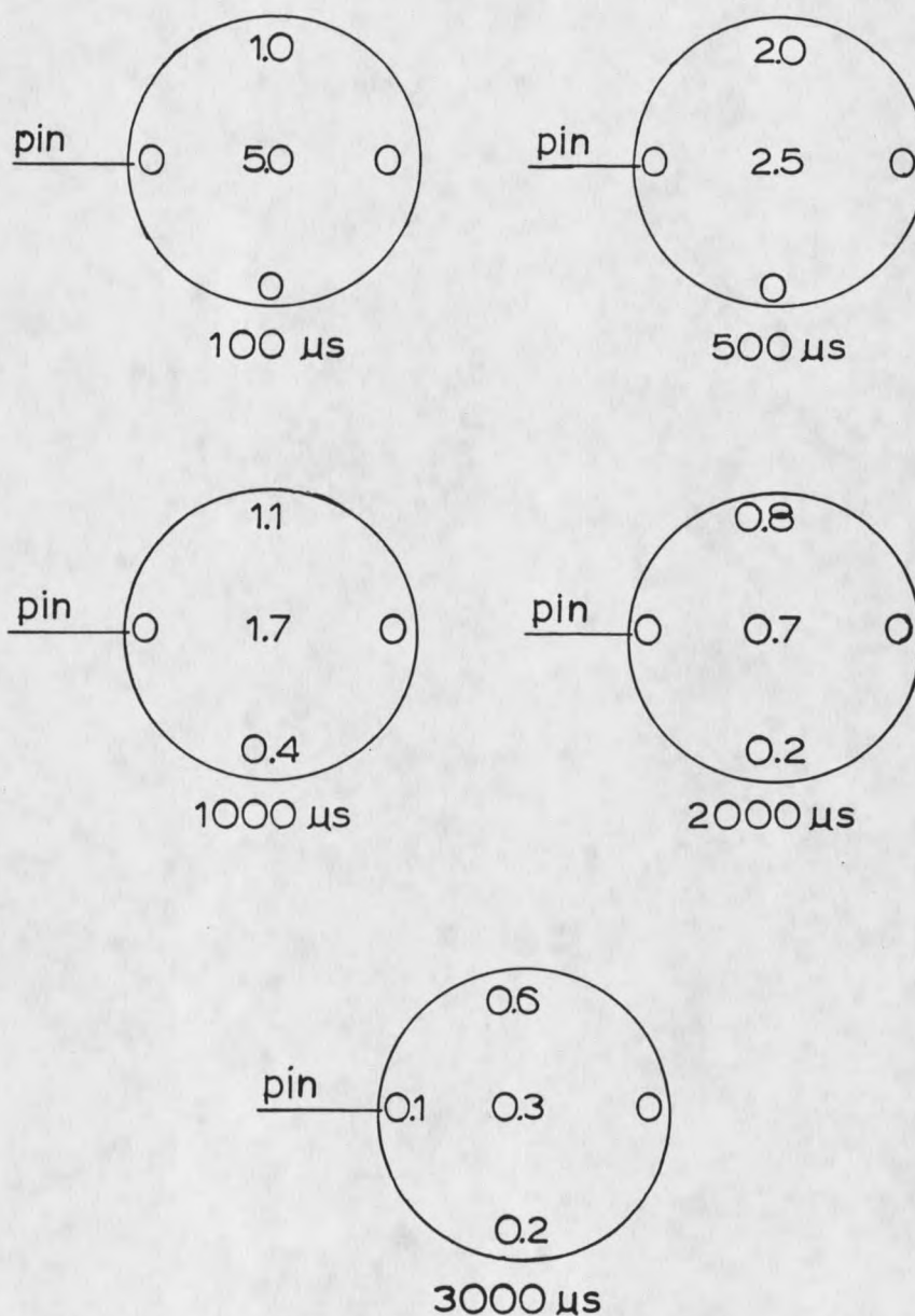
Figure 42. Relative PD responses to iodide with the light focused into the region of the ECD represented by the circles. The full, chopped emission of a Hg/Xe lamp was used. The numbers reflect the relative abundance of negative ions at the various locations in the ECD at the indicated pulse periods, and demonstrate that at fast pulsing (100 \mu\text{s} ), the ions are concentrated in the center of the cell, but at slow pulsing (3000 \mu\text{s} ), the ions are more dispersed.
