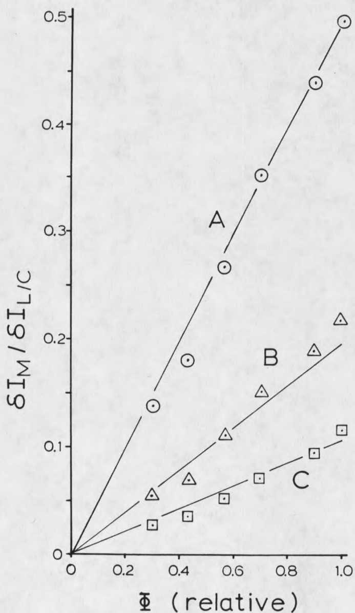
Figure 8. Ratio of \delta I_M / \delta I_{L/C} responses to (A) \text{CH}_3\text{I} , (B) \text{CF}_2\text{Br}_2 , and (C) \text{CHCl}_3 observed with use of various relative intensities of light emitted by the Xe arc lamp, without use of a monochromator or filters. Solid lines are predictions of relative response ratios based on the overlap integrals of the PD cross-sections and the Xe lamp emission spectrum shown in Figure 1.
