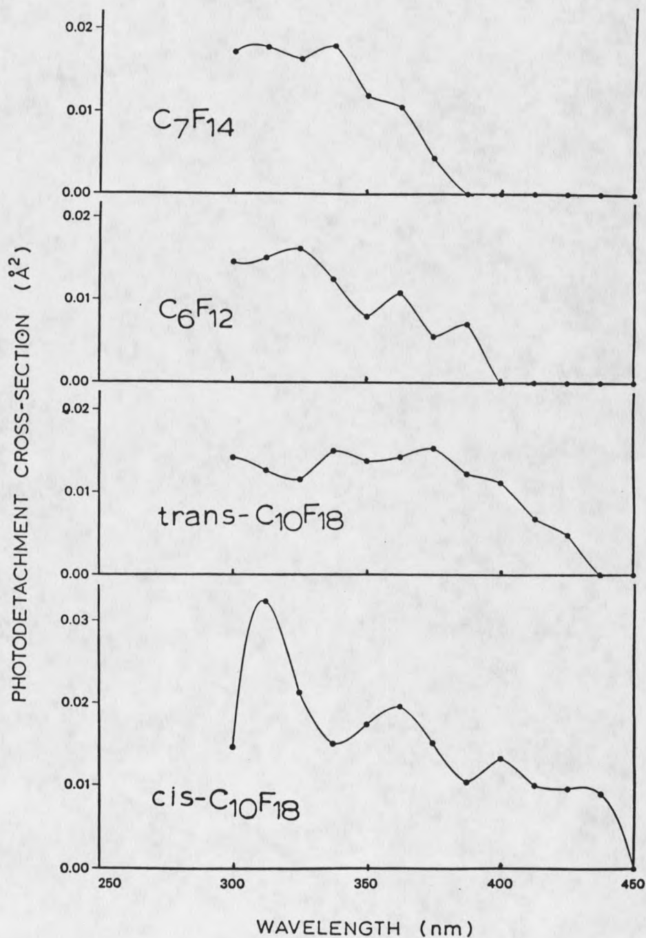
Figure 30. PD spectra of four perfluorocarbons. The \delta I_M responses were quite small resulting in an uncertainty for the PD cross-sections of about \pm 50\% .
