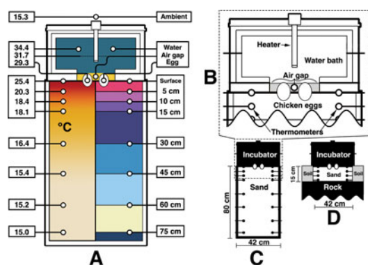
FIGURE 2. Diagram of the surrogate incubator and sediment container. A, A cross section of the experiment with temperatures ( ^{\circ}\text{C} ) corresponding to those recorded at 72 hours (left). The right side of A shows the location of temperature-probe groups. Divisions correspond to those used in Figs. 3–5. B, A simplified pullout of the surrogate incubator, eggs, and sediment interface. C, Dimensions of the sediment container. D, The surrogate over the sand-filled chamber in the outside setup.
