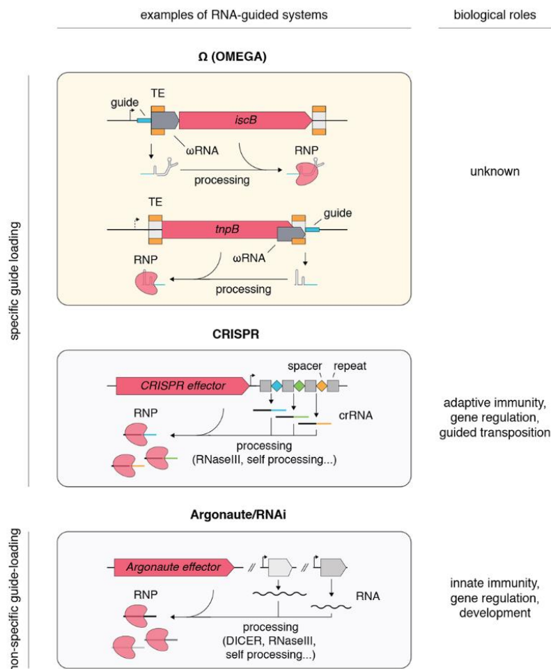
Fig. 6. Naturally occurring RNA-guided DNA-targeting systems. Comparison of Ω (OMEGA) systems with other known RNA-guided systems. In contrast to CRISPR systems, which capture spacer sequences and store them in the locus within the CRISPR array, Ω systems may transpose their loci (or trans -acting loci) into target sequences, converting targets into \omega RNA guides.
