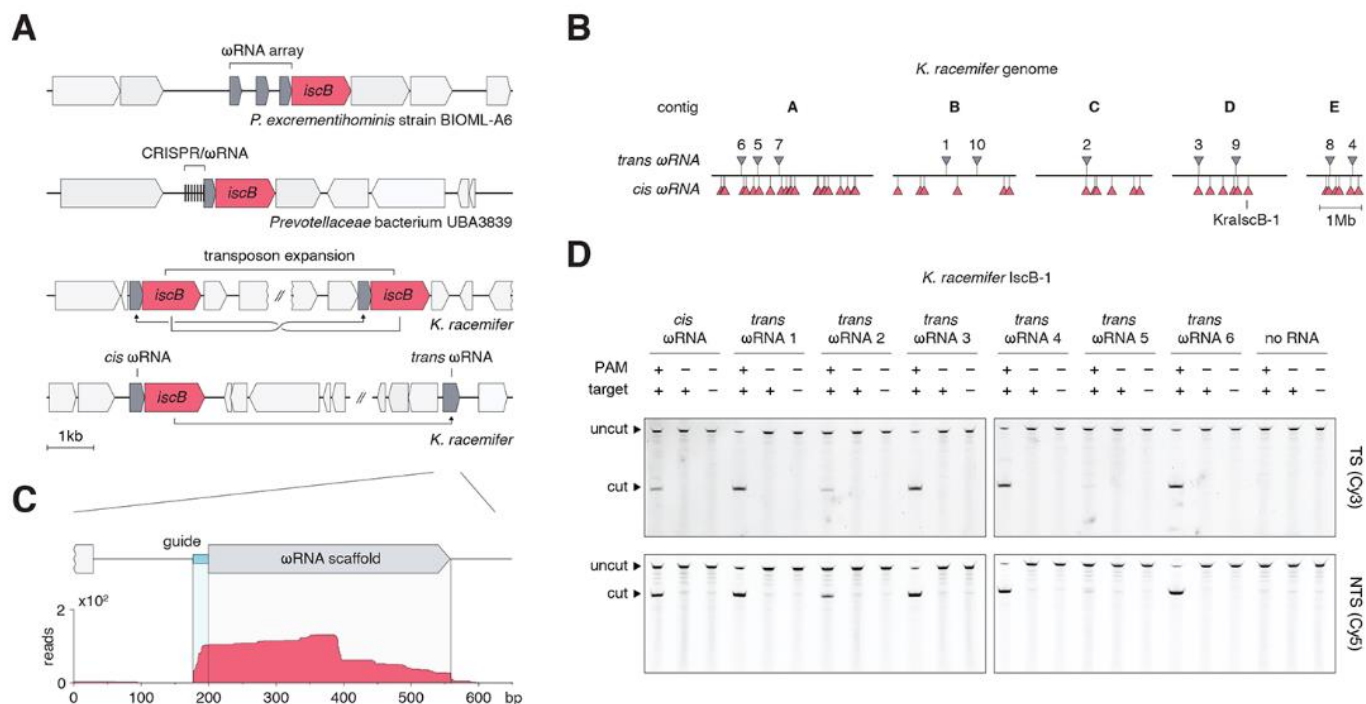
Fig. 3. Guide-encoding mechanisms of IscB. (A) Example loci for each major mechanism of encoding multiple guides: entire ωRNAs arrays associate with IscB, ωRNAs duplicate or insert into CRISPRs, transposon expansion results in multiple nearly identical loci that each express different guides, and standalone trans -acting ωRNAs form independently of adjacent IscBs. (B) K. racemifer encodes 48 IscB loci with cis ωRNAs and 10 standalone trans -acting ωRNAs. (C) Small RNA-seq of a standalone ωRNA locus in K. racemifer . (D) KraliscB-1, in complex with cis or trans ωRNAs with the same guide sequence, mediate cleavage of dsDNA in a TAM- and target-dependent manner. Reactions were performed in IVTT using 5' strand-specific labeled linear targets. TS: Target strand; NTS: non-target strand. Contig accession and position information for all displayed loci are listed in table S6.
