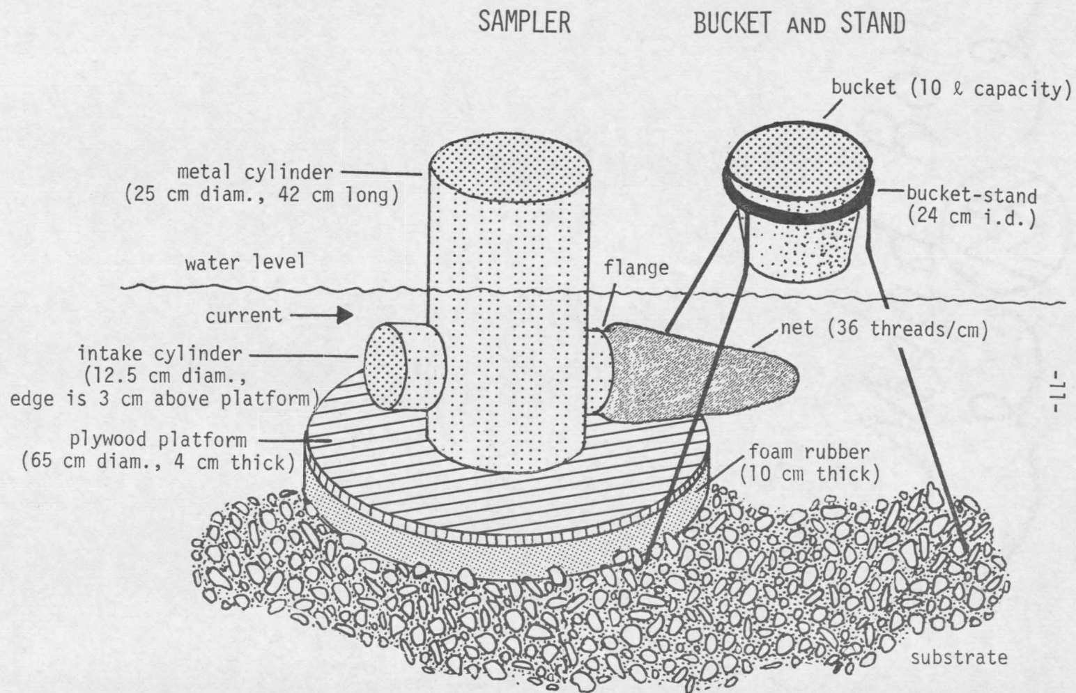
Figure 2. Sampler designed for this study.
