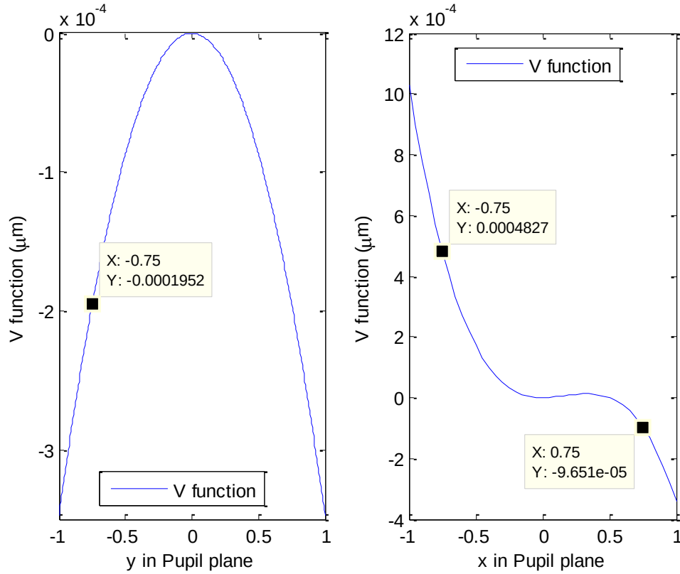
Figure 92: OPD fans from \mathcal{V} -function for 5° incidence mirror, \delta = 2 \mu\text{m} , u_2 = 0.5 \text{ mm} , v_2 = 0 \text{ mm} , and r_1 = \infty .
