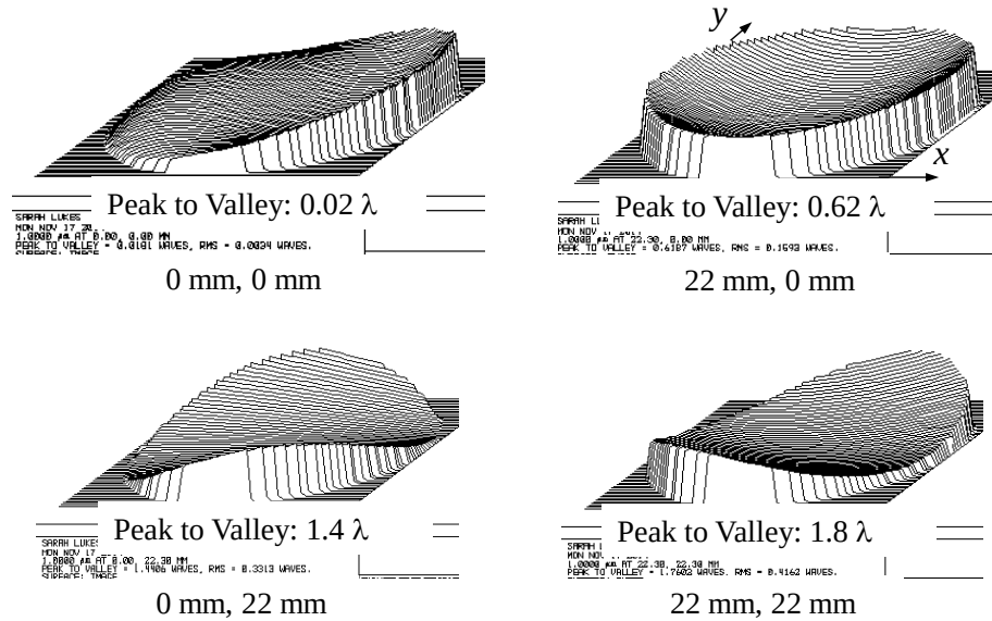
Figure 57: Zemax wavefront surfaces without tilt for four different image locations (u_2, v_2) to verify approximately 1 wave of astigmatism due to 2 nd -order aberration terms. A 5.000 mm x 5.019 mm elliptical-boundary mirror represented as an even polynomial ( Z = .00226X^2 + .00227Y^2 ) is analyzed here with \lambda = 1 \mu\text{m} . Variable r_1 is infinity and r_2 is 110 mm.
