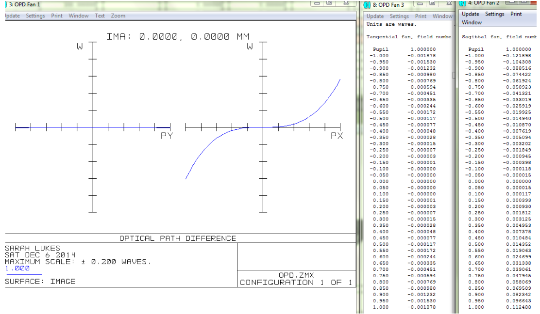
Figure 102: OPD fans from Zemax for 45^\circ incidence mirror, \delta = 20 \mu\text{m} , u_2 = 0 \text{ mm} , v_2 = 0 \text{ mm} , and r_1 = 200 \text{ mm} .
