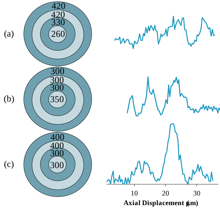
Figure 81: Axial point spread functions ( \lambda = 488 nm) of the confocal microscope for three different voltage profiles. Defocus remained constant for the three measurements. All horizontal (axial displacement) and vertical (intensity) axes are the same scale. (a) The point spread function has several large side lobes with the center electrode's voltage being 160 V less than the outer two electrodes. (b) The side lobes shift to the left-hand side of the main lobe with 350 V on the centermost electrode and 300 V on the outer electrodes. (c) With 300 V on the inner two and 400 V on the outer two electrodes point spread function gains intensity on the central lobe and it narrows to approximately 5 \mu\text{m} FWHM.
