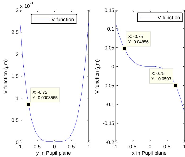
Figure 103: OPD fans from v -function for 45^\circ incidence mirror, \delta = 20 \mu\text{m} , u_2 = 0 \text{ mm} , v_2 = 0 \text{ mm} , and r_1 = 200 \text{ mm} .
