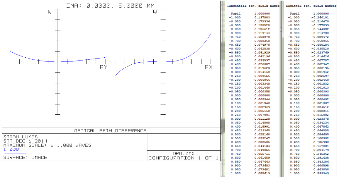
Figure 100: OPD fans from Zemax for 45^\circ incidence mirror, \delta = 20 \mu\text{m} , u_2 = 0 \text{ mm} , v_2 = 5 \text{ mm} , and r_1 = \infty .
