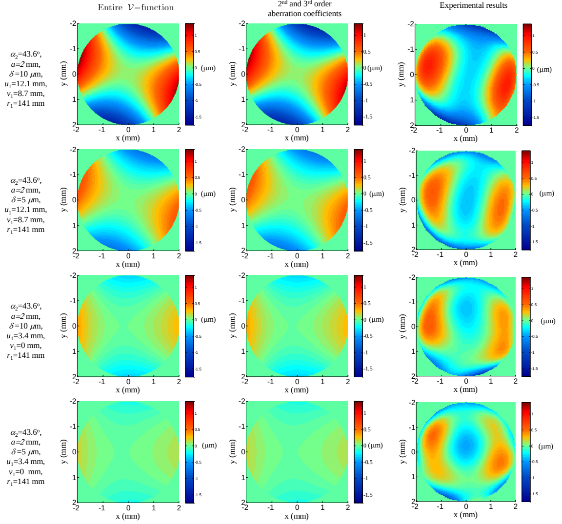
Figure 65: Wavefronts generated from the entire \mathcal{V} -function, 2 nd and 3 rd order aberration terms, and Zernike terms from the WFS for r_1 = 141 mm.
