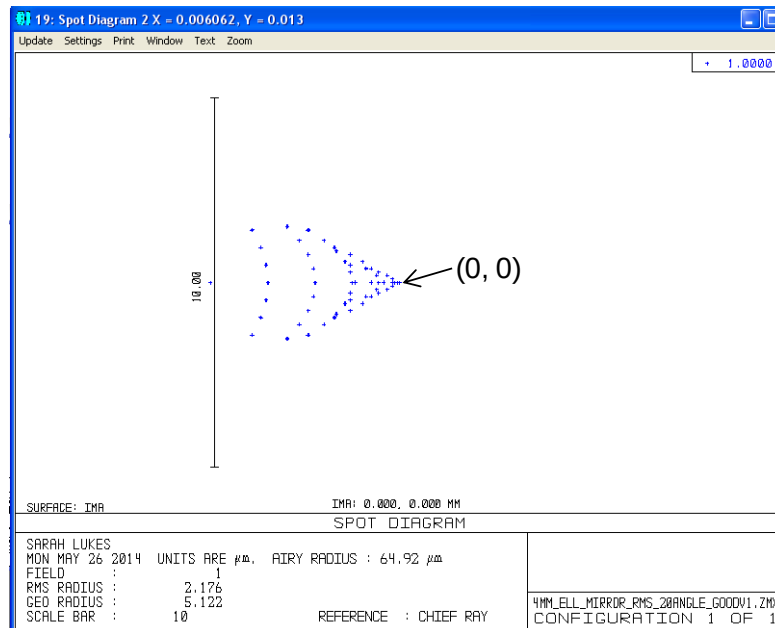
Figure 87: Zemax spot diagram of a 20^\circ incidence angle 4 mm x 4.26 mm elliptical mirror with 5\text{ }\mu\text{m} deflection and an object at infinity with no field.
