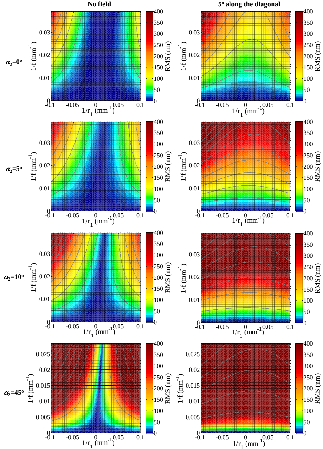
Figure 40: Wavefront RMS for \alpha_2 = 0^\circ, 5^\circ, 10^\circ , and 45^\circ shown in rows. The left column shows no-field imaging with u_2 = v_2 = 0 and the right column has 5^\circ of field along the diagonal in the image plane. All graphs show the mirror with a deflection ranging from 0 \mu\text{m} to 40 \mu\text{m} .
