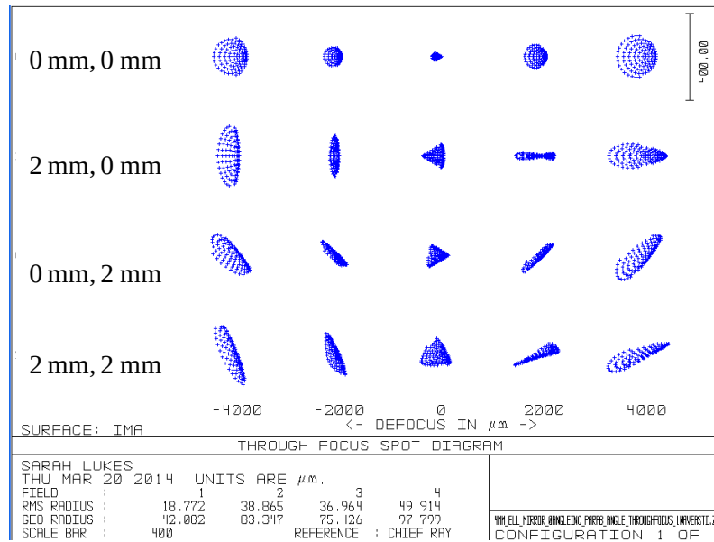
Figure 52: Zemax through-focus spot diagrams for four different image locations (u_2, v_2) to verify approximately 1 wave of astigmatism due to 2 nd -order aberration terms. A 5.000 mm x 7.071 mm elliptical-boundary mirror represented as an even polynomial ( Z = .0016X^2 + .0032Y^2 ) is analyzed here with \lambda = 1 \mu\text{m} . Variable r_1 is infinity and r_2 is 110 mm.
