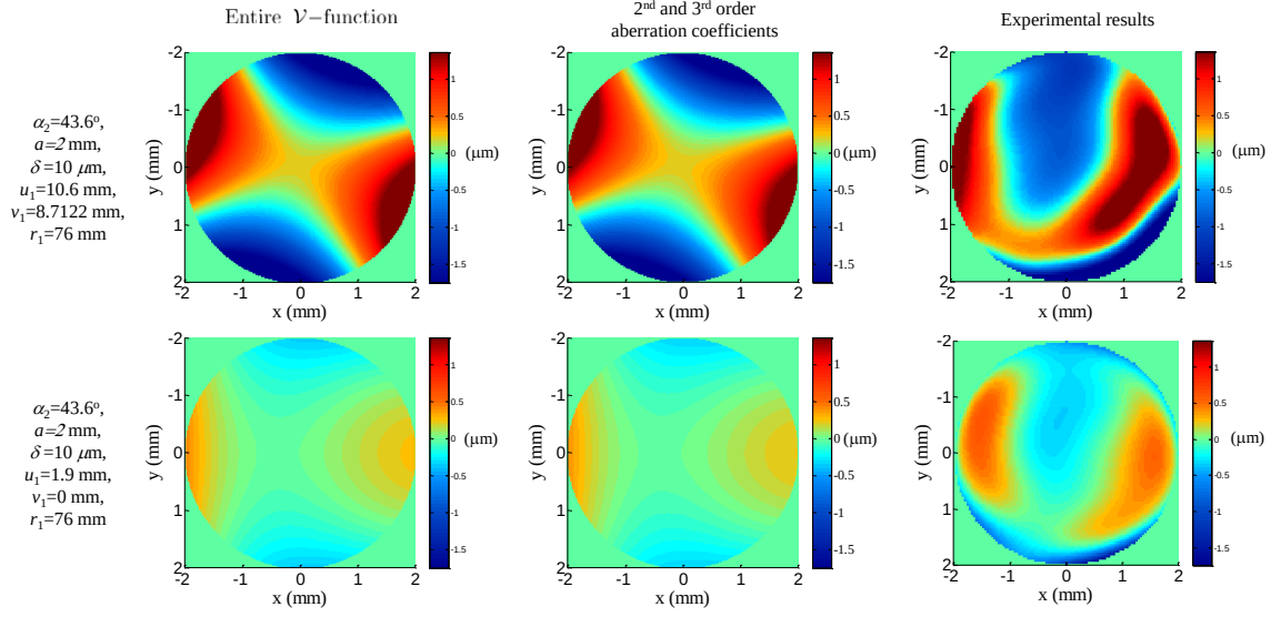
Figure 66: Wavefronts generated from the entire \mathcal{V} -function, 2 nd - and 3 rd -order aberration terms, and Zernike terms from the WFS for r_1 = 76\text{ mm} .
