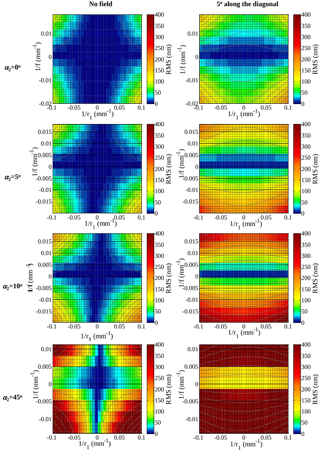
Figure 45: Wavefront RMS for \alpha_2 = 0^\circ, 5^\circ, 10^\circ , and 45^\circ shown in rows. The left column shows no-field imaging with u_2 = v_2 = 0 and the right column has 5^\circ of field along the diagonal in the image plane. All graphs show the mirror with a deflection ranging from -20 \mu\text{m} to 20 \mu\text{m} .
