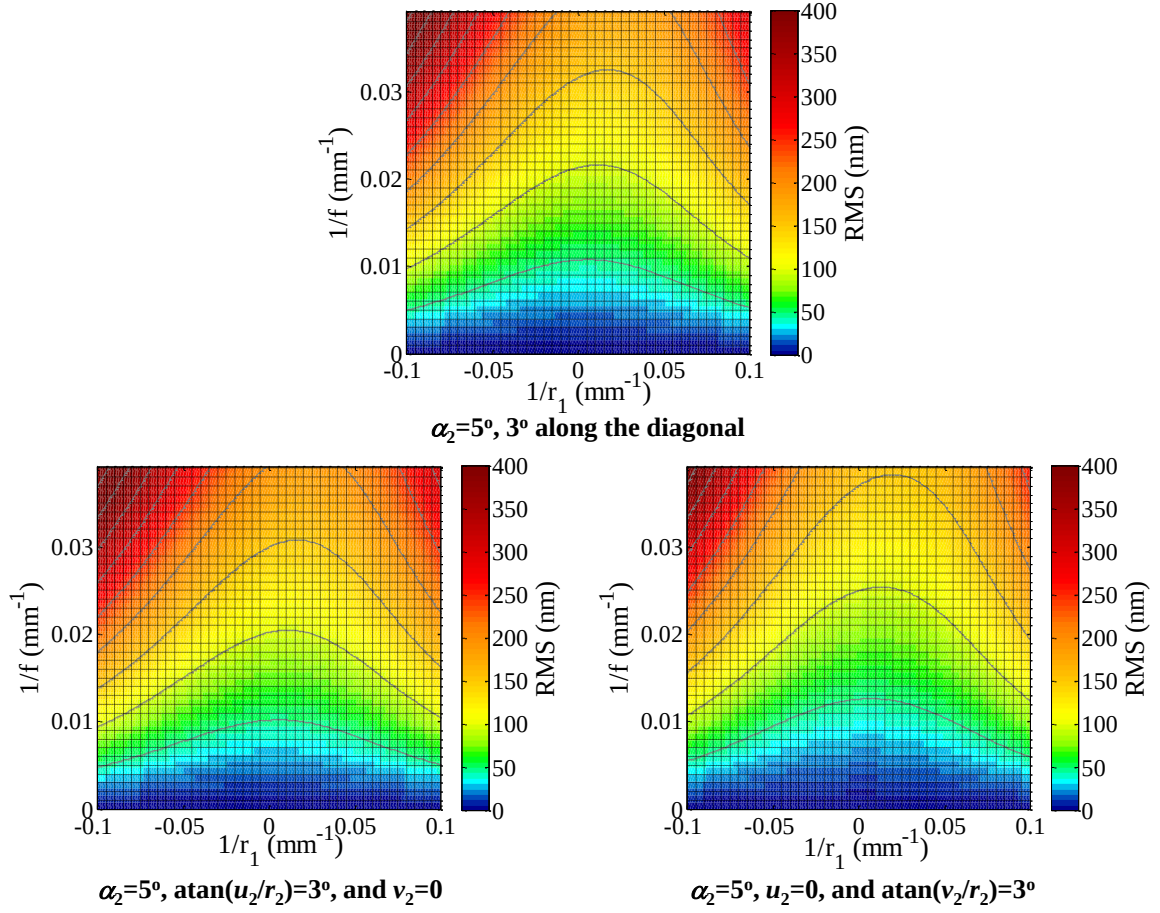
Figure 41: Wavefront RMS for \delta = 0 \text{ }\mu\text{m} to 40 \text{ }\mu\text{m} for 5^\circ incidence angle. The top plot shows a field of 3^\circ along the diagonal. The bottom two plots show the aberrations with 3^\circ field in the individual field coordinates.
