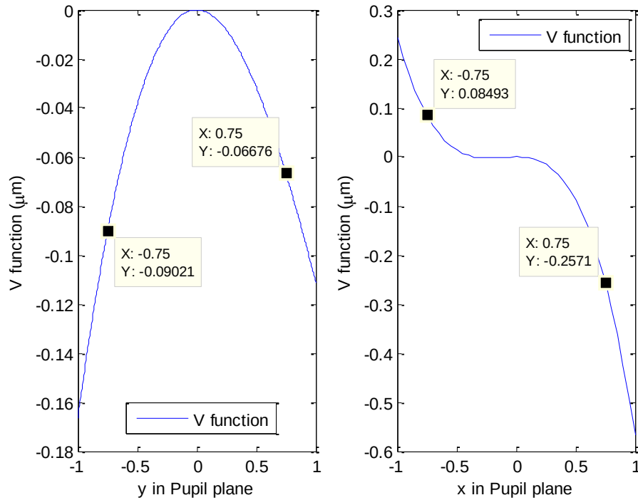
Figure 101: OPD fans from v -function for 45^\circ incidence mirror, \delta = 20 \mu\text{m} , u_2 = 0 \text{ mm} , v_2 = 5 \text{ mm} , and r_1 = \infty .
