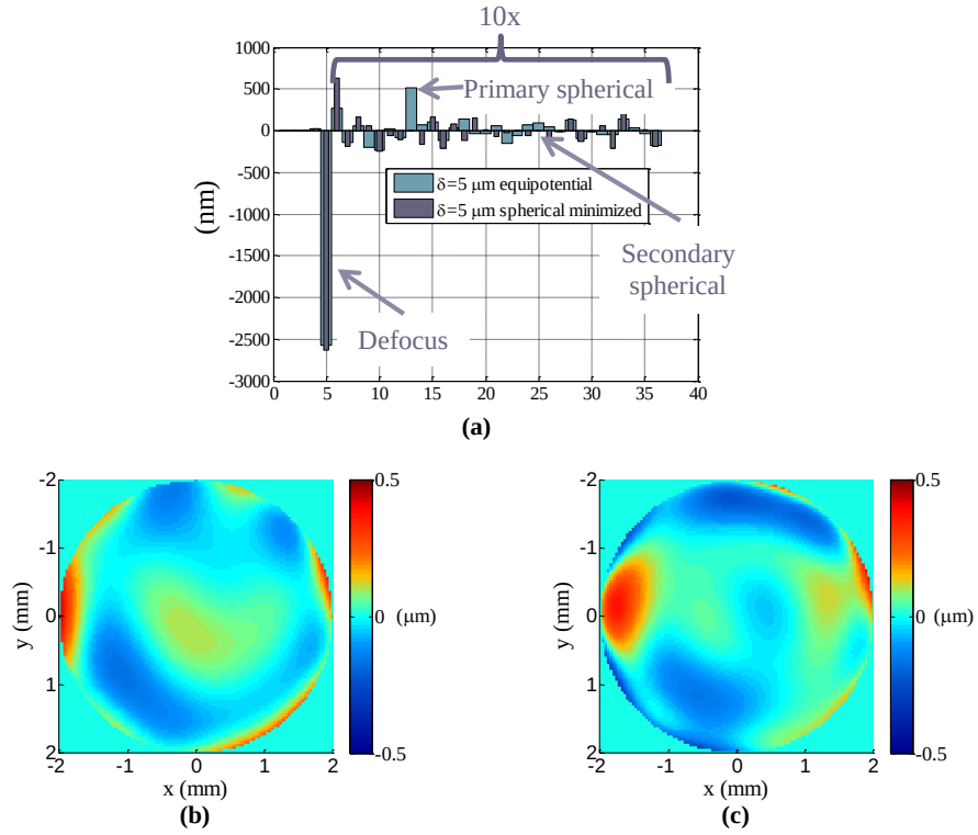
Figure 23: Comparison of Zernike terms and wavefronts for a process-1 4 mm 5^\circ mirror with equipotential (200 V) and varied voltages to minimize spherical aberration terms ( E_1 = 200 V, E_2 = 185 V, E_3 = 205 V, and E_4 = 225 V). For both voltage profiles, the center of the mirror is displaced 5 \mu\text{m} . (a) Zernike terms as generated from a phase-shift interferometer with normal incident light rays on the mirror. Terms above Z5 are magnified by 10x. Primary and secondary spherical aberration decrease for the varied voltage case, where the varied voltages reduce the primary spherical aberration by approximately 500 nm. (b) Equipotential wavefront. (c) The wavefront with spherical aberration minimized.
