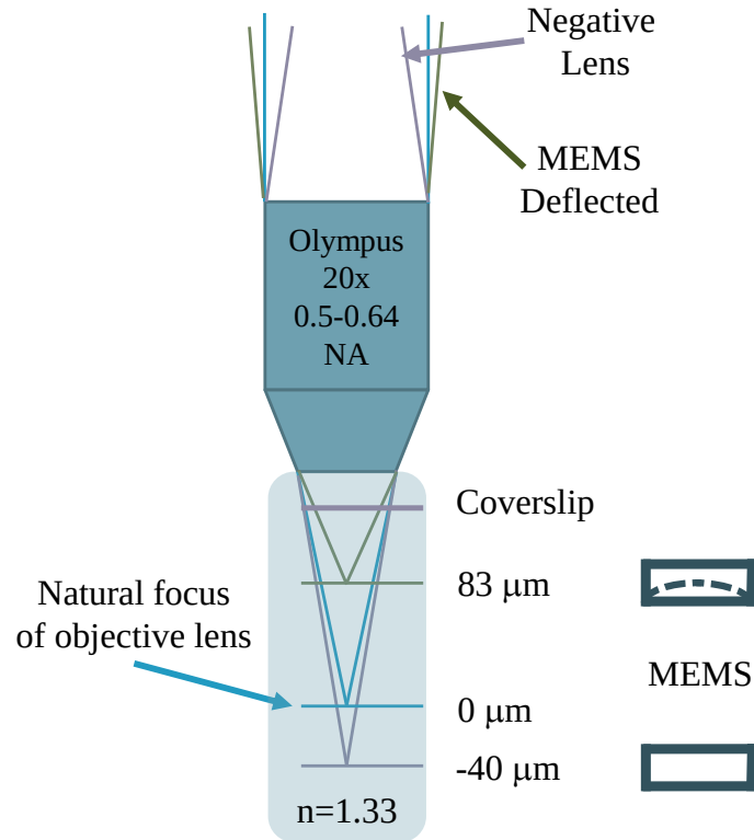
Figure 76: The natural focal plane of the Olympus water objective is defined as 0 \mu\text{m} . With the MEMS module (including the negative lens) inserted with an un-deflected MEMS mirror the focus lies at -40 \mu\text{m} . An increase in voltage on the MEMS mirror increases its displacement until the focal plane behind the objective lens lies at 83 \mu\text{m} .
