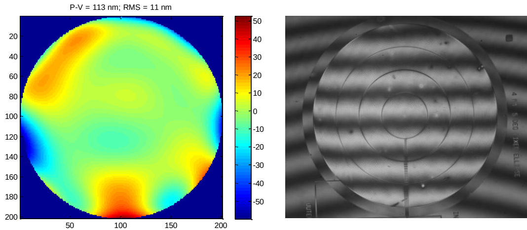
Figure 18: (left) Surface profile of a process-1 4 mm 5^\circ mirror scaled to a circular perimeter as measured by phaseshift interferometry. (right) A photograph of the mirror tilted in the interferometer for a flat (no voltage applied) process-1 4 mm 5^\circ mirror. The MEMS mirror exhibits excellent optical quality with 113 nm peak-to-valley and 11 nm RMS.
