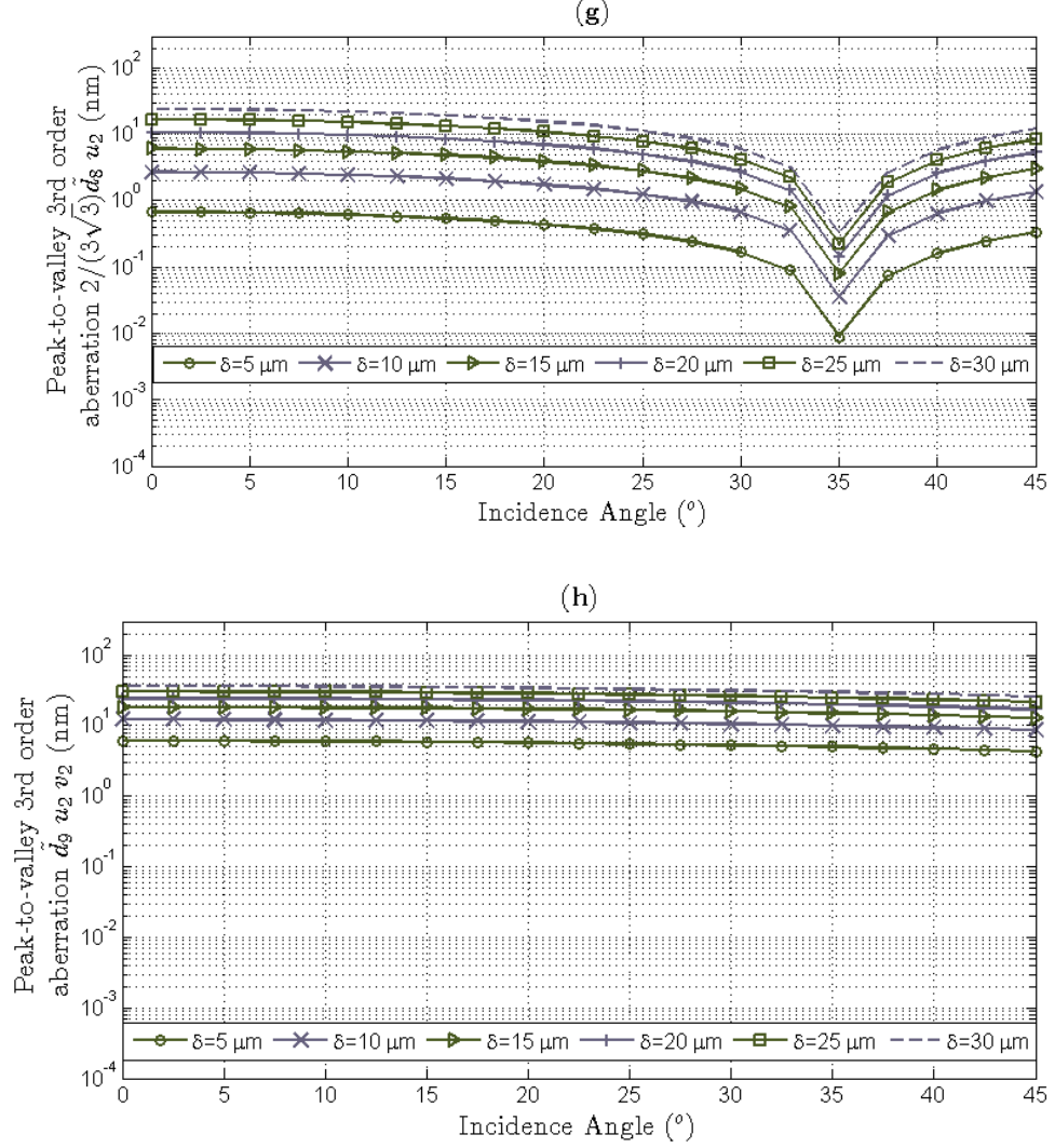
Figure 34: The 3 rd -order, peak-to-valley aberrations for various deflections and incidence angles of an a = 2 \text{ mm} mirror and r_1 = \infty . Although \text{atan}(u_2/r_2) = \text{atan}(v_2/r_2) = 1^\circ for all plots, the vertical axis labels show dependence of the aberration terms on field angles for ease of changing field angles. Plots a, b, c, d, e, f, g, h, i, j, and k are for coefficients \tilde{d}_1, \tilde{d}_2, \tilde{d}_3, \tilde{d}_4, \tilde{d}_5, \tilde{d}_6, \tilde{d}_8, \tilde{d}_9, \tilde{d}_{11}, \tilde{d}_{12} , and \tilde{d}_{14} .
