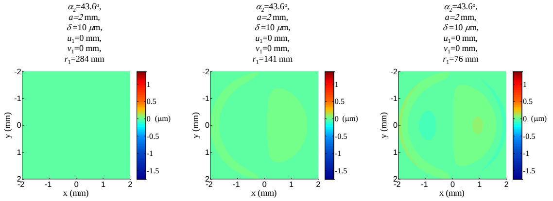
Figure 67: Wavefronts generated from the entire \mathcal{V} -function to demonstrate theoretical aberrations for no-field imaging for r_1 = 284\text{ mm} , r_1 = 141\text{ mm} , and r_1 = 76\text{ mm} .
