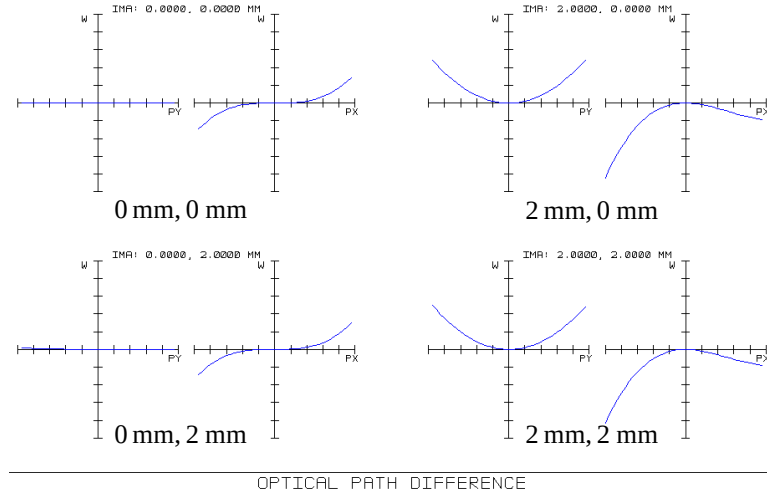
Figure 50: Zemax optical path difference fans for four different image locations ( u_2, v_2 ) to verify approximately 1 wave of astigmatism due to 2 nd -order aberration terms. A 5.000 mm x 7.071 mm elliptical-boundary mirror represented as an even polynomial ( Z = .0016X^2 + .0032Y^2 ) is analyzed here with \lambda = 1\mu\text{m} . Variable r_1 is infinity and r_2 is 110 mm.
