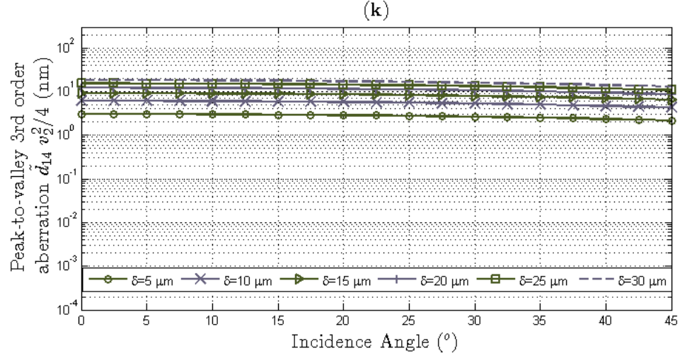
Figure 34: The 3 rd -order, peak-to-valley aberrations for various deflections and incidence angles of an a = 2 mm mirror and r_1 = \infty . Although \text{atan}(u_2/r_2) = \text{atan}(v_2/r_2) = 1^\circ for all plots, the vertical axis labels show dependence of the aberration terms on field angles for ease of changing field angles. Plots a, b, c, d, e, f, g, h, i, j, and k are for coefficients \tilde{d}_1 , \tilde{d}_2 , \tilde{d}_3 , \tilde{d}_4 , \tilde{d}_5 , \tilde{d}_6 , \tilde{d}_8 , \tilde{d}_9 , \tilde{d}_{11} , \tilde{d}_{12} , and \tilde{d}_{14} .
