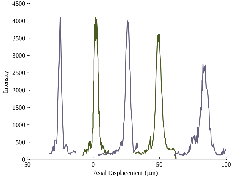
Figure 80: Altering voltages on the four electrodes improves the axial PSFs ( \lambda = 633 nm) while maintaining similar focal planes as in Figure 79.
