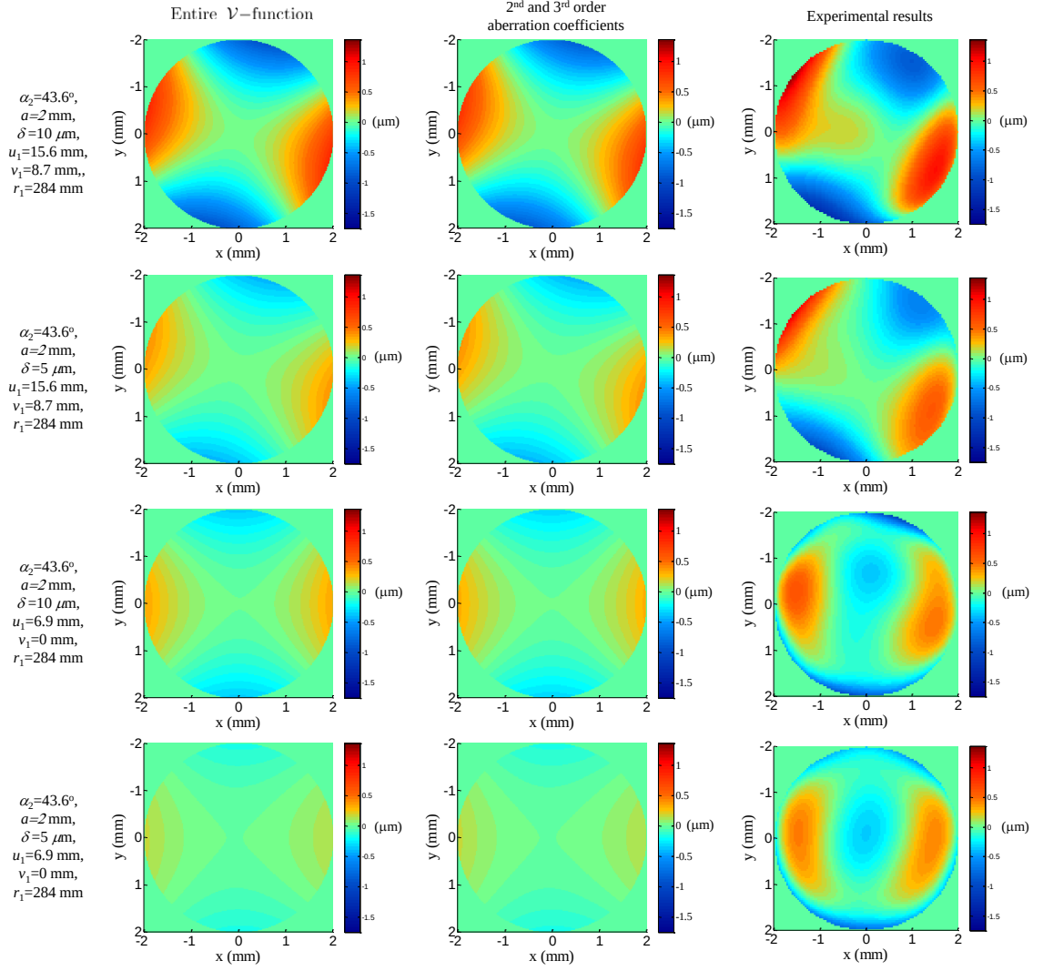
Figure 64: Wavefronts generated from the entire \mathcal{V} -function, 2 nd - and 3 rd -order aberration terms, and Zernike terms from the WFS for r_1 = 284 mm.
