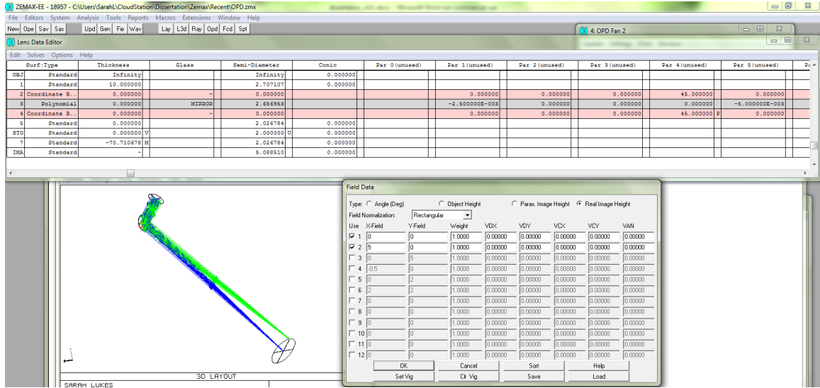
Figure 96: Lens Data Editor and 3D Layout in Zemax for 45^\circ incidence mirror, \delta = 20 \mu\text{m} , u_2 = 5 \text{ mm} , v_2 = 0 \text{ mm} , and r_1 = \infty .
