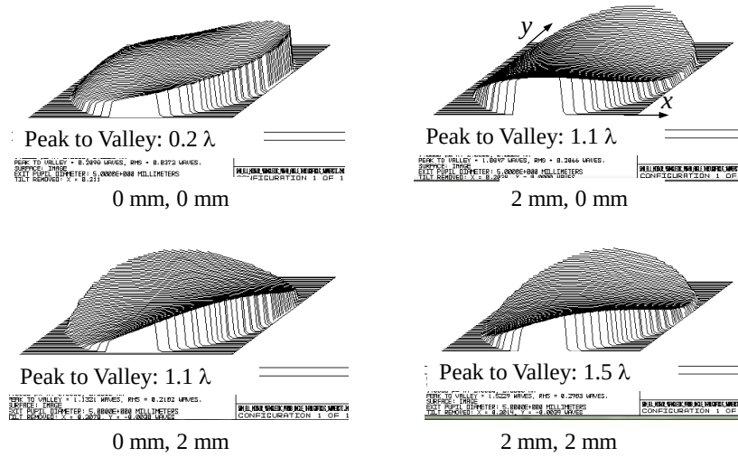
Figure 51: Zemax wavefront surfaces without tilt for four different image locations (u_2, v_2) to verify approximately 1 wave of astigmatism due to 2 nd -order aberration terms. A 5.000 mm x 7.071 mm elliptical-boundary mirror represented as an even polynomial ( Z = .0016X^2 + .0032Y^2 ) is analyzed here with \lambda = 1 \mu\text{m} . Variable r_1 is infinity and r_2 is 110 mm.
