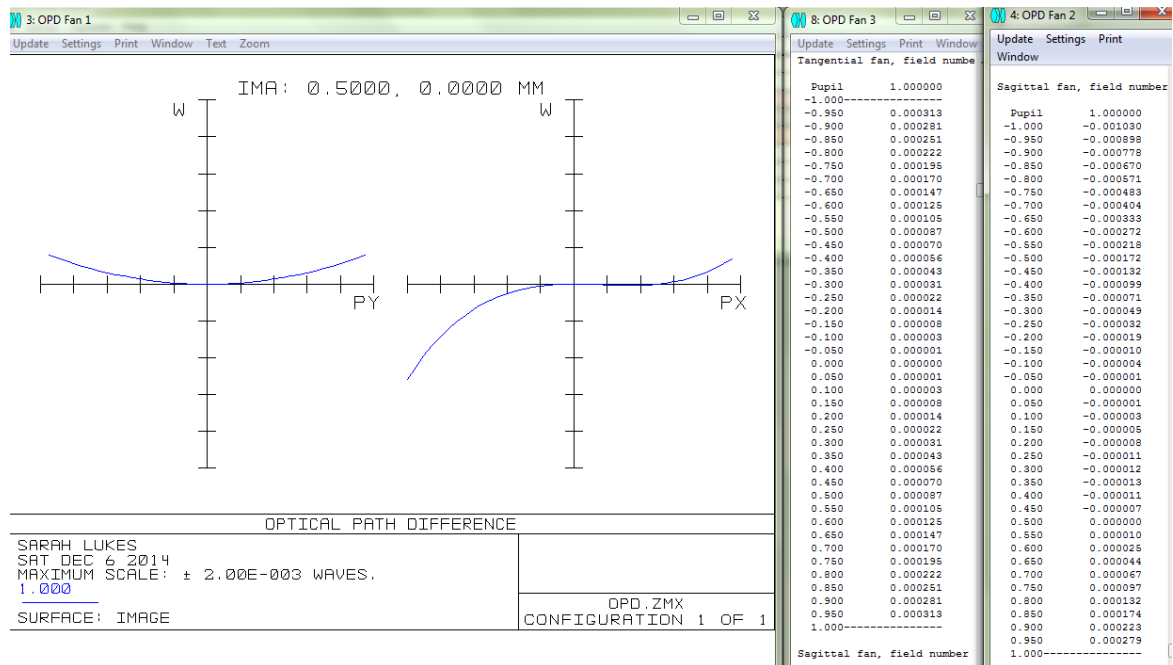
Figure 91: OPD fans in Zemax for 5° incidence mirror, \delta = 2 \mu\text{m} , u_2 = 0.5 \text{ mm} , v_2 = 0 \text{ mm} , and r_1 = \infty .
