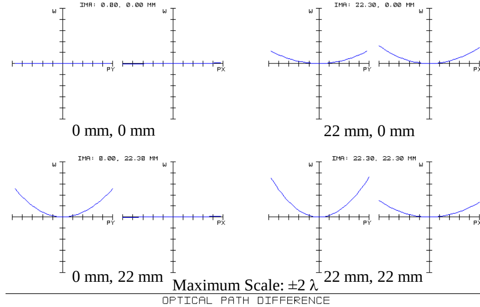
Figure 56: Zemax optical path difference fans for four different image locations (u_2, v_2) to verify approximately 1 wave of astigmatism due to 2 nd -order aberration terms. A 5.000 mm x 5.019 mm elliptical-boundary mirror represented as an even polynomial ( Z = .00226X^2 + .00227Y^2 ) is analyzed here with \lambda = 1 \mu\text{m} . Variable r_1 is infinity and r_2 is 110 mm.
