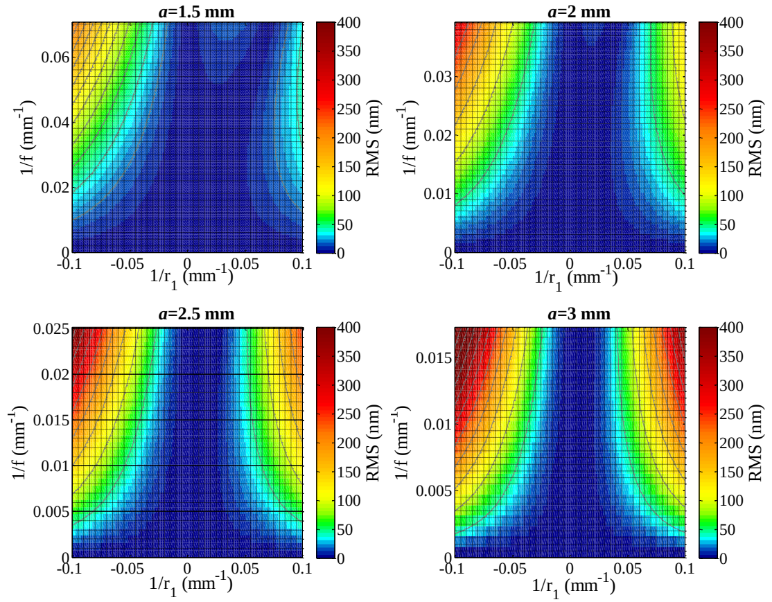
Figure 43: Wavefront RMS for MEMS mirrors with different radii. All graphs show results for \alpha_2 = 0^\circ with a deflection range of 0\text{ }\mu\text{m} to 40\text{ }\mu\text{m} . Mirrors with larger radii have less optical power for the same deflection as smaller radii mirrors.
