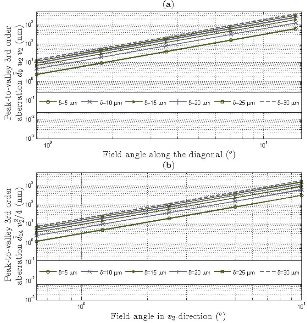
Figure 35: The 3 rd -order, peak-to-valley aberrations for various deflections and field angles of an a = 2 mm mirror with r_1 \rightarrow \infty . These two aberration terms, \tilde{d}_{g, r_1 \rightarrow \infty} , and \tilde{d}_{14, r_1 \rightarrow \infty} , have no dependence on \alpha_2 . The field angle along the diagonal means that u_2 = v_2 . For instance, if \text{atan}(u_2/r_2) = \text{atan}(v_2/r_2) = 3.54^\circ , then field angle along the diagonal is 5^\circ .
