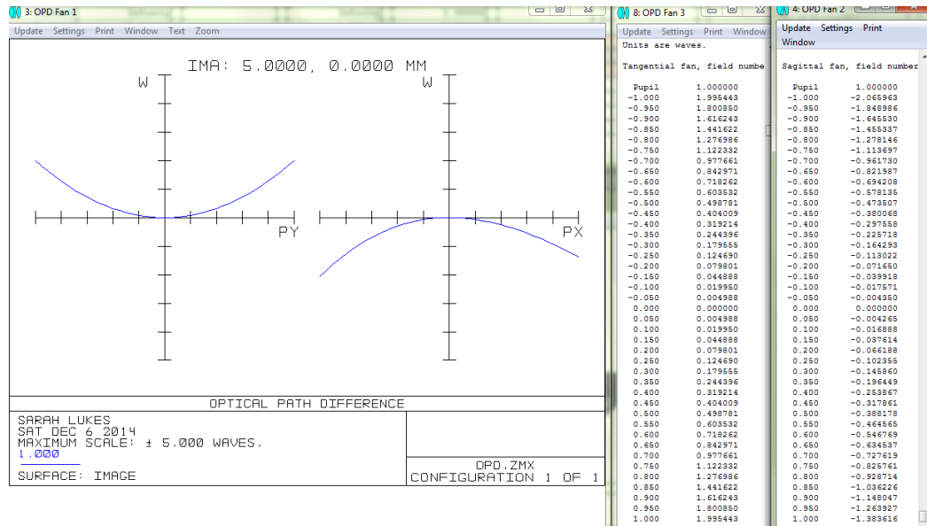
Figure 97: OPD fans from Zemax for 45^\circ incidence mirror, \delta = 20 \mu\text{m} , u_2 = 5 \text{ mm} , v_2 = 0 \text{ mm} , and r_1 = \infty .
