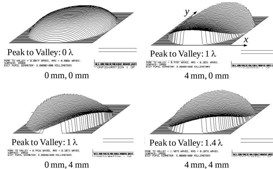
Figure 60: Zemax wavefront surfaces to verify approximately 1 wave of astigmatism due to 2 nd -order aberration terms. A 5.000 mm x 7.071 mm elliptical-boundary mirror represented as an even polynomial ( Z = .0016X^2 + .0032Y^2 ) is analyzed here with \lambda = 1 \mu\text{m} . Variables r_1 and r_2 are 221 mm.
