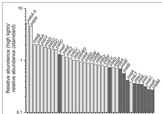
FIGURE 4 | Relative transcript levels of genes encoding components of photosystem I and photosystem II after a 1-h exposure to high light compared to standard conditions. The transcript level of genes encoding components of PS II (light gray) and PS I genes (dark gray) are displayed as the ratio of the relative transcript abundances for high-light-treated cells compared to the mean of three samples for standard conditions. A value of 1 represents an equal mRNA level under both conditions; values greater than 1 indicate an increase in relative transcript abundance; and values lower than 1 represent a decrease in relative transcript abundance after a 1-h exposure to high light.
