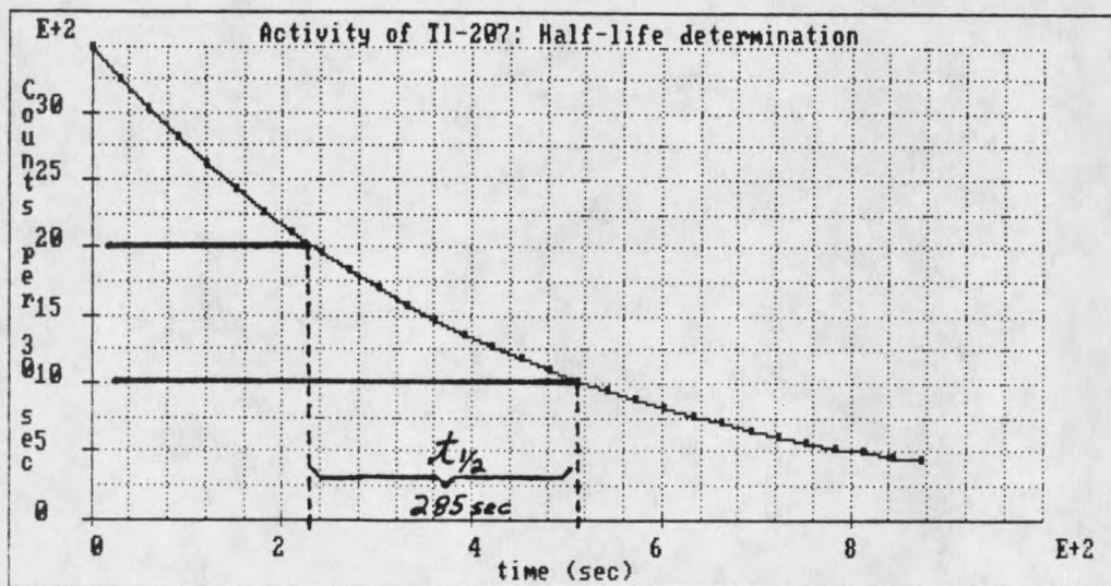
FIGURE 59. Decay Curve for Tl-207. The actual half life is 288 seconds.
