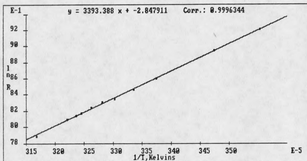
FIGURE 23. \ln(R) Versus 1/T for a 5-kohm Thermistor.
