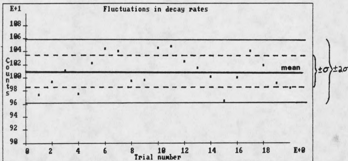
FIGURE 55. Counts Data with Lines Indicating \pm One and Two Standard Deviations of the Mean.
