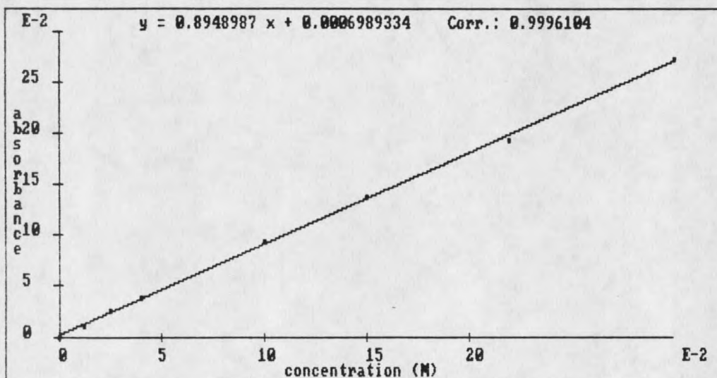
FIGURE 47. Beer's Law: Absorbance Versus Concentration for \text{Co}^{2+} Solutions.
