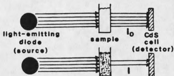
FIGURE 43. Principle Behind Beer's Law.
