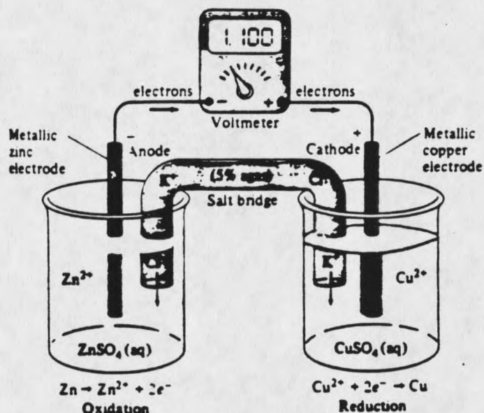
FIGURE 1. Daniell Cell (from Whitten, et.al. ).
