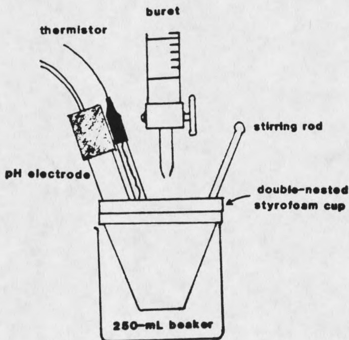
FIGURE 30. Experimental Set-up for Acid/Base Titrations.
