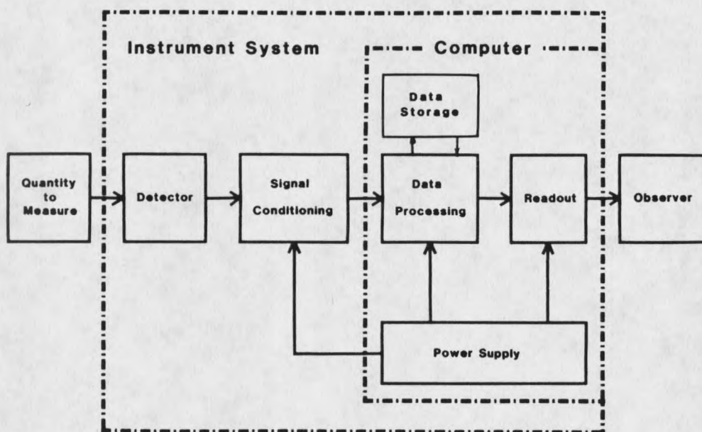
FIGURE 8. The Computer as Part of an Instrument System (75).
