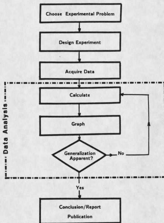
FIGURE 3. The Process of Science in the Laboratory (73).
