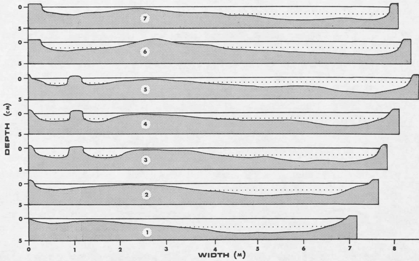
Figure 7. Cross-sections of test riffle at seven transects showing water levels at base flow (solid line) and 90% flow reduction (dotted line).
