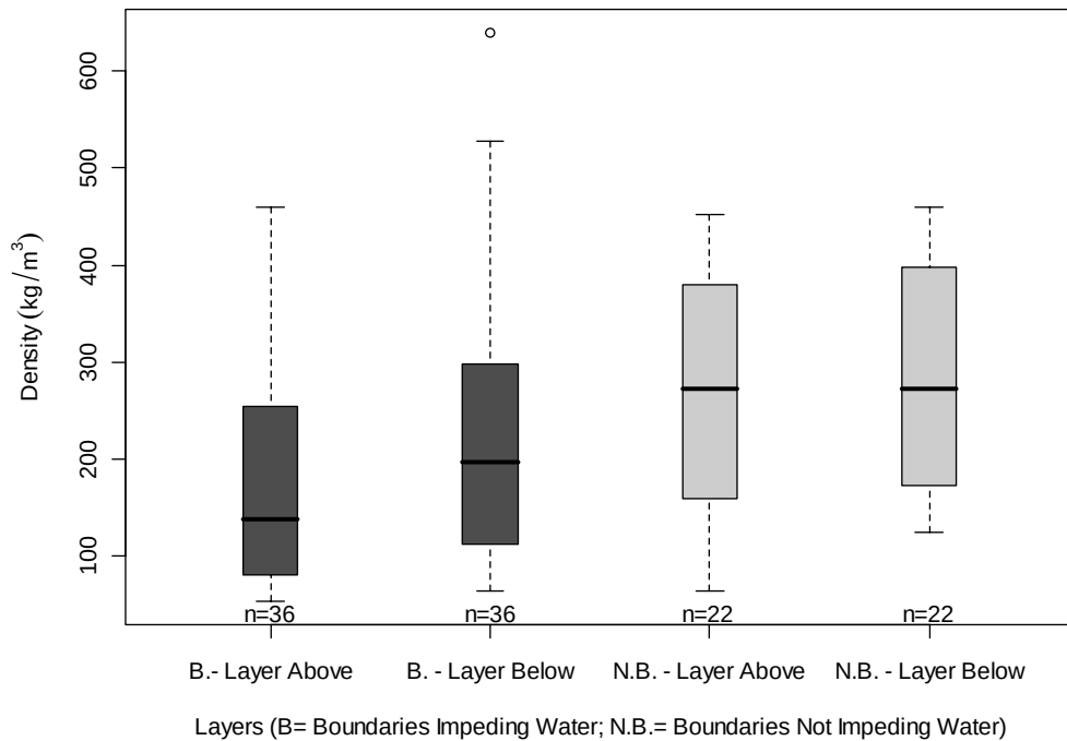
Figure 21: Box plot of density (kg/m³) of layers above and layers below transitions that impeded water and transitions that did not impede water. Thick black lines indicate median, boxes interquartile range, whiskers extend to the 0.05 and 0.95 quantiles, and the circles indicate outliers.
