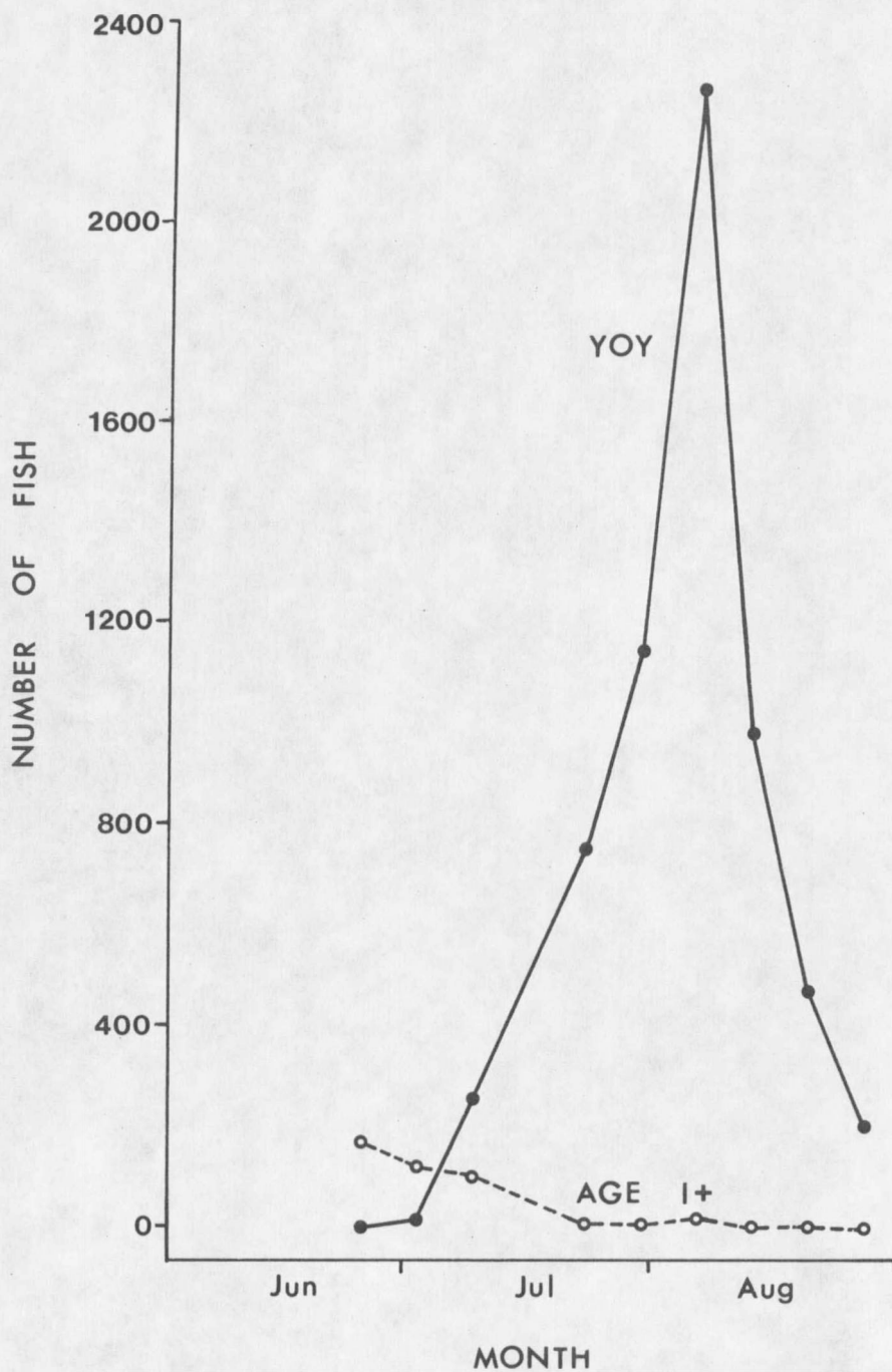
Figure 19. Weekly counts of rainbow trout emigrants from Beaver Creek into the Missouri River, June-August, 1983.
