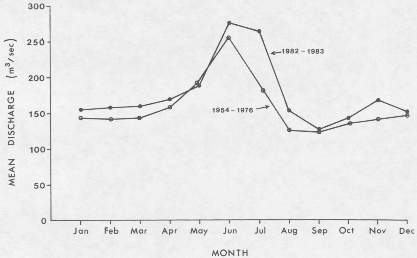
Figure 2. Mean monthly discharge of the Missouri River at Hauser Dam for the periods 1954-1976 and 1982-1983.
