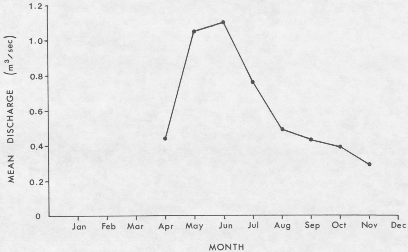
Figure 4. Mean monthly discharge of Beaver Creek, April -November, for the period 1982-1983.
