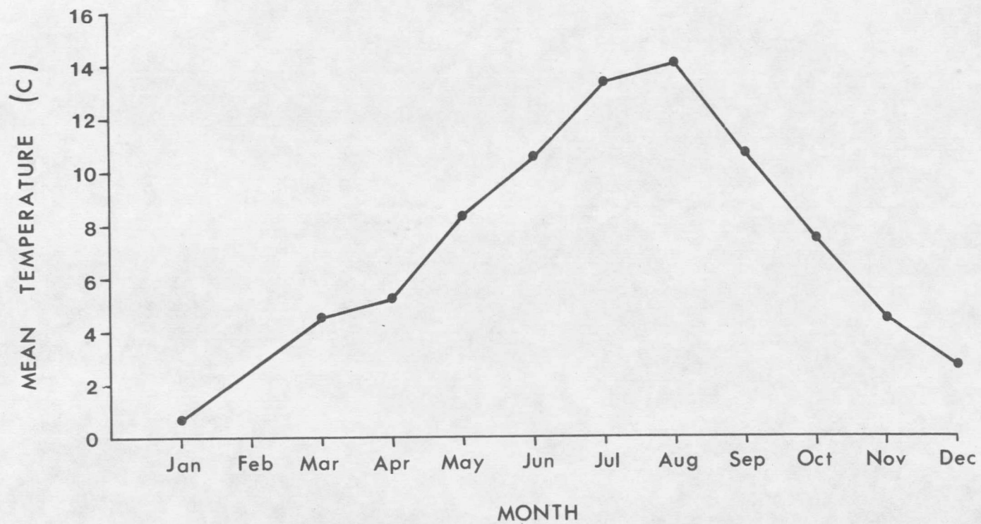
Figure 5. Mean monthly temperature of Beaver Creek for the period 1982-1983 (no data for February).
