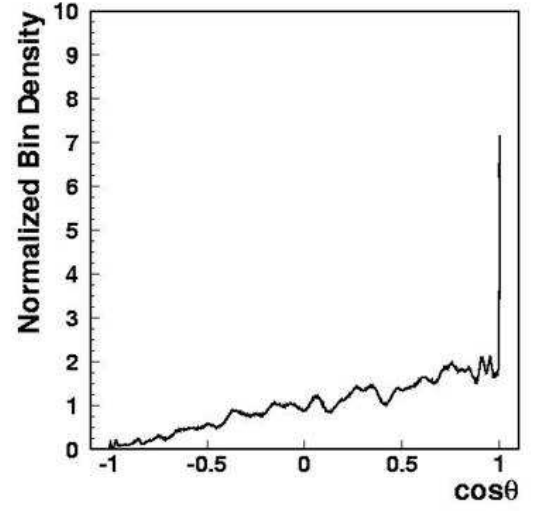
Figure 2.14: Autocorrelation observed in AGASA data.
