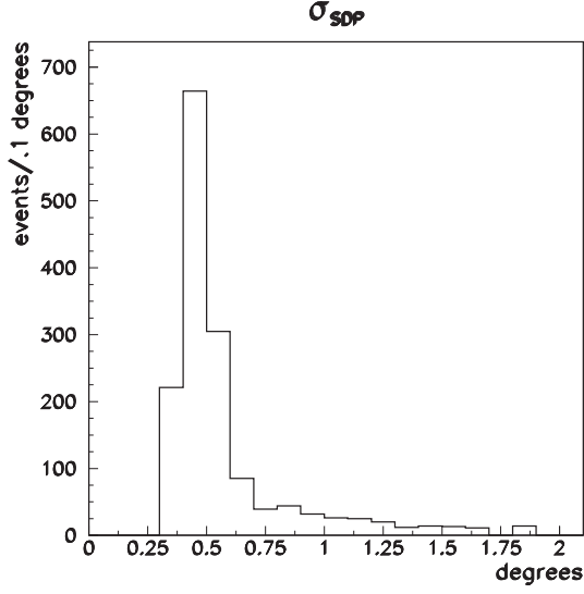
Figure 3.7: Distribution of \sigma_{SDP} for the HiRes-I monocular data set
