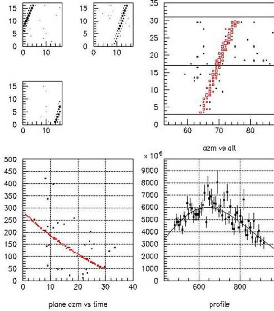
Figure 3.2: Diagrams of event reconstruction. A single event is shown triggering photomultiplier tubes in several arrays (upper left) and is reconstructed in altitude vs. azimuth (upper right). Time vs. azimuth is shown in the bottom left and intensity vs. penetration depth is shown on the bottom right.
