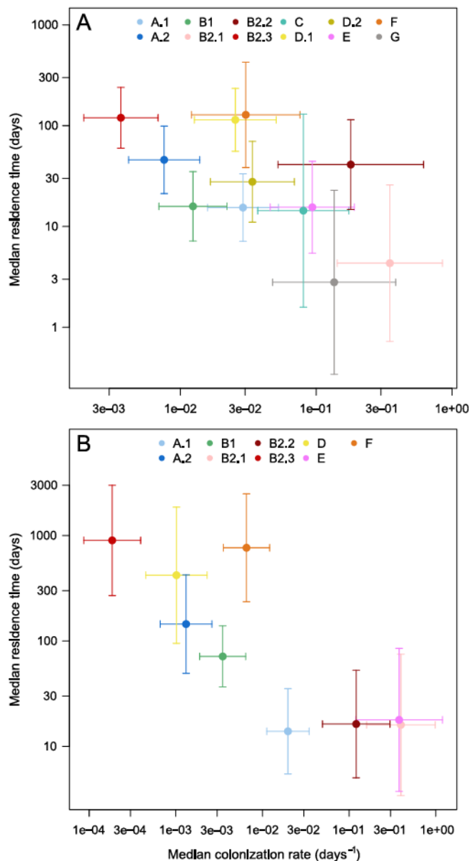
Figure 2. Median residence time as a function of the median colonization rate for each phylogroup appearing in the French (A) and the USA (B) datasets, for the average host and average values of the quantitative explanatory factors in their respective datasets. Estimates (dots) are represented with their 95% confidence interval (bars).
