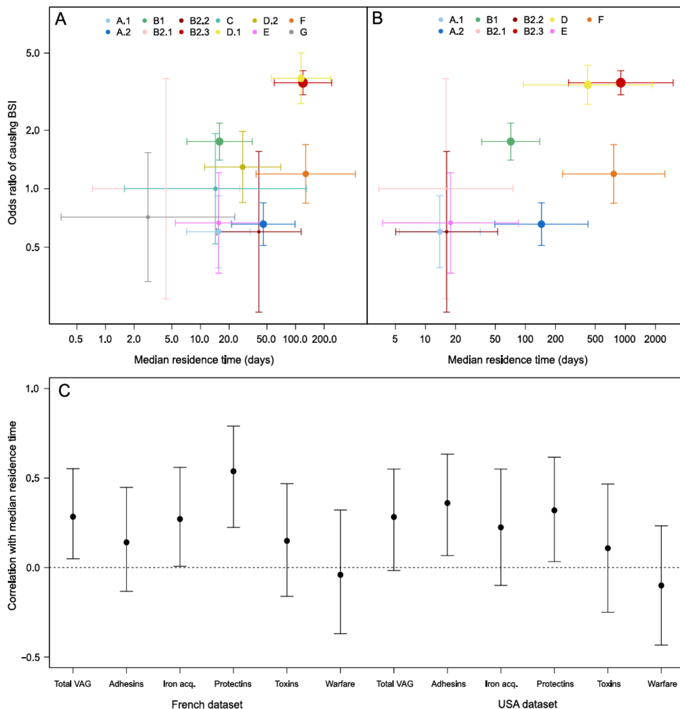
Figure 3. (A and B) Odds ratio of the association with bloodstream infections (BSI) as a function of median residence time for each phylogroup appearing in the French (A) and the USA (B) datasets. Estimates (dots) are represented with their 95% confidence interval (bars), with the size of the dots proportional to the number of samples of a given phylogroup used to estimate the odds ratios of causing BSI. (C) Correlation rate between the median residence time of each phylogroup estimated for the two datasets and its number of VAGs (total or associated with adhesins, iron acquisition systems, protectins, toxins, or bacterial warfare). Estimates (dots) are represented with their parametric bootstrap 95% confidence interval (bars). Correlations whose confidence interval does not include 0 are considered significant.
