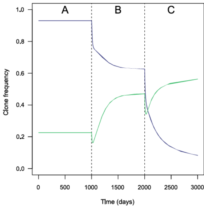
Figure 4. Variation in the frequencies of phylogroups x (purple) and y (green) over 3000 simulated days of the model with increasing levels of additive clearance ( \theta ), with R_x = 3.5 , R_y = 3 , b = 0 , b_s = -0.1 , and d = 0 . Three time-periods of 1000 days each (separated by dashed lines) are defined: no additive clearance ( \theta = 0 ) for t \in [0, 1000] (A), \theta = 0.1 for t \in [1000, 2000] (B), and \theta = 0.2 for t \in [2000, 3000] (C). Phylogroup x has a slower turnover than y. The phylogroup hierarchy is reversed for a high enough value of \theta .
