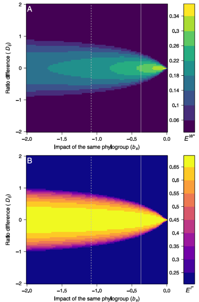
Figure 5. Asymptotic within-host coexistence E^{W*} (A) and inter-host coexistence E^{I*} (B) as a function of the ratio difference D_{ij} and the strength of clones of the same phylogroup on clearance b_s . Vertical lines correspond to the coefficients characterizing the impact of other clones of the same phylogroup from the best AFT models for the French (solid) and USA datasets (dashed). For these simulations, R_{ij} = 2 , b = 0 , d = 0 , E^{W*} \in [0, 1] and E^{I*} \in [0, \ln(2)] .
