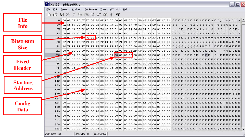
Figure 5.7: Hex translation of the partial BIT file for PicoBlaze tile 0.
