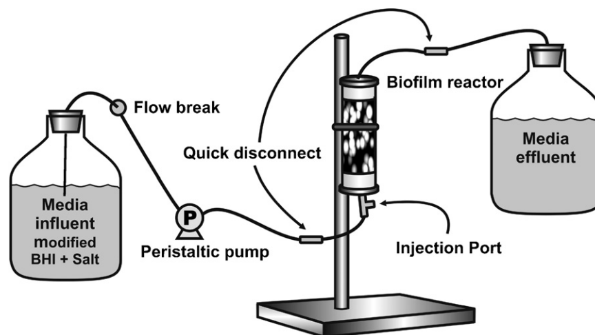
Fig. 1. Schematic of biofilm growth reactors used in this study.
