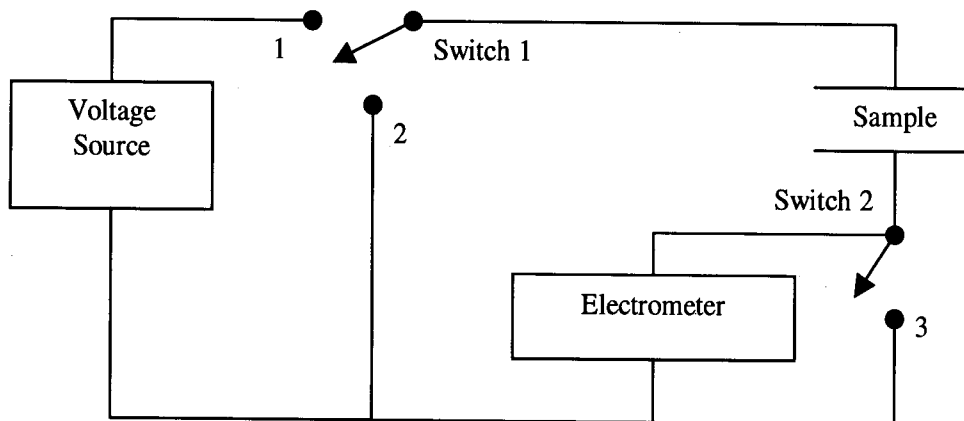
Figure 29. A schematic of the experimental setup for measuring transient response.
