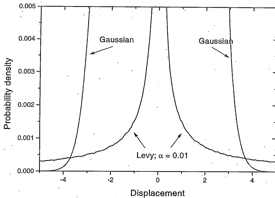
Figure 44. Comparison of the Lévy, or \alpha -stable, ( \alpha = 0.01 ) and Gaussian distributions in the cross-over regime.
