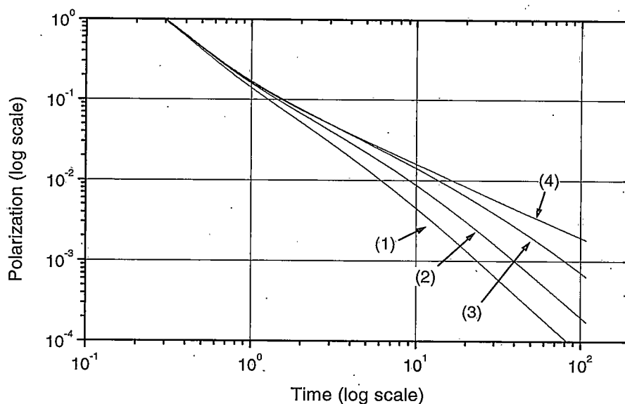
Figure 22. Polarization decay curves resulting from pulses of varying duration. The toy system has a time constant \tau = 0.1 \text{ sec} . Curve (1) is decay after pulse of 40\tau , curve (2) after pulse of 120\tau , curve (3) after pulse of 600\tau . Curve (4) is the fractional relaxation curve predicted by Equation 4.16.
