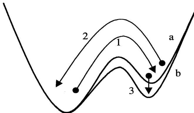
Figure 10. A schematic representation of the bound charge hopping model. The initial potential landscape is represented by curve (a). After a hop to the right (1), the particle can relax back to the initial state (2), or the environment can relax to curve (b) reducing the energy (3) resulting in reduced likelihood of return to the ground state.
