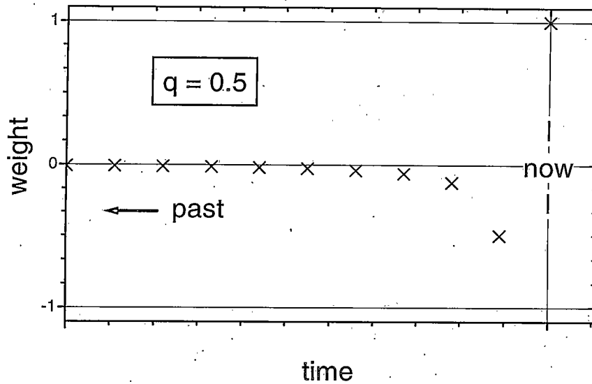
Figure 11. Linear plot of weights associated with the fractional derivative for q = 0.5 .
