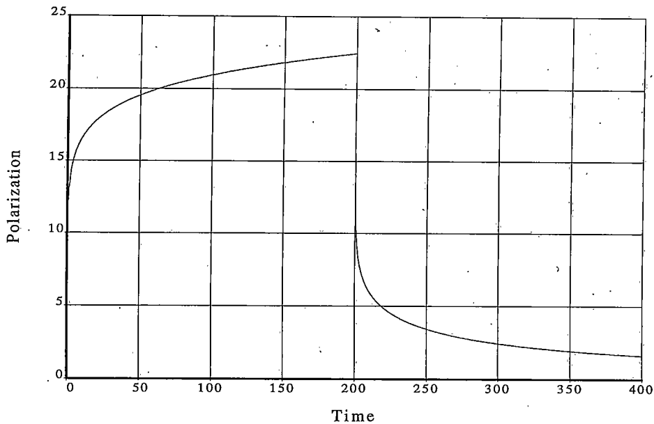
Figure 23. A time domain simulation reconstructing the response of the second toy system to a pulse 200 seconds ( 2000 \tau ) in duration. The exponent \delta = -0.1 for this case.
