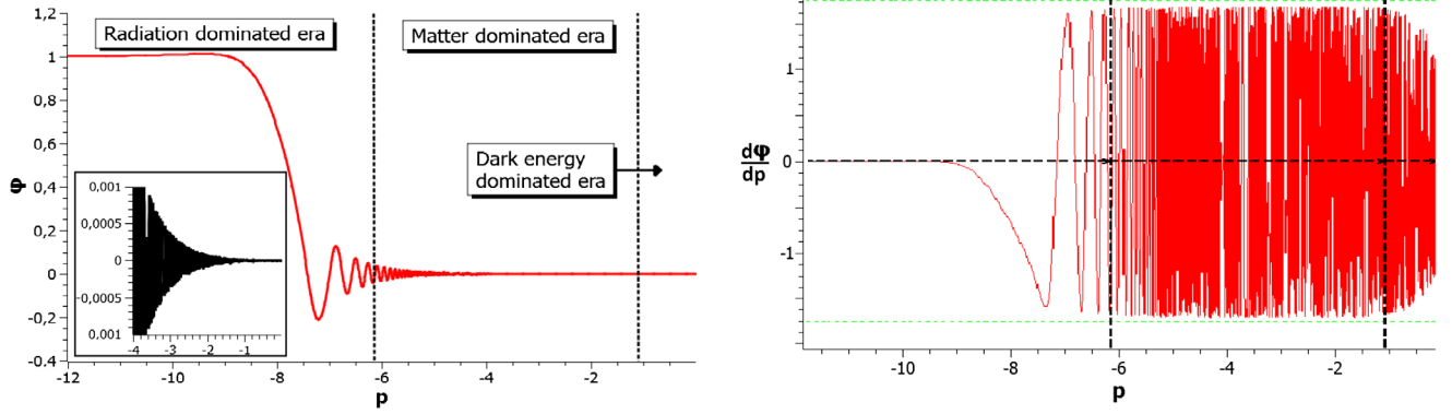
FIG. 1. Evolution of the scalar field (left panel) and its derivative (right panel) as functions of the dimensionless conformal p -time in massive DEF theory with \beta = -4.5 and m = 5.8 \times 10^{-28} eV. In both panels, the dashed vertical lines roughly separate the different cosmological eras (radiation, matter and dark energy). Observe that after a quiescent phase, the field begins to oscillate rapidly while its amplitude decays exponentially to zero. The amplitude of the envelope of its derivative grows during radiation and matter domination, approaching the limiting value of \sqrt{3} (horizontal dashed green lines on right panel) but decays during dark energy domination. The inset in the right panel shows the decay of the scalar field during the matter-dominated era and the dark-energy dominated era for p \geq -4 .
