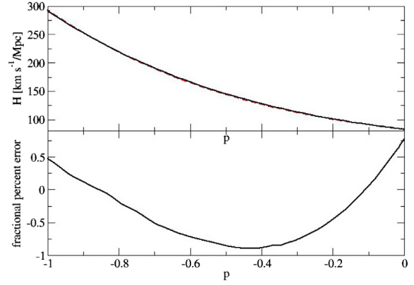
FIG. 2. Hubble parameter as a function of p -time for \beta = -4.5 , m = 5.8 \times 10^{-28} eV and \varphi_0 = 1 . Top: The Hubble parameter is computed first by solving the field equations numerically (dashed red line), and then fitting this data to the analytical approximate model of Eq. (64) (black line). Bottom: Fractional percent difference between the numerical and the analytical result. Observe that the error between the numerical solution and the analytic expression is at most approximately 1%.
