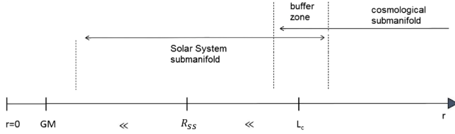
FIG. 4. Schematic representation of a spacelike hypersurface t = \text{cst} of the spacetime, the two submanifolds we consider, and the different scales at play in our perturbative scheme. The region r \gg L_c is dominated by cosmology and the behavior of the field is given in Sec. III. We are interested in computing observables in the Solar System submanifold, which is characterized by length scales of \mathcal{O}(R_{SS}) .
