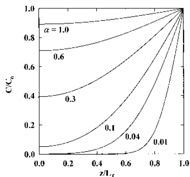
FIG. 1. Concentration profiles for unsteady-state diffusion in a slab of uniform thickness L_f . The parameter \alpha is dimensionless time.
