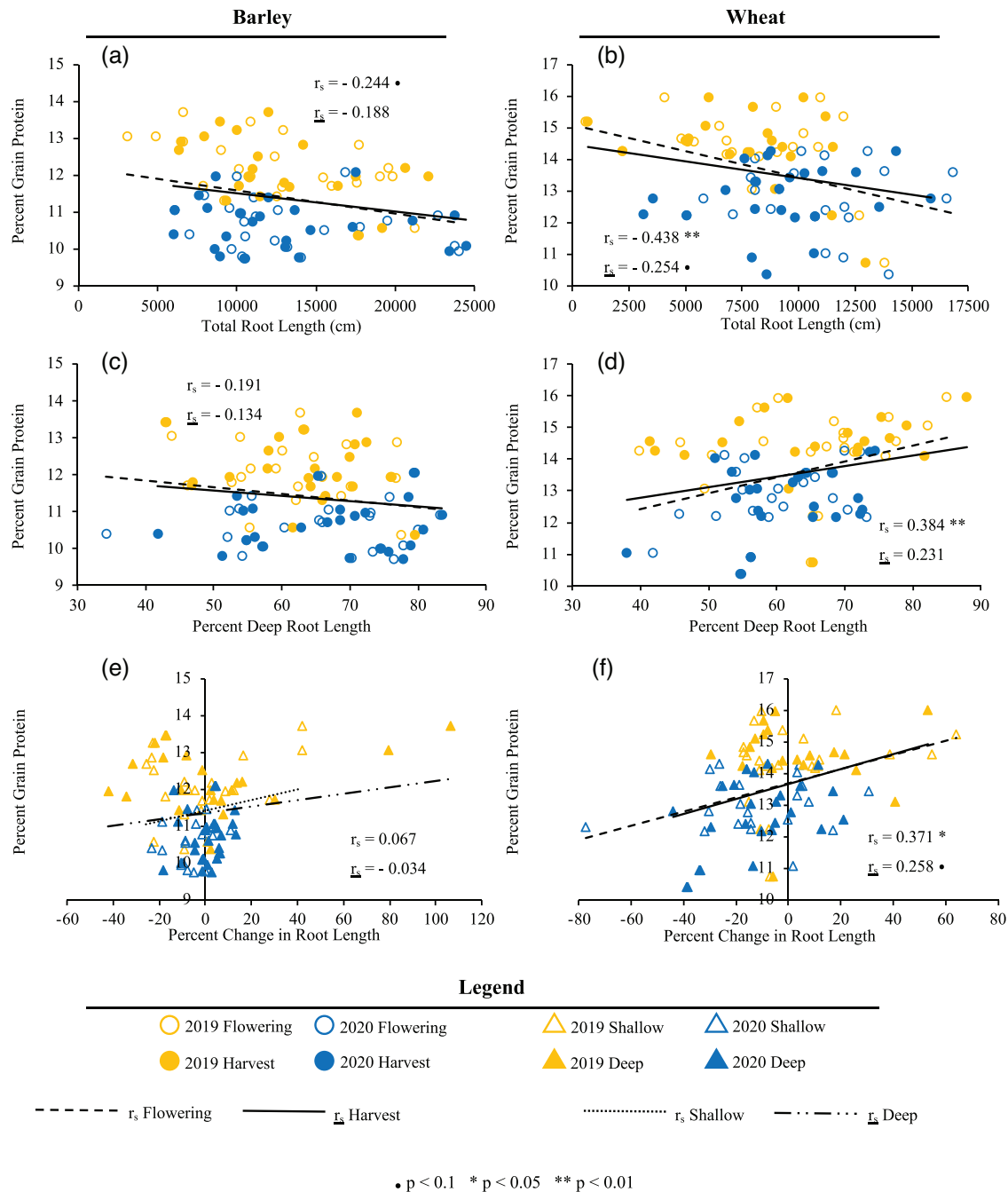
FIGURE 4 Correlations between percent grain protein and field root traits measured by minirhizotron. Points represent values measured on a single plot. Trendlines and Spearman correlation coefficients ( r_s ) are from all seasons combined. A, C, E: Barley. B, D, F: Wheat. A, B: Percent grain protein and total root length at flowering and harvest. C, D: Percent grain protein and percent deep root length (Equation 1) at flowering and harvest. E, F: Percent grain protein and percent change (Equation 2) in shallow and deep root length between flowering and harvest (during grain fill)
