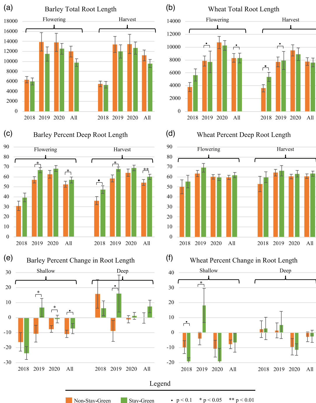
FIGURE 2 Means of non-stay-green and stay-green groups of lines, with p values from ANOVA for the fixed effect of stay-green for field root traits measured by minirhizotrons. Sample sizes are listed in corresponding Supplemental Table S2. A, C, E: Barley. B, D, F: Wheat. A, B: Total root length at flowering and harvest. C, D: Percent deep root length (Equation 1) at flowering and harvest. E, F: Percent change (Equation 2) in shallow and deep root length between flowering and harvest (during grain fill)
