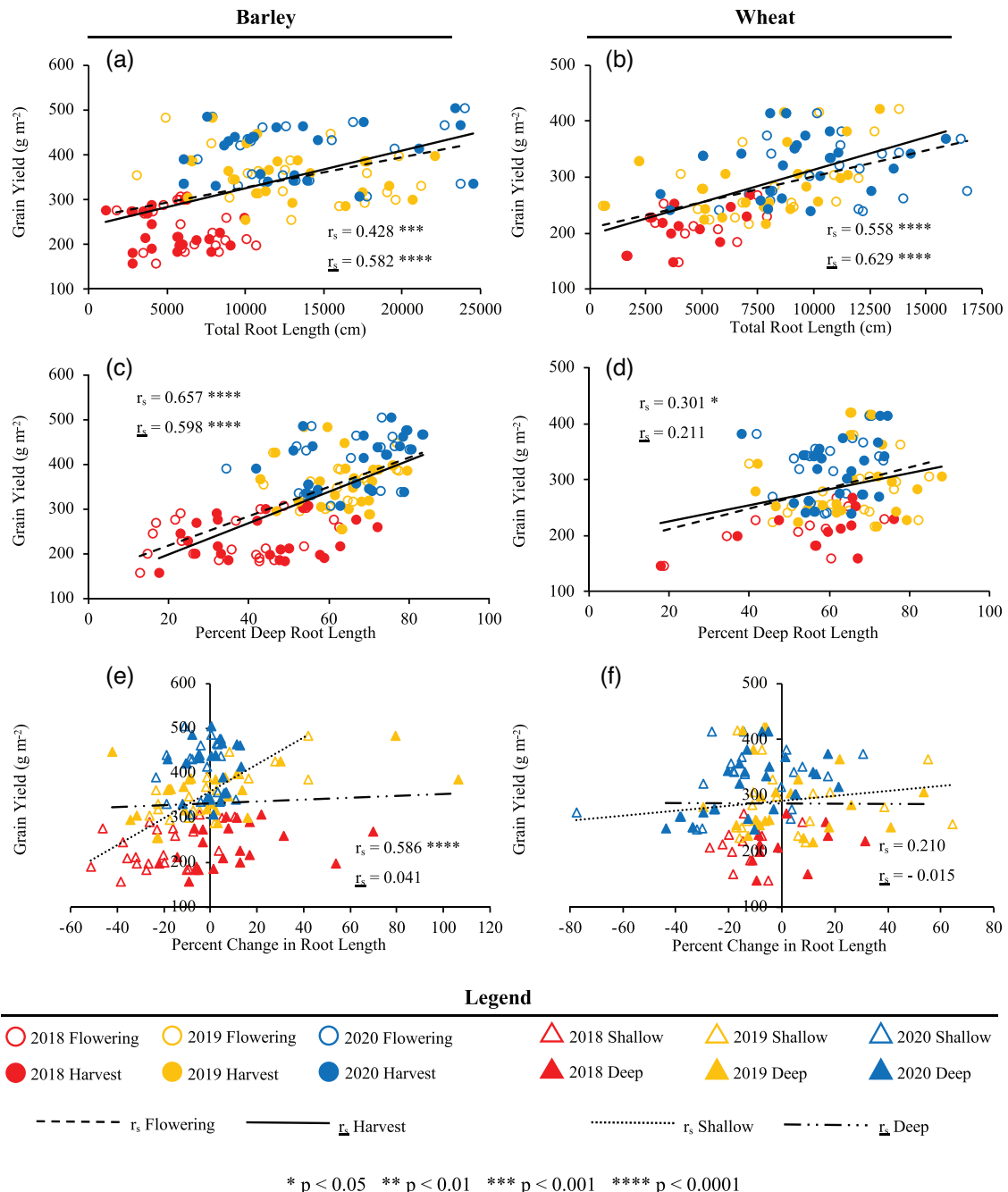
FIGURE 3 Correlations between grain yield and field root traits measured by minirhizotron. Points represent values measured on a single plot. Trendlines and Spearman correlation coefficients ( r_s ) are from all seasons combined. A, C, E: Barley. B, D, F: Wheat. A, B: Grain yield and total root length at flowering and harvest. C, D) Grain yield and percent deep root length (Equation 1) at flowering and harvest. E, F: Grain yield and percent change (Equation 2) in shallow and deep root length between flowering and harvest (during grain fill)
