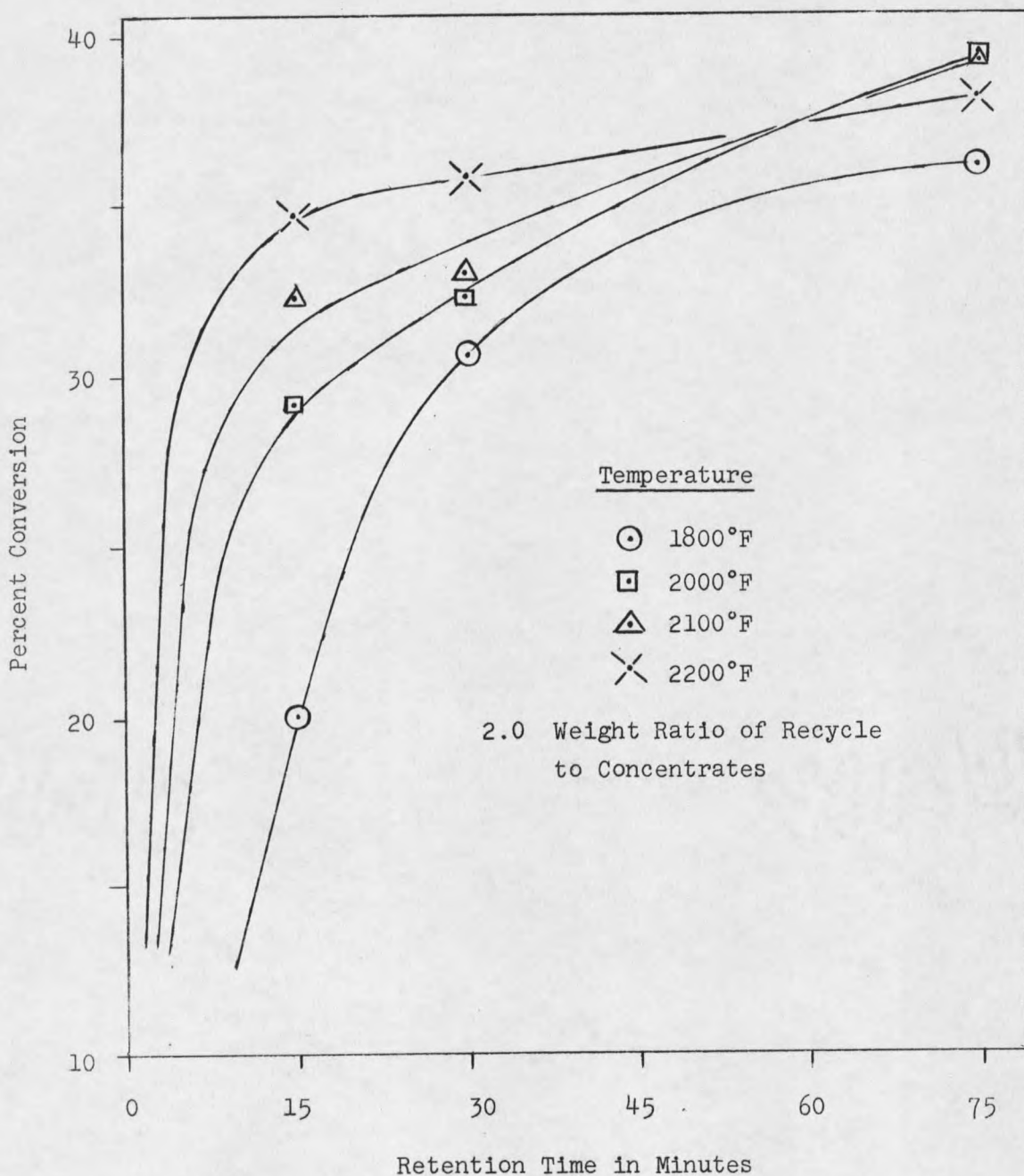
Figure 8. Plot of Percent Conversion vs. Retention Time for Muffle Samples Containing 20 Wt.% \text{Na}_2\text{CO}_3
