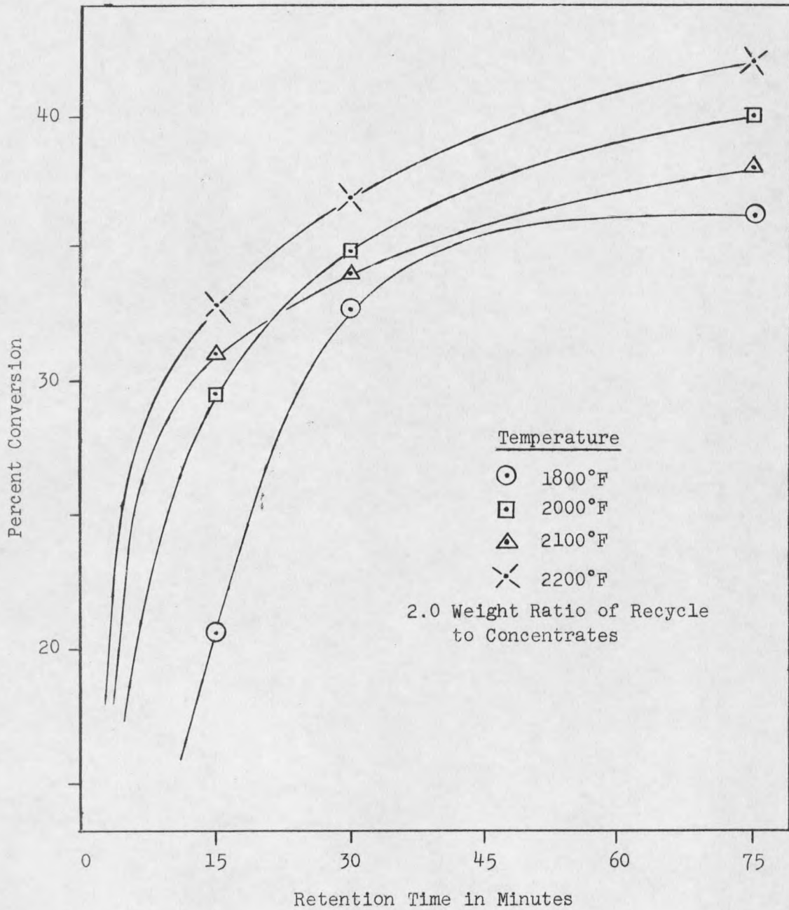
Figure 9. Plot of Percent Conversion vs. Retention Time for Muffle Samples Containing 22 Wt.% \text{Na}_2\text{CO}_3
