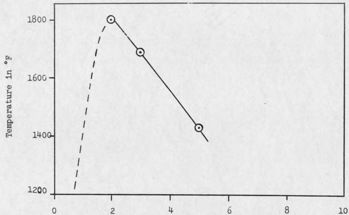
Figure 5. Plot of Temperature vs. Position Down Length of Rotary Kiln
