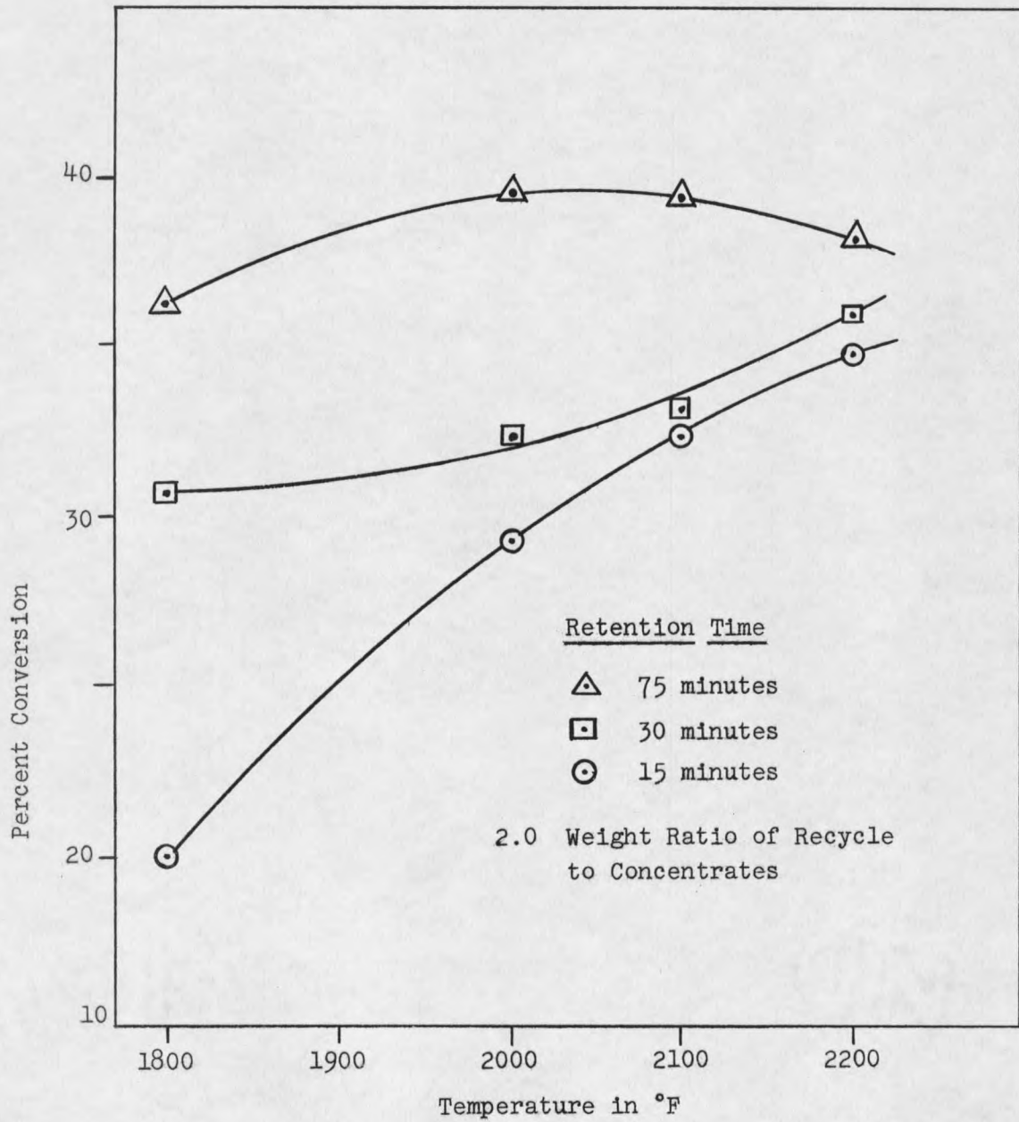
Figure 6. Plot of Conversion vs. Temperature for Muffle Samples Containing 20 Wt.% \text{Na}_2\text{CO}_3
