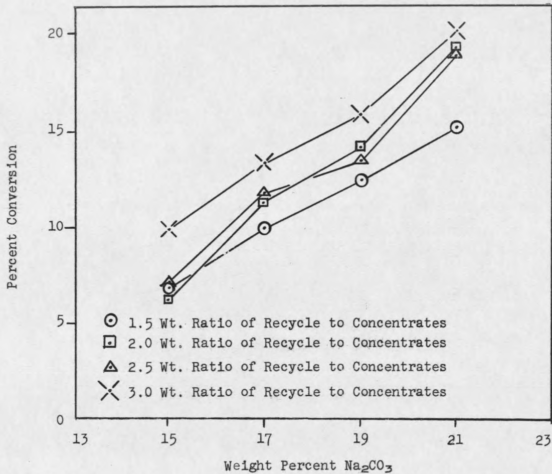
Figure 4. Plot of Conversion vs. Weight Percent \text{Na}_2\text{CO}_3 for Rotary Kiln Samples
