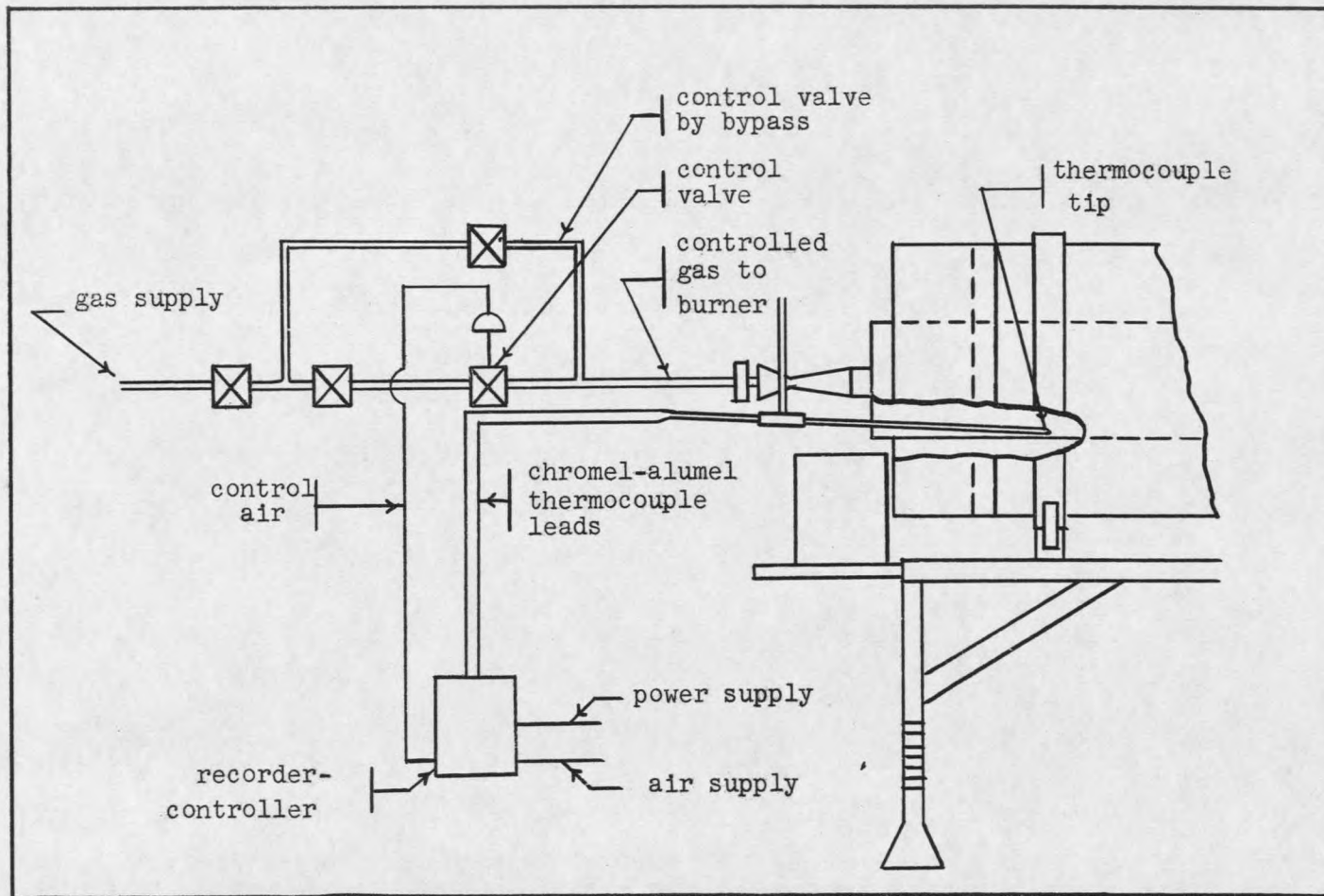
Figure 2. Kiln Temperature Control System
