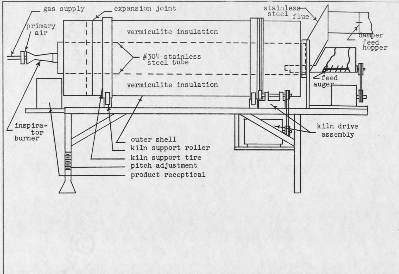
Figure 1. Laboratory Rotary Kiln
