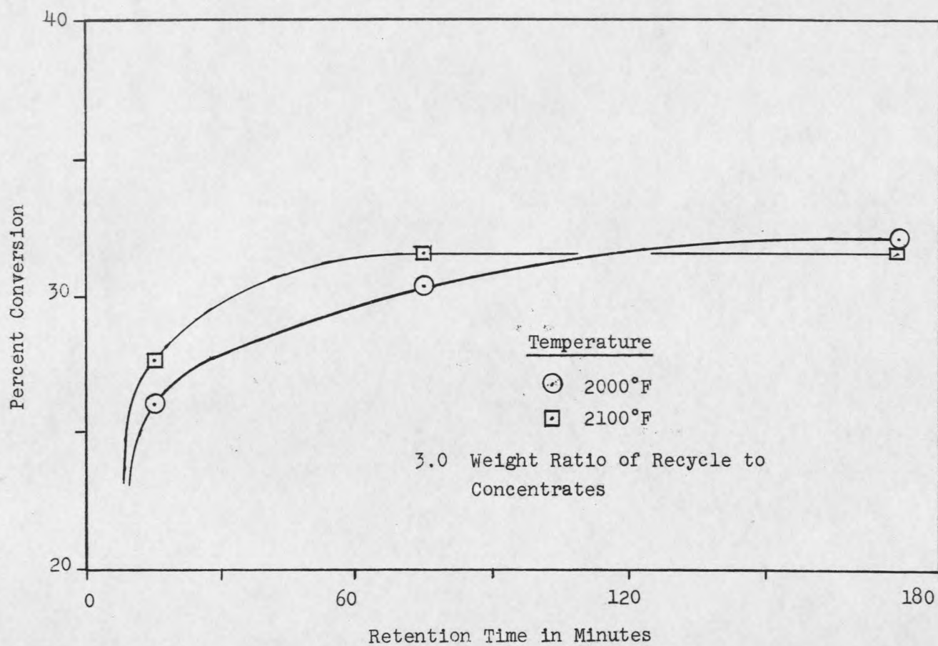
Figure 10. Plot of Percent Conversion vs. Retention Time for Muffle Samples Containing 17 Wt.% \text{Na}_2\text{CO}_3
