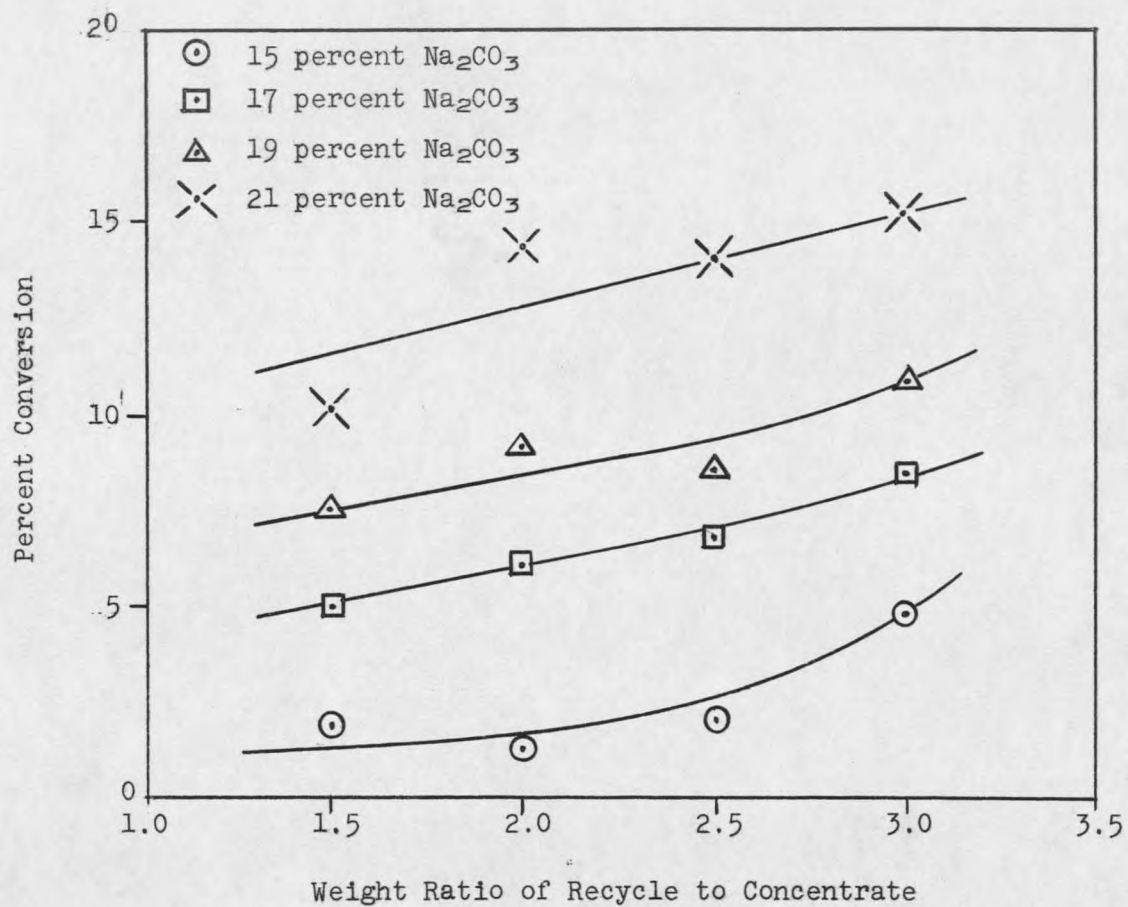
Figure 3. Plot of Conversion vs. Weight Ratio of Recycle to Concentrates for Rotary Kiln Samples
