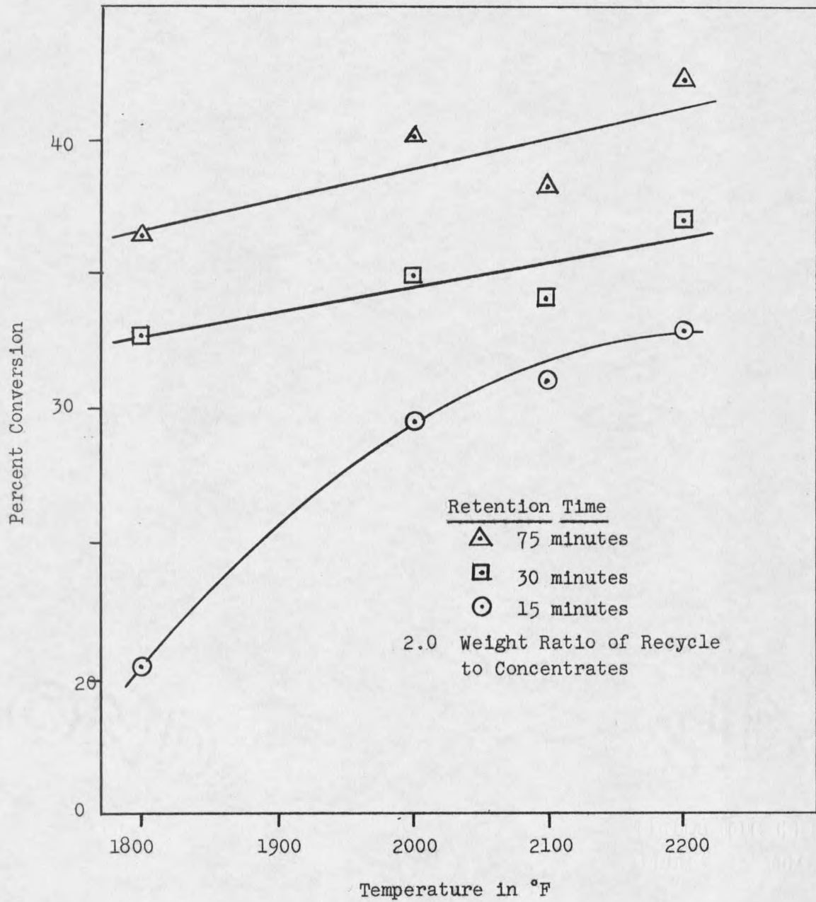
Figure 7. Plot of Conversion vs. Temperature for Muffle Sample Containing 22 Wt.% \text{Na}_2\text{CO}_3
