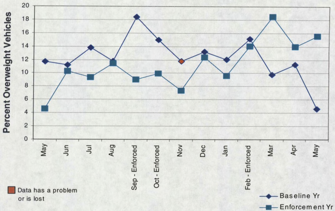
Figure 9. Percent Overweight Commercial Vehicles by Month at the Decker STARS Site, Baseline and Focused Enforcement Years.
