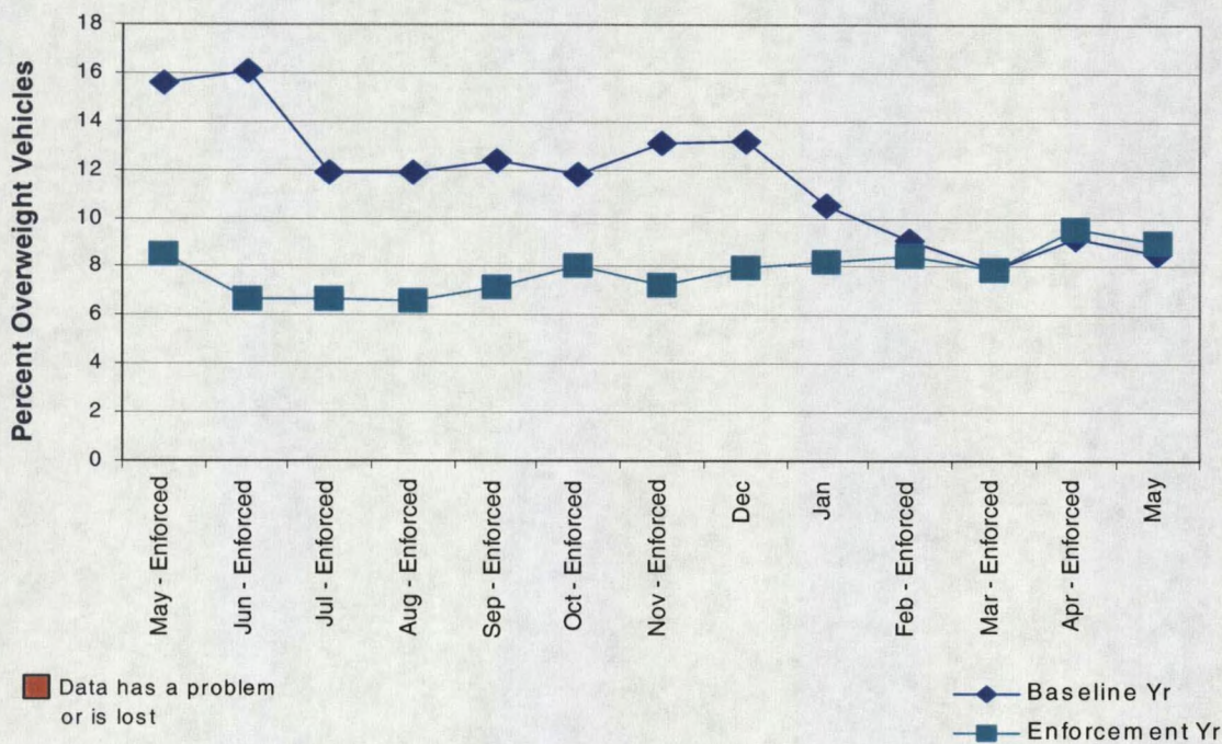
Figure 8. Percent Overweight Commercial Vehicles by Month at the Stanford STARS Site, Baseline and Focused Enforcement Years.
