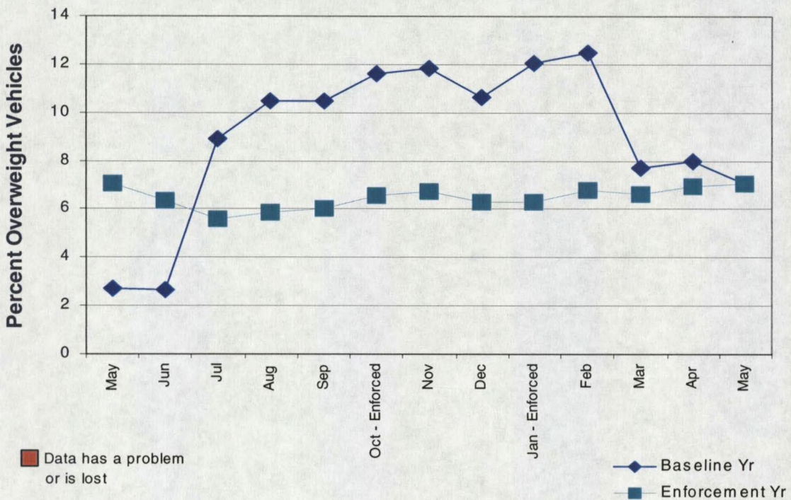
Figure 10. Percent Overweight Commercial Vehicles by Month at the Manhattan STARS Site, Baseline and Focused Enforcement Years.
