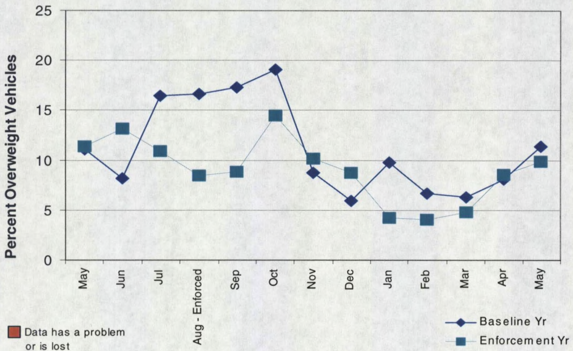
Figure 12. Percent Overweight Commercial Vehicles by Month at the Miles City East STARS Site , Baseline and Focused Enforcement Years.
