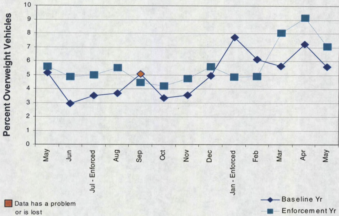
Figure 11. Percent Overweight Commercial Vehicles by Month at the Arlee STARS Site , Baseline and Focused Enforcement Years.
