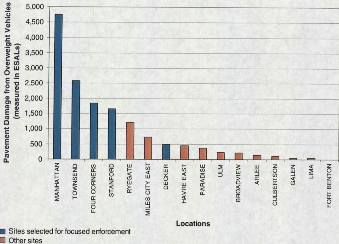
Figure 4. Typical Pavement Damage (measured in ESALs) for each STARS Site for October 2000 (Baseline Year).
