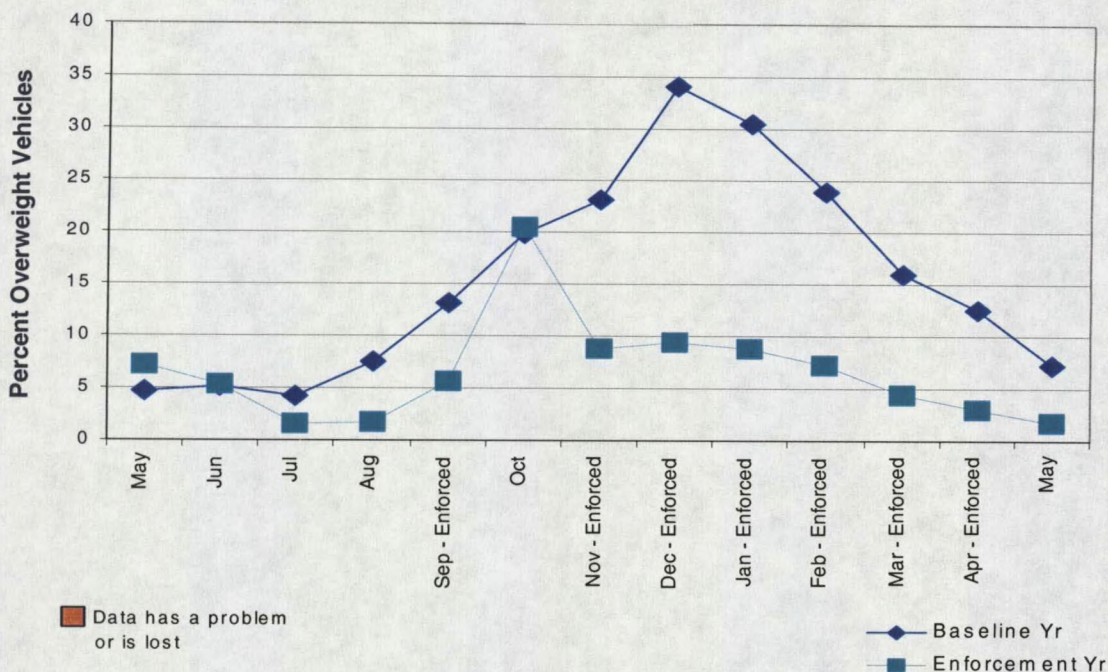
Figure 7. Percent Overweight Commercial Vehicles by Month at the Ryegate STARS Site, Baseline and Focused Enforcement Years.
