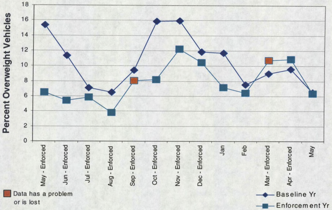
Figure 5. Percent Overweight Commercial Vehicles by Month at the Townsend STARS Site, Baseline and Focused Enforcement Years.
