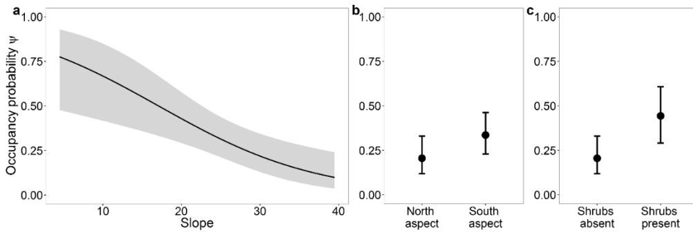
Figure 2.0.3. Changes in occupancy (and 95% CI) of hoary marmots with (a) slope, (b) aspect categorized as North or South, and (c) presence or absence of shrub cover, northwestern Montana, summers 2014 and 2015.
