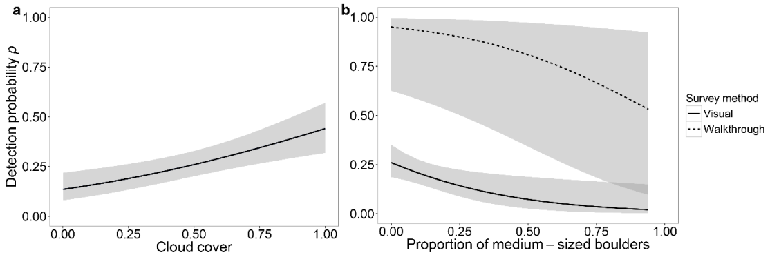
Figure 2.0.2. Changes in detection probability (and 95% CI) for hoary marmots during occupancy surveys, northwestern Montana, summers 2014 and 2015. (a) Detection probability during visual surveys over the observed range of overhead cloud cover. (b) Detection probabilities by survey method over the observed range of medium-sized boulders.
