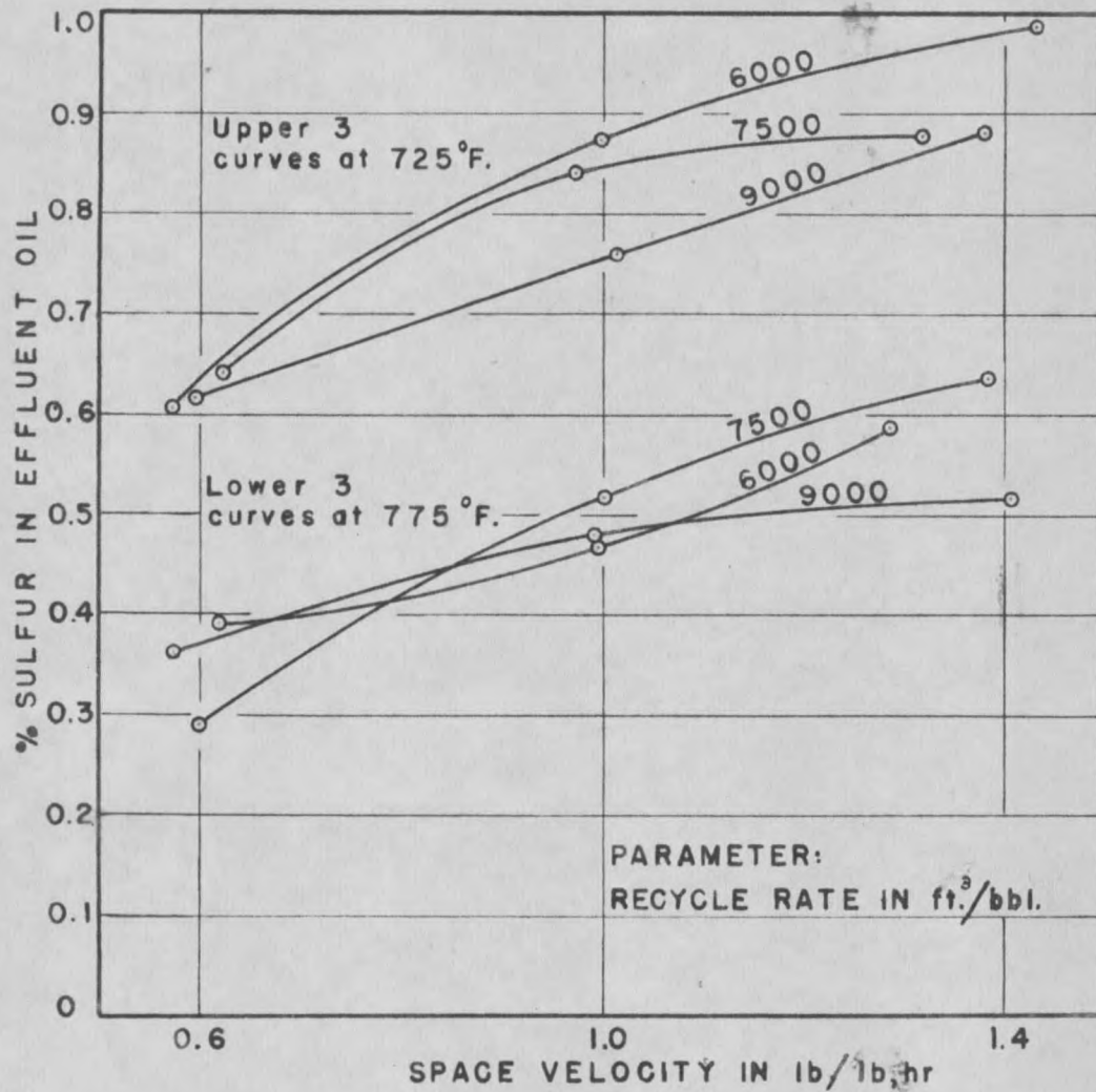
Figure 2. Percent Sulfur in Effluent Oil Versus Space Velocity. Molybdenum Oxide Statistical Run (Set 2).
