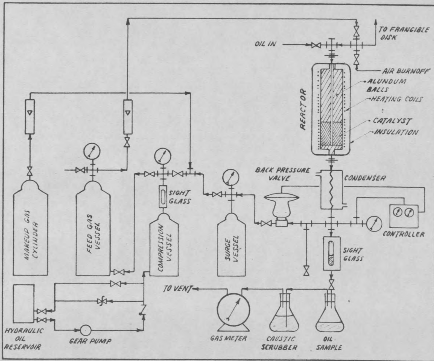
Figure 1. Schematic Flow Diagram of Desulfurization Unit
