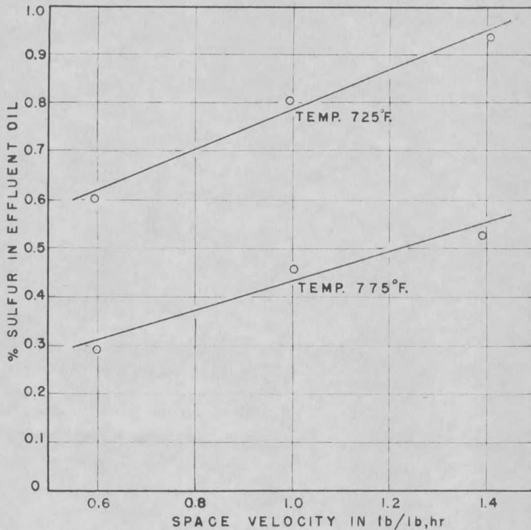
Figure 4. Effect of Space Velocity on Percent Sulfur in Effluent Oil. Molybdenum Oxide Statistical Runs (Sets 1 and 2).
