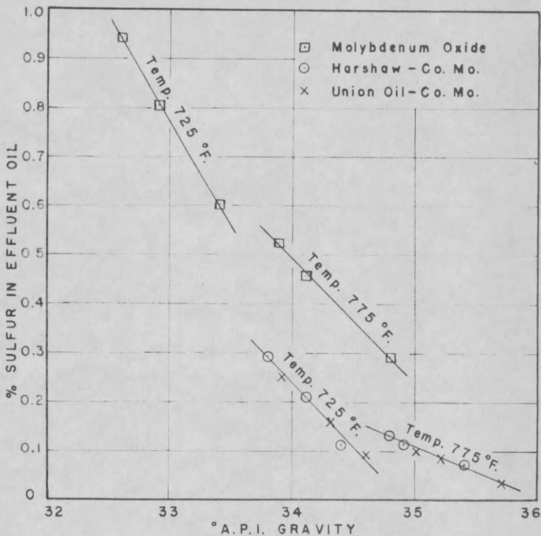
Figure 8. Percent Sulfur in Effluent Oil Versus °A.P.I. Gravity.
