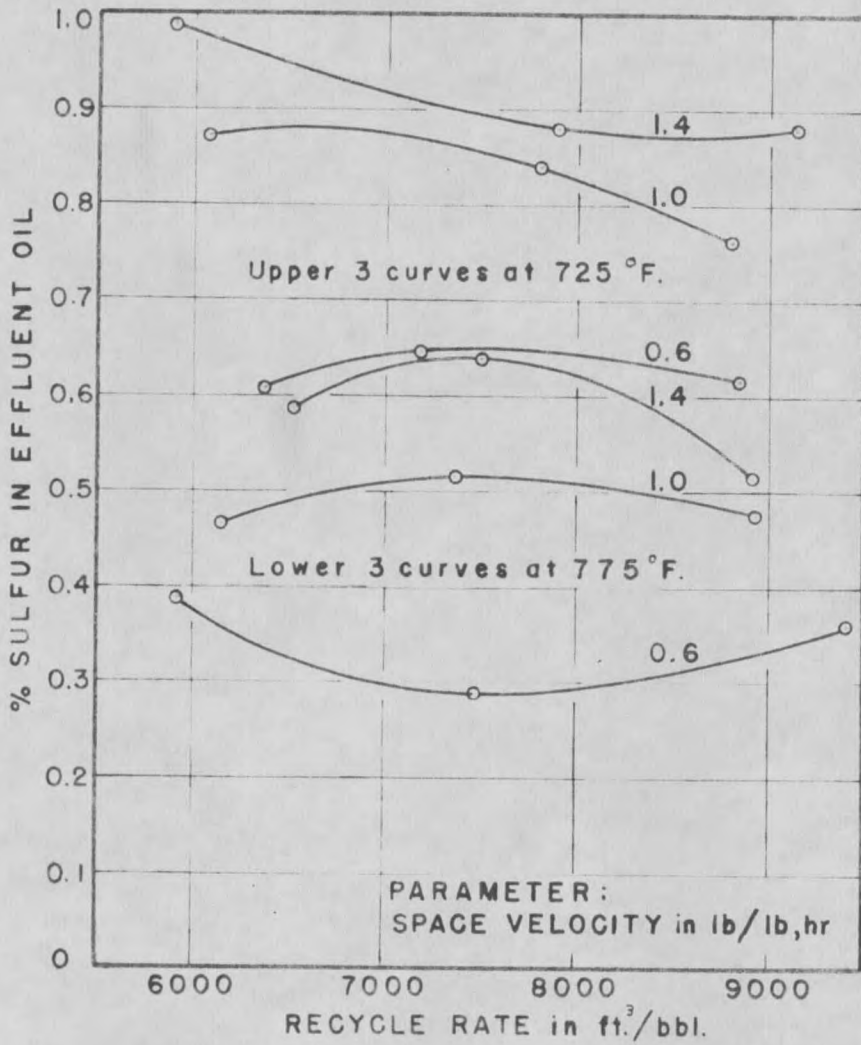
Figure 3. Percent Sulfur in Effluent Oil Versus Recycle Rate. Molybdenum Oxide Statistical Run (Set 2)
