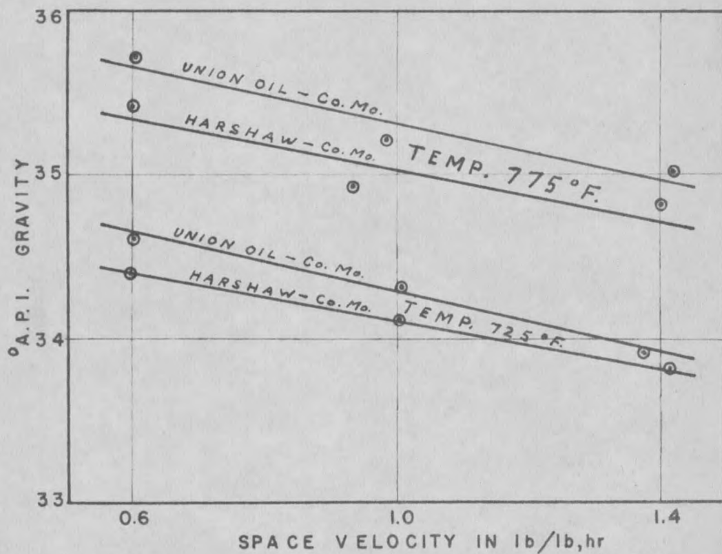
Figure 7. Effect of Space Velocity on °A.P.I. Gravity. Cobalt Molybdate Statistical Runs (Sets 3 and 4).
