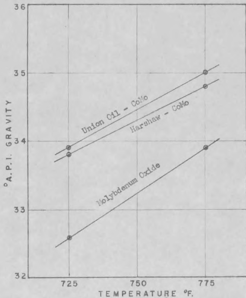
Figure 9. Effect of Temperature on API Gravity.
