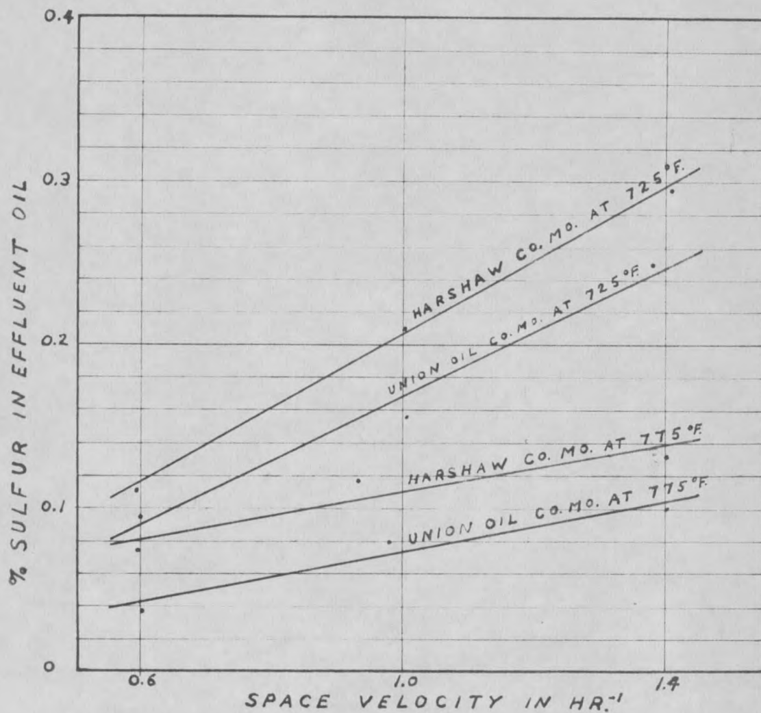
Figure 5. Effect of Space Velocity on the Percent Sulfur in the Effluent Oil. Cobalt Molybdate Statistical Runs (Sets 3 and 4).
