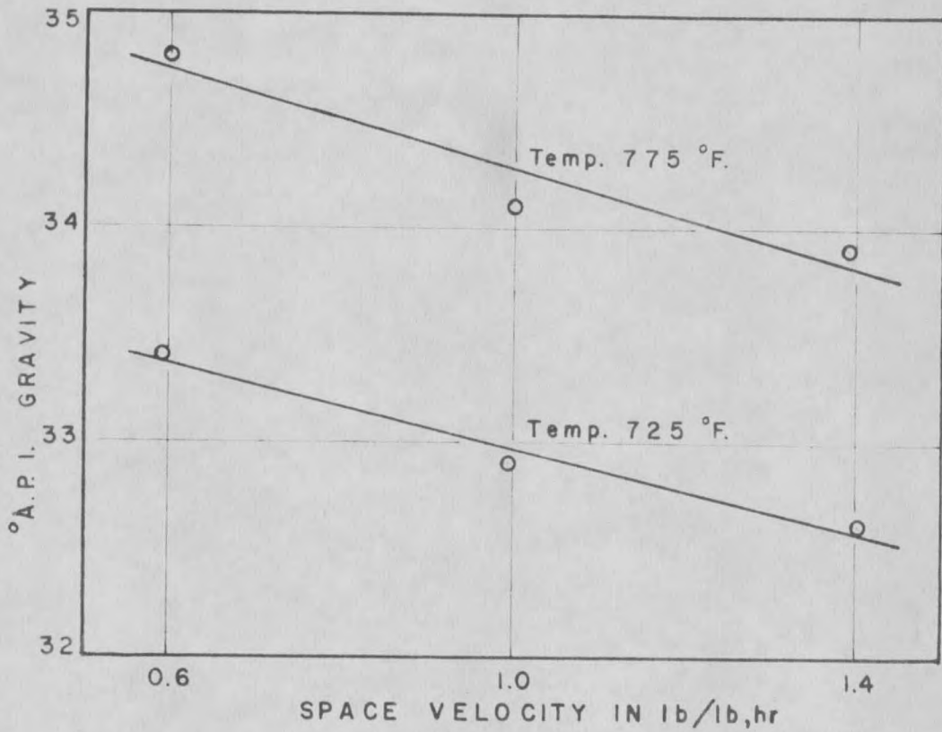
Figure 6. Effect of Space Velocity on °A.P.I. Gravity. Molybdenum Oxide Statistical Runs (Sets 1 and 2).
