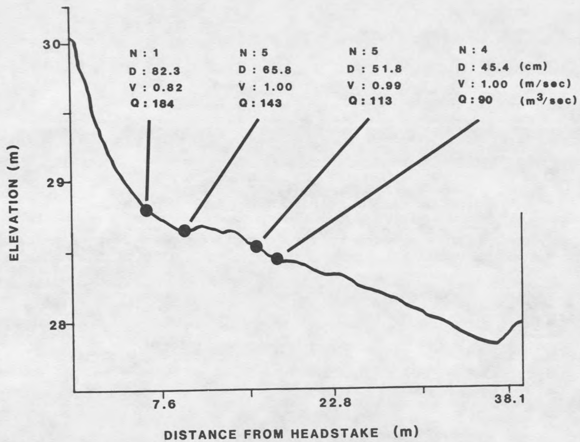
Figure 12. Relationship between spawning aggregations and hydraulic variables along a single, cross sectional transect at four discharges, Missouri River study area (1981-83) (N = Number of redds, D = Depth, V = Mean column velocity, Q = Discharge).
