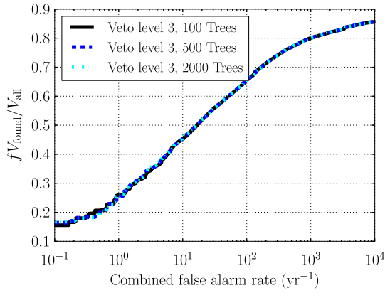
FIG. 3 (color online). Investigation of the effect of using a different number of trees on the recovery of q = 1 EOBNRv2 simulated waveforms at Veto Level 3. In general, we find that the use of more than 100 trees gives roughly the same sensitivity regardless of mass ratio or veto level. In this ROC, to adjust for the loss in analysis time in moving from Veto Level 2 to Veto Level 3, we scale the volume fraction in Eq. (8) by the ratio of analysis times f = t_{VL3}/t_{VL2} . From the analysis times reported in Sec. III, we find f = 0.88 .
