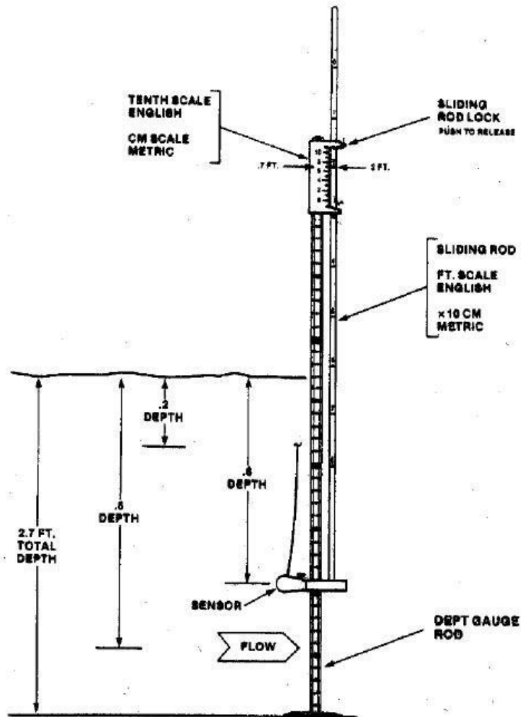
Figure 3. Top Setting Rod – Obtained from Holly Kreiner at the MSU Extension, from the Water Quality SOP for Discharge Measurement with Marsh McBirney Flow Meter, 2016).
