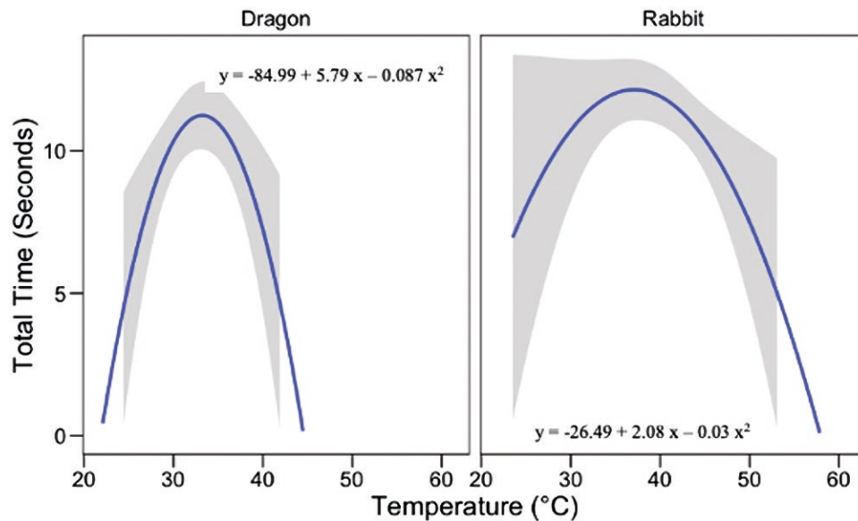
Fig. 5. Regressions of the relationship between substrate surface temperature from each research site and the time adult Cicindelia haemorrhagica spent at those temperatures. The line is the fitted values using the total time averages from each research site. The gray shaded area represents the 95% CI for the average value.
