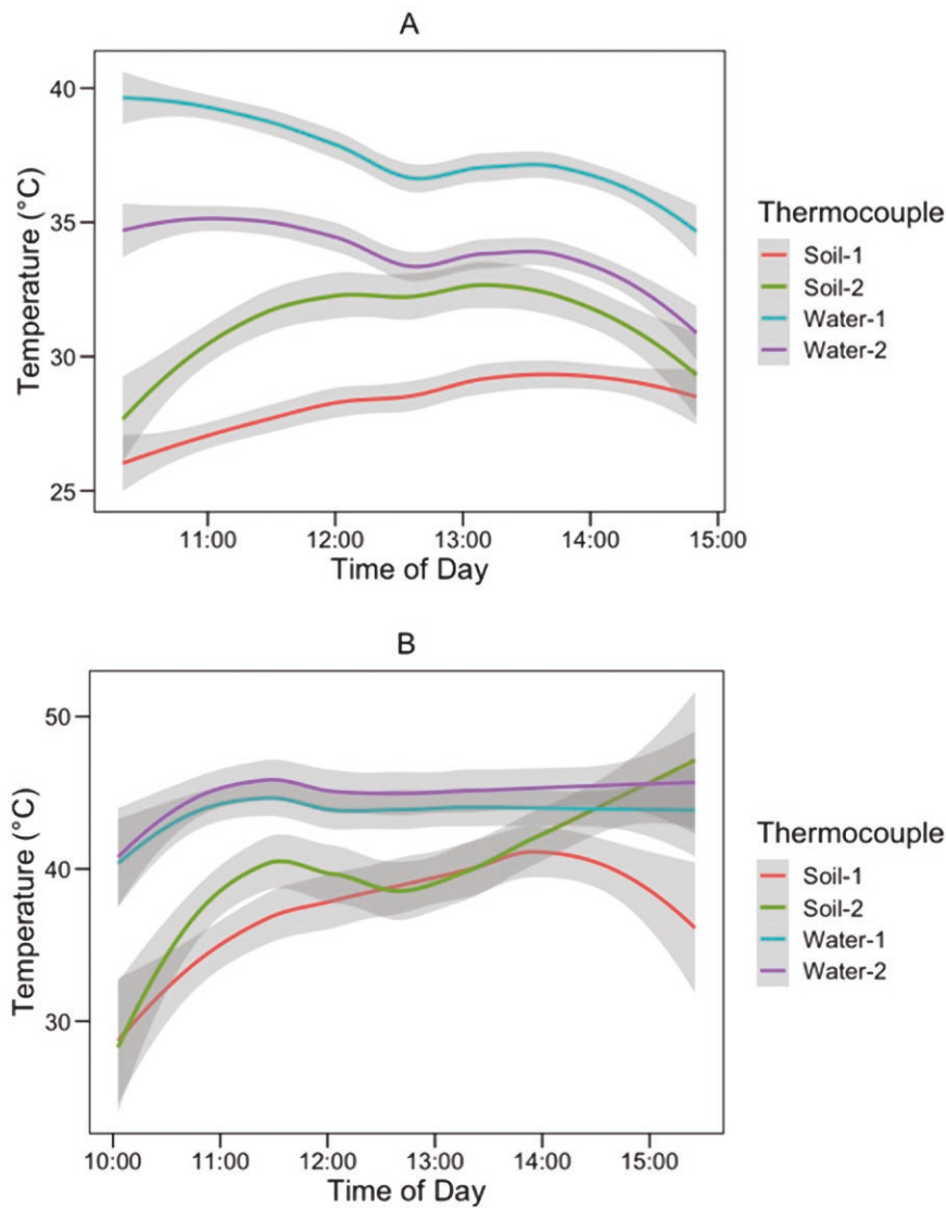
Fig. 6. A) Average temperatures during periods of observation at Dragon Spring recorded by thermocouples. B) Average temperatures during periods of observation at Rabbit Creek recorded by thermocouples.
