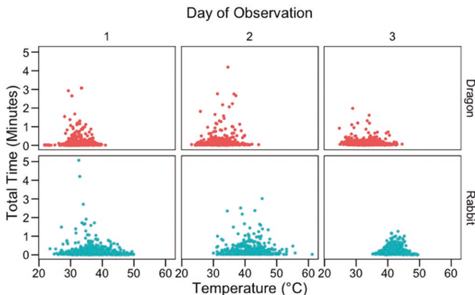
Fig. 4. Surface temperatures for each day of recording from Dragon Spring and Rabbit Creek. Each point represents the time spent by one adult Cicindelia haemorrhagica at a specific surface temperature.
