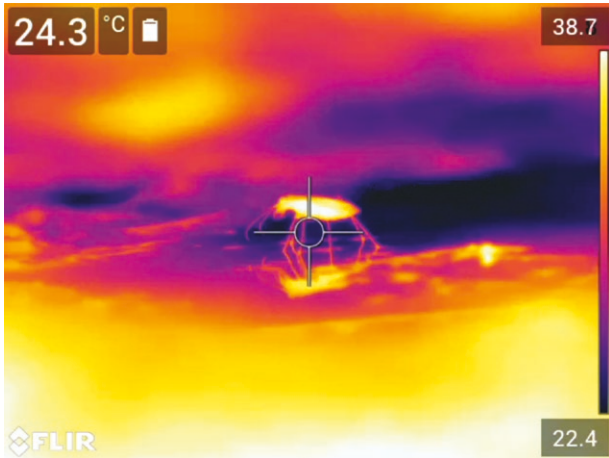
Fig. 1. A still image from the thermal video recording. The reflection of the beetle on the substrate is the more accurate surface temperature of the substrate not influenced by solar reflection and was the target area for measurement when analyzing the temperature-time relationship data in the recordings. Video still by JL Bowley.
