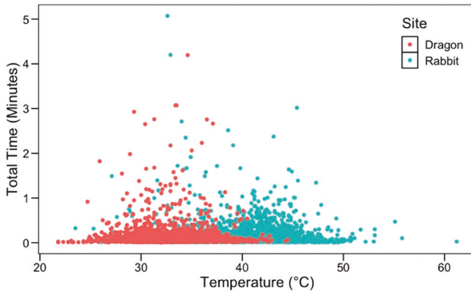
Fig. 3. Surface temperatures for each research site. Each point represents the time spent by one adult Cicindelia haemorrhagica at a specific surface temperature.
