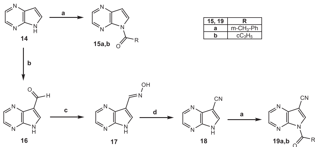
Scheme 4. Reagents and Conditions: (a) R-COCl, Et 3 N, anhydrous CH 2 Cl 2 , 0 °C, 2 h, then r.t., 2 h; (b) HTMA, glacial CH 3 COOH, reflux, 2 h; (c) NH 2 OH-HCl, H 2 O, 60 °C, 30 min; NaHCO 3 , reflux, 4 h; (d) POCl 3 , reflux, 2 h.
