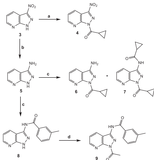
Scheme 2. Reagents and Conditions: (a) dry THF, NaH, 0 °C, 30', then \text{C}_3\text{H}_5\text{-COCl} , r.t., o/n; (b) HCl 37%, \text{SnCl}_2 \cdot 2\text{H}_2\text{O} , r.t., 30'; (c) \text{Et}_3\text{N} , DMF/1,4-Dioxane, R-COCl, 50 °C, 4 h; (d) \text{CH}_3\text{COCl} , \text{Et}_3\text{N} , anhydrous \text{CH}_2\text{Cl}_2 , 0 °C, 2 h, then r.t., 2 h.
