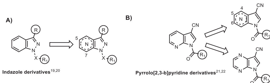
Fig. 1. Indazole and pyrrolo[2,3- b ]pyridine derivative modification.
