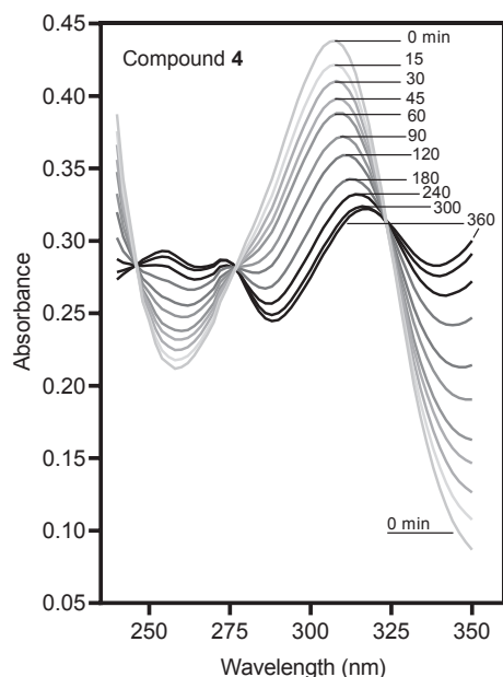
Fig. 2. Analysis of changes in compound absorbance resulting from spontaneous hydrolysis of 4 . The changes in absorbance spectra of the compounds (20 \mu M in 0.05 M phosphate buffer, pH 7.4, 20 °C) were monitored over time in solution.
