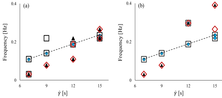
Figure 11: Dominant frequencies for \alpha (open black squares), \hat{\gamma}_h (closed blue circles), \hat{\gamma}_l (closed black triangles) and \hat{\gamma}_{true} (open red diamonds) for (a) protocol 1 (no pre-shear) and (b) protocol 2 (with pre-shear). Dashed lines correspond to the rotationally correlated frequencies.
