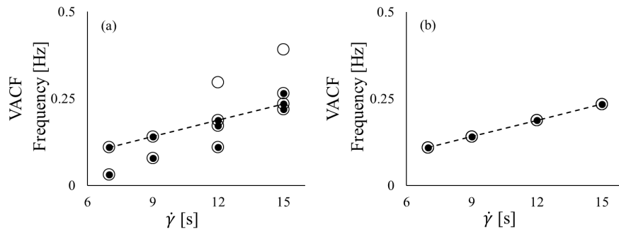
Figure 12: The dominant frequencies in the velocity autocorrelation function (VACF) spectra plotted as a function of applied shear rate for (a) the velocity in the spatial center of the high shear band and (b) the velocity in the spatial center of the low shear band. Filled black circles are protocol 1 and open circles are protocol 2. Dashed lines correspond to the rotationally correlated frequencies.
