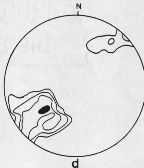
d. Sourdough Creek (S-N) 22, N 39 E, 44, S 41 W. 46 points. Contours, 2%, 4%, 15%, per 1% area.
