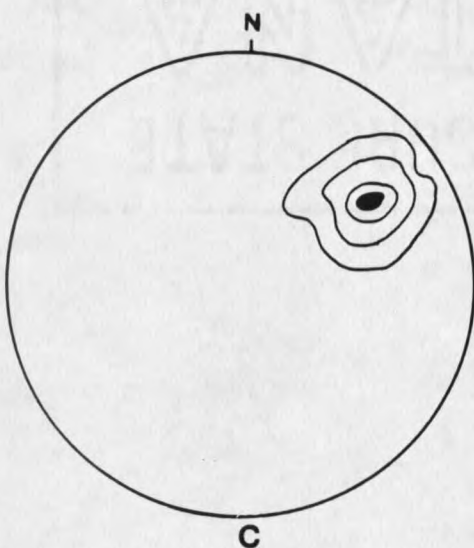
c. Sourdough Creek (S-12) 25, N 56 E. 18 points. Contours, 1%, 5%, 15%, 20%, per 1% area.
