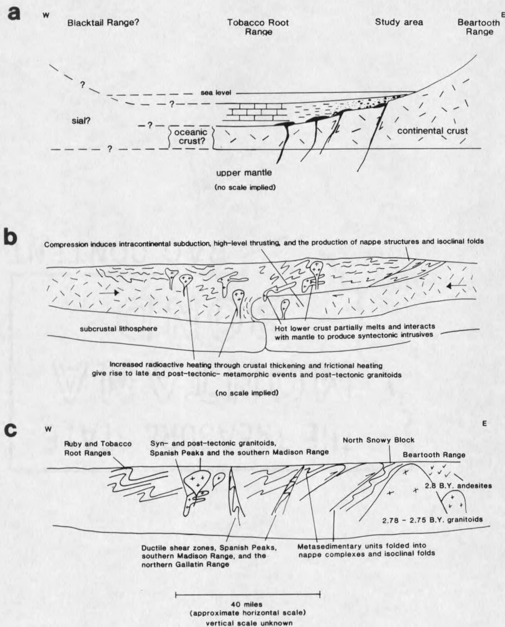
Figure 24. Suggested stages in the Archean tectonic evolution of southwest Montana (excluding the Beartooth Range) involving A-type (continental) subduction. a) Pre-tectonic setting. b) Compressional tectonics resulting from A-type subduction (modified from a model of the Pan-African Damara Belt by Kroner, 1981). c) Structural and lithologic features within southwest Montana Archean exposures.
