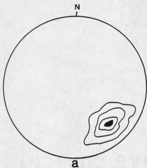
a. Leverich Creek (L-1) 25, S 67 E. 32 points. Contours, 1%, 3%, 10%, 20%, per 1% area.
