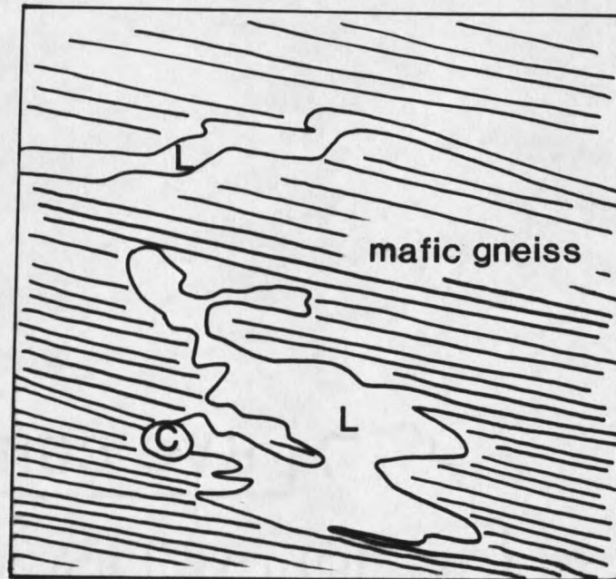
Figure 5. Mobilized leucosomes (L) within mafic gneiss (mesosome). Lens cap (C) diameter = 5 cm.
