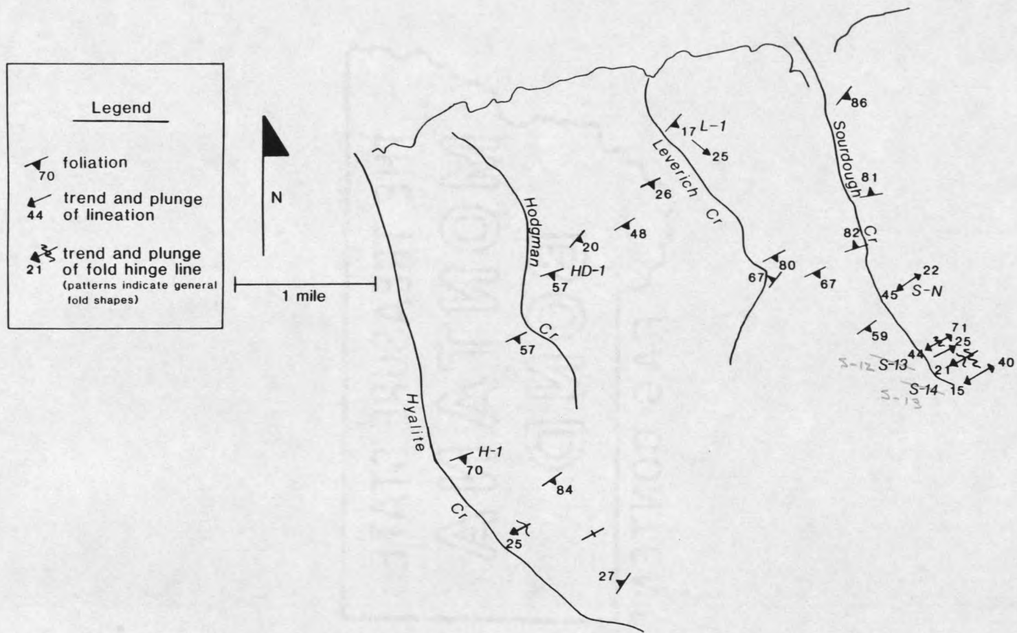
Figure 16. Generalized structure map for study area. (Lettered locations explained in text and in stereonet captions. See also Appendix A.)
