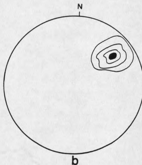
b. Sourdough Creek (S-13) 40, N 63 E. 25 points. Contours, 1%, 5%, 10%, 15%, per 1% area.
