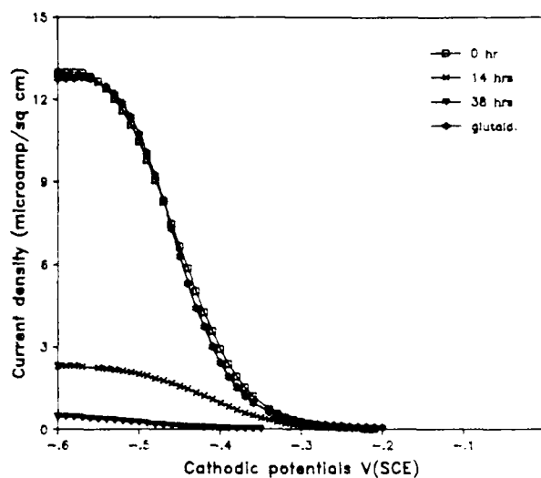
FIGURE 8. The results of cathodic polarization measurements at corrosion coupons in an open channel flow reactor.
