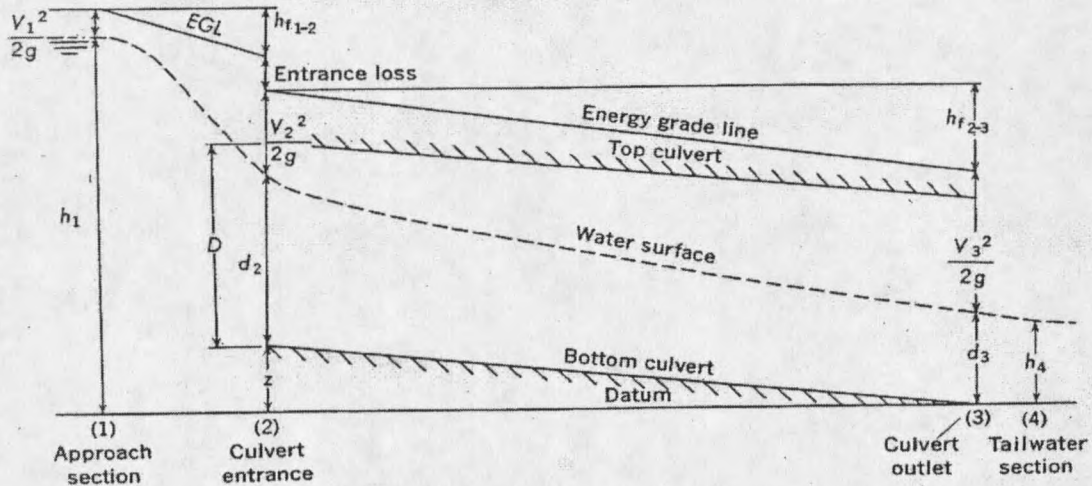
Figure 1. Culvert Cross Sectional Diagram
