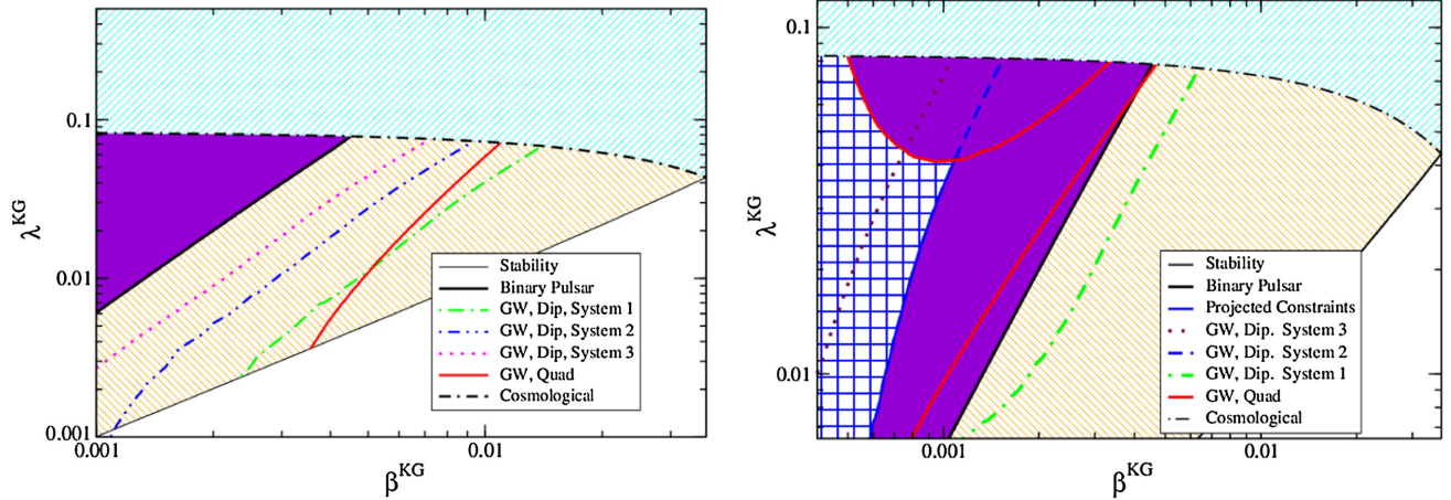
FIG. 3 (color online). Projected constraints on \beta^{\text{KG}} and \lambda^{\text{KG}} via a gravitational-wave detection by third-generation detectors ET (left panel) and DECIGO (right panel), consistent with GR. The contours are produced by finding the values of \beta_{\text{OPN,KG}} and \beta_{\text{-IPN,KG}} are met exactly. Thus, the regions above (or bounded by) the contours are the allowed regions for \beta_{\text{KG}} and \lambda_{\text{KG}} . The dark (purple) shaded region is the allowed region from binary pulsar observations, as calculated in [4,5], the light (cyan) shaded region is that allowed by stability, and the mid (orange) shaded region is the allowed region from cosmological constraints. Note that the constraints producible via second-generation gravitational-wave detection are entirely outside the region allowed by requiring stability and cosmological constraints.
