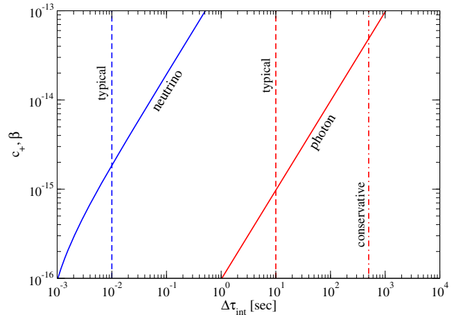
FIG. 4 (color online). Projected constraints on c_+ and \beta_{\text{KG}} , assuming a coincident gravitational wave and electromagnetic observation. The vertical (dashed) lines show conservative and typical estimates for the intrinsic uncertainty in the time of arrival of electromagnetic radiation. The solid lines are the solutions to Eq. (119) for c_+ and \beta_{\text{KG}} . The intersection of the solid and dashed lines shows the projected constraints.
