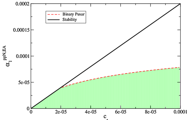
FIG. 6 (color online). In the figure above, we show the allowed regions in parameter space for the coupling parameters c_- and \alpha_1^{\text{ppN}} in Einstein-Æther theory based on binary pulsar observations, in the case of a restriction on the speed of gravity through coincident gravitational-wave or electromagnetic detection. For our analysis, we used observational bounds on the values of \dot{P}/\dot{P}_{\text{GR}} to bound the magnitude of \mathcal{A} . We chose a representative case, PSR J1141-6545 [65]. We also considered pulsars: PSRJ03848 + 0432 [66], PSR J0737-3039 [67], and PSR J1738-0333 [68], and found comparable results.
