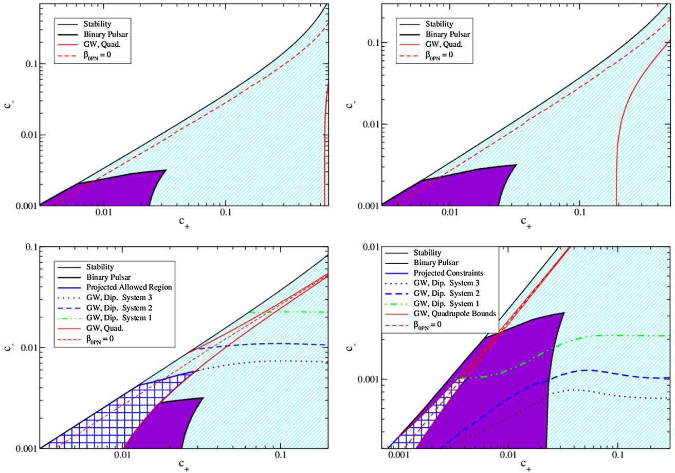
FIG. 2 (color online). Projected constraints on the (c_+, c_-) space, given a gravitational-wave detection by aLIGO, LIGOIII, DECIGO and ET (clockwise from top left) consistent with GR. We inject a simulated signal produced by the quasicircular inspiral of nonspinning NSs at a luminosity distance of 270 Mpc. The contours are produced by finding the values of (c_+, c_-) that satisfy Eqs. (111) and (112). Thus, the regions below the contours are the allowed regions for c_+ and c_- . One cannot place constraints from \beta_{-1PN,EA} with aLIGO or LIGOIII because the measurement errors on the masses are too large due to degeneracy with \beta_{0PN,EA} . The dark shaded (purple) region is the allowed region from binary pulsar observations, as calculated in [4,5]. Note that the gravitational-wave projected constraints are less strict by orders of magnitude than those calculated with binary pulsar observations.
