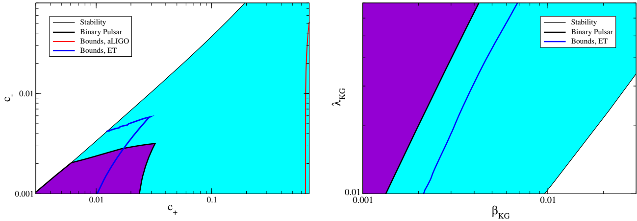
FIG. 1 (color online). Projected constraints on c_+ and c_- (left panel), and \beta_{\text{KG}} and \lambda_{\text{KG}} (right panel) assuming gravitational-wave observations from the quasicircular inspiral of nonspinning NSs consistent with GR, at a luminosity distance of 270 Mpc. This corresponds to SNRs 10 and 130 for aLIGO and ET, respectively, averaging over sky location. The regions below and to the left of the contours are the allowed regions for the respective coupling parameters. The purple shaded region is the allowed region from binary pulsar and cosmological observations, as calculated in [4,5], and the lighter shaded region is the allowed region from stability. As a representative case we show here contours produced given a detection with aLIGO and with ET. In the khronometric gravity case, the constraint from aLIGO is outside the scale of the plot.
