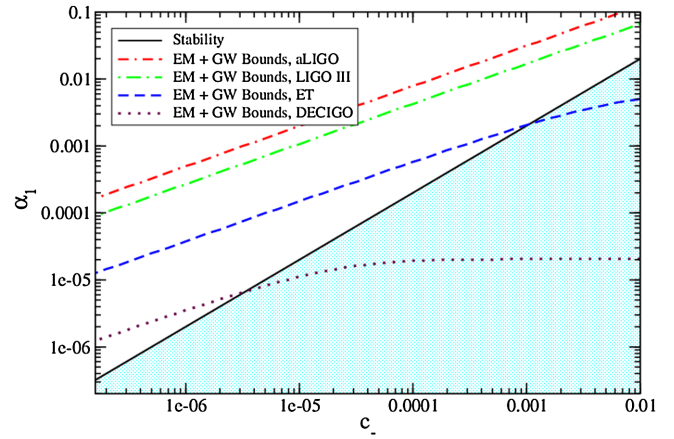
FIG. 5 (color online). Bounds on (\alpha_1^{\text{ppN,EA}}, c_-) , given a constraint on the speed of gravity through a coincident gravitational-wave-electromagnetic observation. Note that in the region for c_- allowed by stability, the constraints on \alpha_1^{\text{ppN,EA}} are approximately 2 orders of magnitude weaker than current Solar System constraints ( \alpha_1^{\text{ppN,EA}} < 10^{-4} ), and of comparable size to the bounds on \alpha_1^{\text{ppN,EA}} found in [64]. For third-generation detectors, such as ET, the constraints become 1 order of magnitude stricter than current Solar System constraints.
