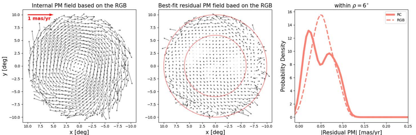
Figure A2. Same as Figure 3, but for the RGB sample. The first two panels show the internal motion field and residual PM field of the RGB stars. In the third panel, we compare the distribution of the residual PM amplitudes of the RC (solid curve) and RGB (dashed curve) stars within the inner 6^\circ .
