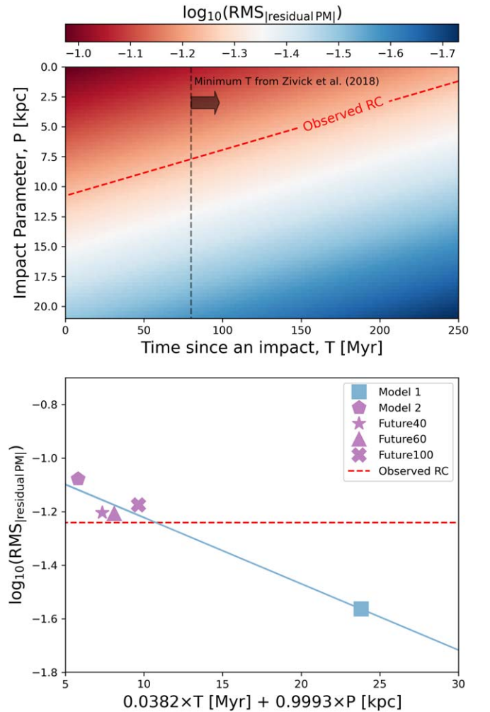
Figure 8. Top: predicted \log_{10} of an rms of a residual PM amplitude distribution as a function of impact timing ( T ) and impact parameter ( P ). The prediction is made from the best-fit plane of (T, P, \log_{10}(\text{rms})) using the five simulated LMCs. The red dashed line indicates the one-dimensional family of (T, P) that is consistent with the RC-based observational results. The black dashed line denotes the minimum T from the LMC–SMC orbit modeling (Zivick et al. 2018). Bottom: the edge-on view of the best-fit plane (blue solid line) and distribution of the five simulated LMCs around the plane. The observation agrees reasonably well with all three future models (Future40, Future60, and Future100).
