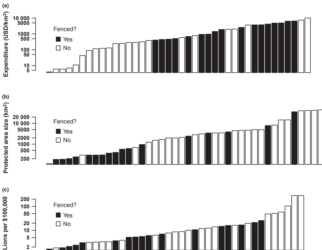
Figure 2 Lion populations with and without perimeter fences, ranked by (a) management expenditure per \text{km}^2 , (b) protected area size and (c) lions conserved per $100 000 of management expenditure. Unfenced populations were larger, were managed with smaller budgets (per unit area), and were more cost-effective. The ordinate is logarithmically scaled in all panels. In panel C, we assume that lion density (like other ecological attributes) responds directly or indirectly to the level of management expenditure used to conserve an area. If lion density was estimated for a subset of a protected area, we assume similar effects of expenditure on lion density (but not equal density) inside and outside the study site. The significantly larger number of lions conserved per dollar of management expenditure in unfenced populations runs opposite to the primary inference of Packer et al. , although they did not present any statistical test of cost-effectiveness.
