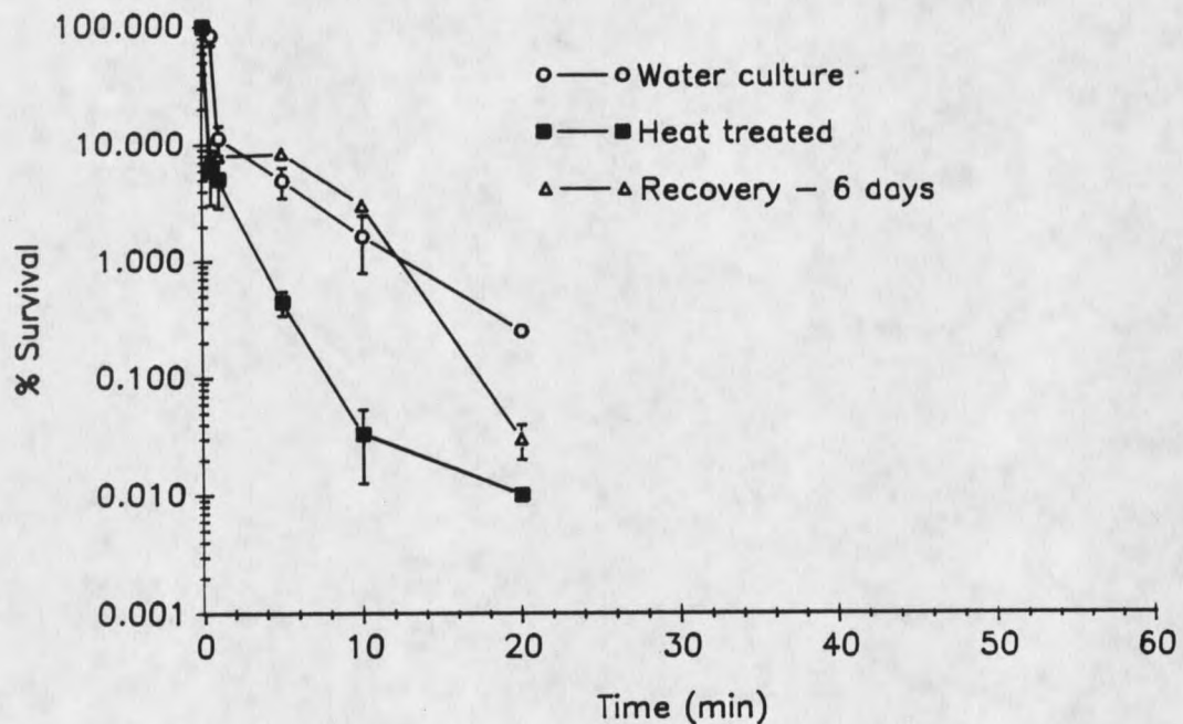
Figure 6. Iodination (16 ppm) of heat-treated legionellae and heat-treated legionellae after recovery (at 35 C for six days).
