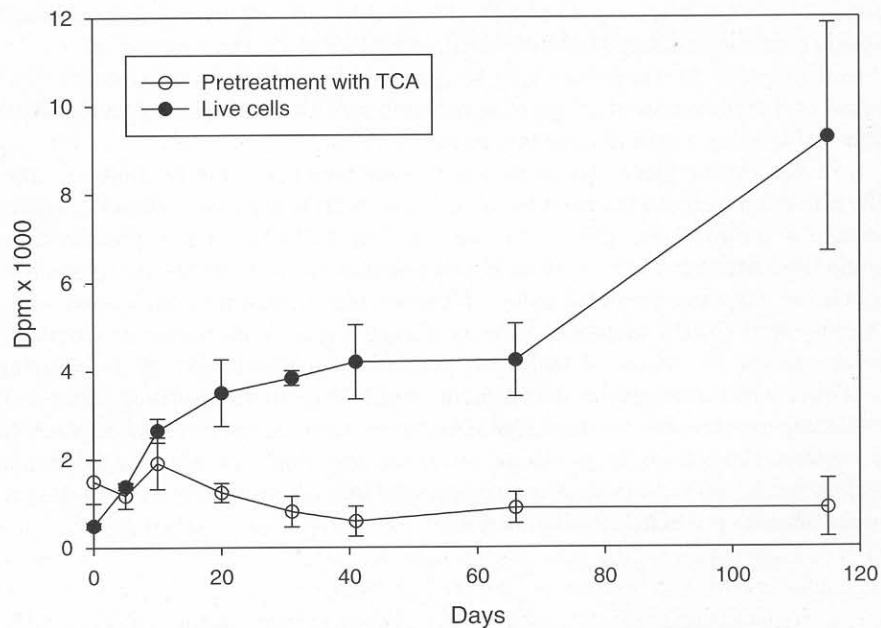
Fig. 4.4 Incorporation of [ ^3\text{H} ]thymidine into TCA-precipitable material by frozen suspensions of Sporosarcina species TGTB5-5B at -15^\circ\text{C} . The experiment was conducted for 115 days in a media with a total dissolved solid concentration of \sim 10^{-4} M. Freezing conditions and experimental details were as described by Christner (2002)
