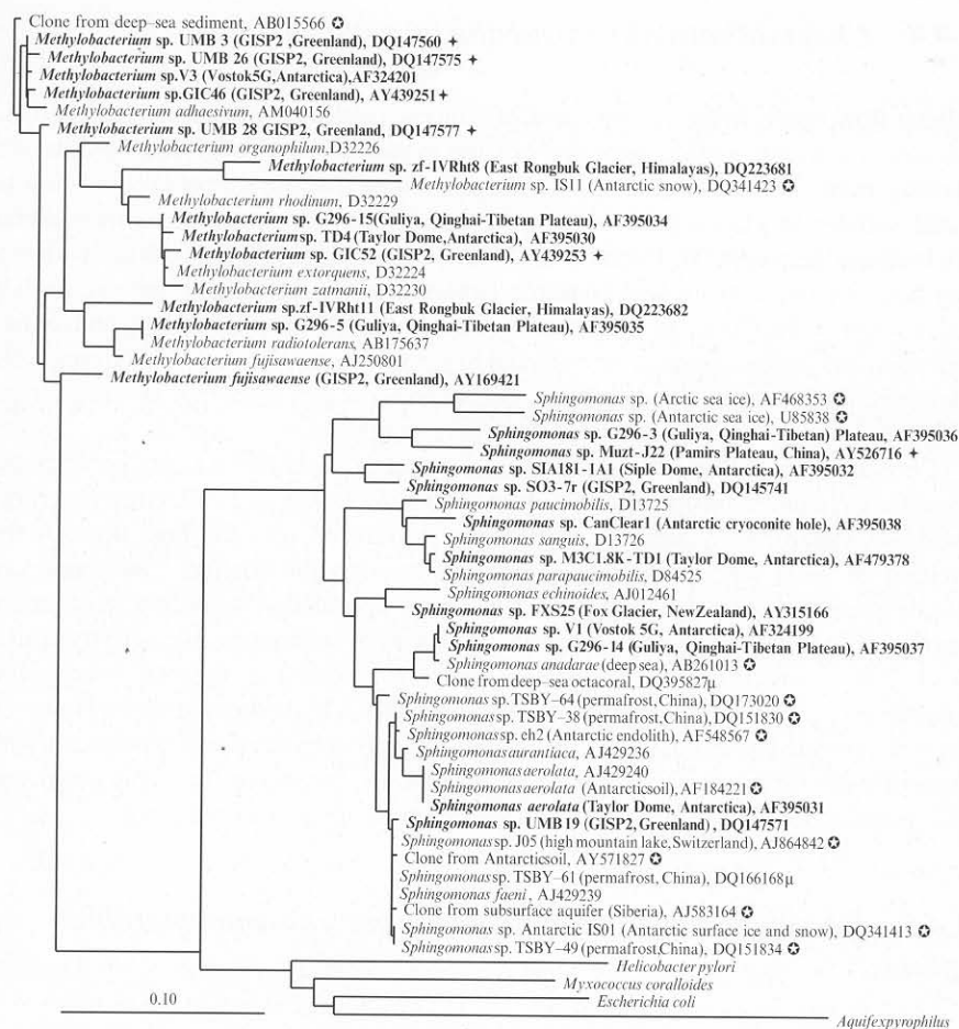
Fig. 4.6 Phylogenetic analysis of small subunit (16S) rRNA gene sequences from Methylobacterium and Spingomonas species isolated from glacial and subglacial environments (in bold). The sequences were aligned on the basis of secondary structure and a 1,220-nucleotide mask (120–1,377, Escherichia coli 16S rRNA gene numbering) was used to generate the tree using the maximum likelihood method. The scale bar represents 0.1 fixed substitutions per nucleotide position. Branches labeled with a white star in a black circle are isolates and cloned sequences obtained from permanently cold and frozen environments; a black star designates lineages for which only short sequences (488–720 nucleotides) are available, and these sequences were added to the tree using the ARB parsimony insertion tool ( http://arb-home.de/ ). The source environment is shown in parentheses, followed by the GenBank accession number
