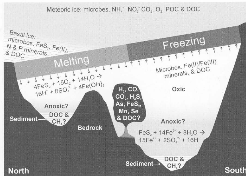
Fig. 4.2 Hypothetical scenario for chemically-driven biogeochemical reactions that could be used for bioenergetics in Lake Vostok. Inputs to the system (northern portion of the lake; see text) are through the melting of basal ice, which contains crushed sulfide and iron minerals and organic material from the bedrock, and glacial ice, which provides a constant supply of oxidants ( O_2 and NO_3^- ), nutrients, and organic material. Microbes, minerals, and organic carbon are removed from the lake via the accretion ice (southern portion of the lake). Shown are oxic and anoxic chemolithotrophic reactions (i.e., metal sulfide oxidation) that have been documented in Alpine and Arctic subglacial environments (Bottrell and Tranter 2002; Tranter et al. 2002; Wadham et al. 2004). Fault vents may be present in the shallow embayment of the lake (Bulat et al. 2004), which could introduce significant amounts of thermal energy, geochemical energy, and organic carbon to the lake. If biotic and/or abiotic oxygen sinks exist in the lake, then the deep waters and sediments would be expected to be anaerobic. POC = particulate organic carbon; DOC = dissolved organic carbon
