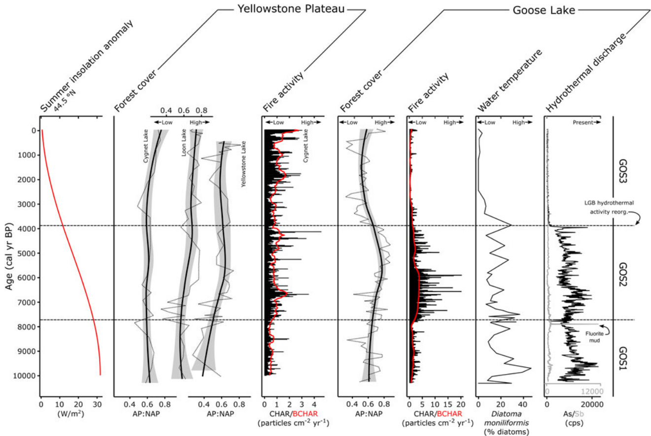
Figure 7. Comparison plot of proxy data from the Goose Lake composite core YNP4-GOS18 with other sites on the Yellowstone Plateau (Cygnnet Lake, Yellowstone Lake). Seasonal insolation anomaly calculated for 44.5°N (Laskar et al., 2004). Forest cover at sites without significant surficial hydrothermal activity (Whitlock, 1993; Whitlock et al., 1995; Theriot et al., 2006) is plotted as standardized AP:NAP ratios ( AP - NAP / AP + NAP ; dotted line) with loess smoother (solid line with shaded 95% confidence interval); fire activity at Cygnnet Lake (Millspaugh et al., 2000; CHAR in black, BCHAR in red). Forest cover and fire activity plots for Goose Lake are juxtaposed with diatom and geochemical indicators of hydrothermal conditions. (For interpretation of the references to color in this figure legend, the reader is referred to the web version of this article.)
