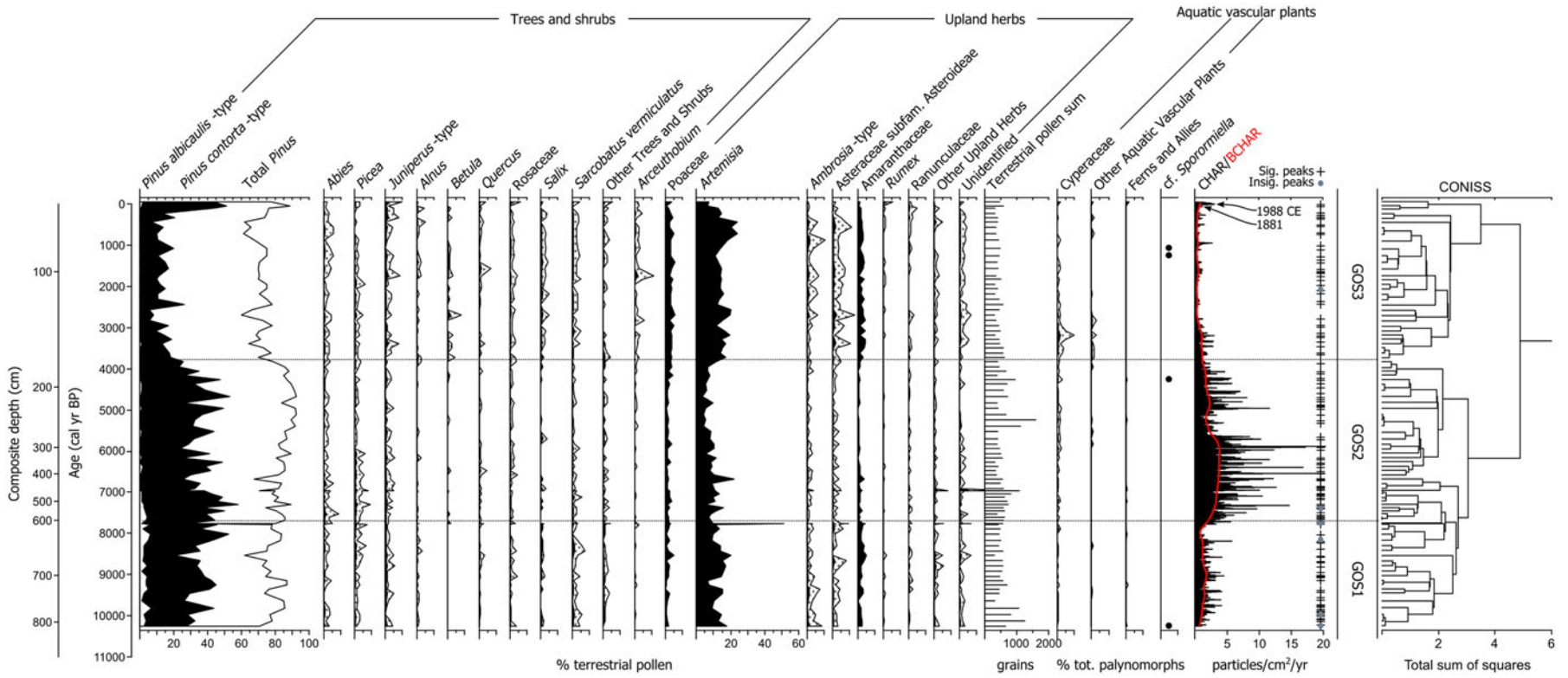
Figure 5. (color online) Percentage diagrams of major pollen types and spores (>1%), total sum of terrestrial pollen, and charcoal data (CHAR and BCHAR) with significant and insignificant peaks from Goose Lake composite core YNP4-GOS18. Where present, curve exaggeration is 5x. Zone delineation is supported by CONISS dendrogram constructed with percentage data from terrestrial pollen.
