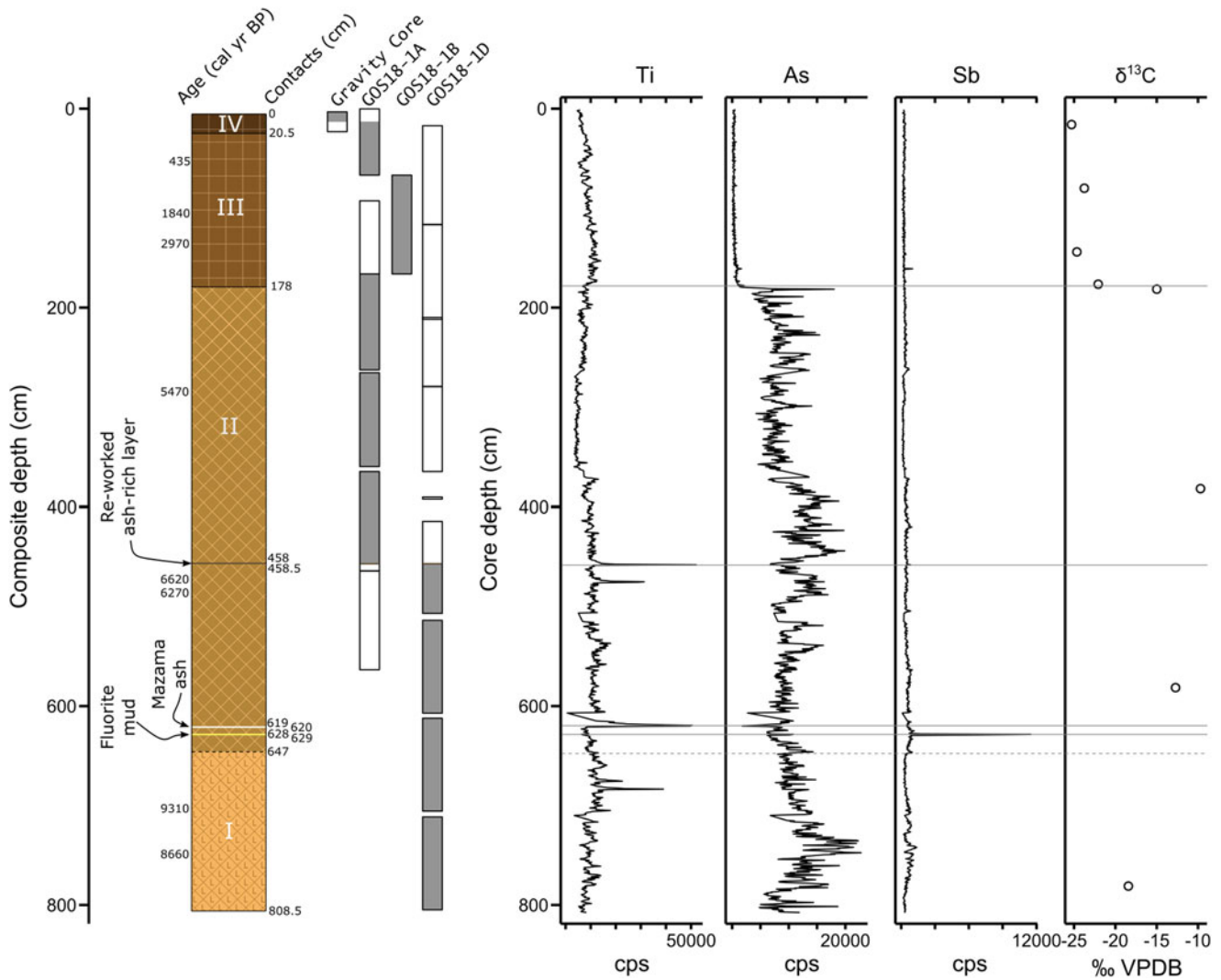
Figure 2. (color online) Lithology and geochemistry of the composite Goose Lake core YNP4-GOS18. The core was divided into four stratigraphic units: (I) Indistinctly laminated diatomaceous ooze with clay; (II) Laminated diatomaceous ooze with sapropel and minor, fragmental plant remains, punctuated by antimony-rich fluorite mud (629–628 cm depth), the Mazama ash (620–619 cm depth), and a reworked ash-rich siliciclastic deposit (458.5–458 cm depth); (III) Thinly bedded diatom ooze with sapropel; (IV) Massive diatomaceous sapropel with high water content. The diagram of the composite core is based on core depth, except the correlation between GOS18-1A and GOS18-1D, which was made using the reworked Yellowstone ash. Shaded core drives (gray) were used in developing the composite record. Abundant arsenic is associated with geothermal water influx; and antimony-rich fluorite mud (619–618 cm depth) is definitively of hydrothermal provenance. Higher \delta^{13}\text{C}_{\text{sediment}} (‰ VPDB) likely indicates an admixture with hydrothermally degassed carbon.
