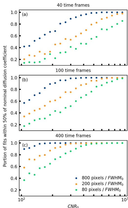
FIG. 6. Variations in spatial and temporal resolution for a simulation with a diffusion length of 0.01FWHM_0 , a duration of one lifetime, and a spatial domain width of 5FWHM_0 over a range of CNR_0 values between 100 and 1000. Increasing the number of spatial pixels or temporal frames improves the precision of diffusion coefficient estimates. (a) 40 time frames, (b) 100 time frames, and (c) 400 time frames.
