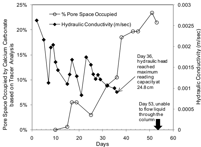
Figure 4. Relative decrease in pore space over time in the column (based on tracer analysis) and decrease in hydraulic conductivity observed over the first 36 days of the column experiment.
