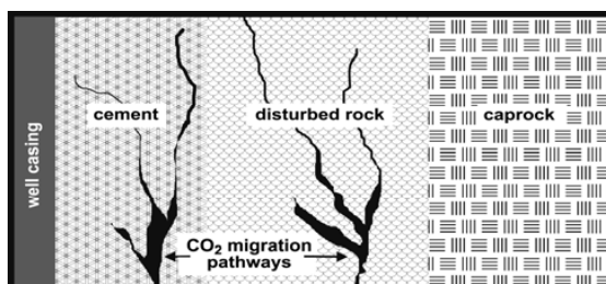
Figure 1. Schematic showing potential CO 2 leakage pathways in disturbed rock, cement and along well casing. This schematic represents the cement layer and disturbed rock at a location where the well passes through the cap rock, above the reservoir.
