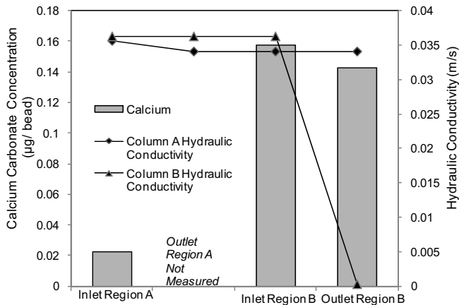
Figure 2. Distribution of Calcium Carbonate Deposits and Hydraulic Conductivity in 1 cm diameter, 2.5 cm long columns packed with 1 mm glass beads. Column A was injected with media containing 0.025 M \text{Ca}^{2+} and Column B with media containing 1.25M \text{Ca}^{2+} over 17 days. Plugging and homogenous calcium distribution (between inlet and outlet) was achieved in Column B. Plugging was not achieved in Column A.
