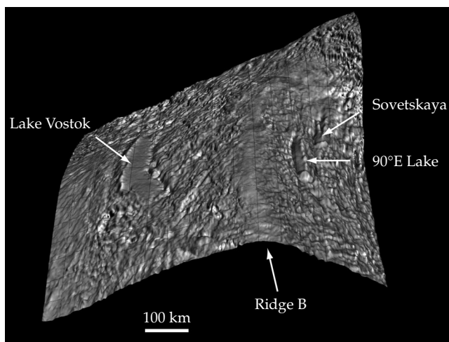
Figure 7.2 MODIS mosaic of Ridge B region including the 90°E and Sovetskaya lakes as well as Lake Vostok. Geographic north is to the bottom. See Bell et al. (2006) for details.
