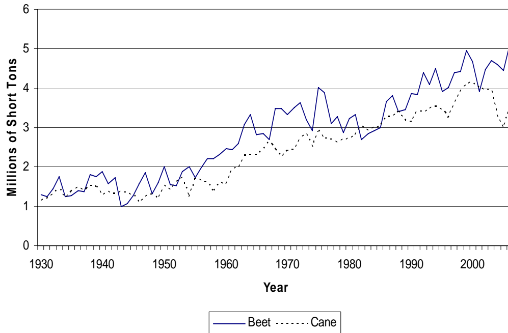
Figure 5. Beet versus cane sugar production, raw value, 1930-2006. (Data from USDA ERS Sugar Statistical Bulletins, various issues).
