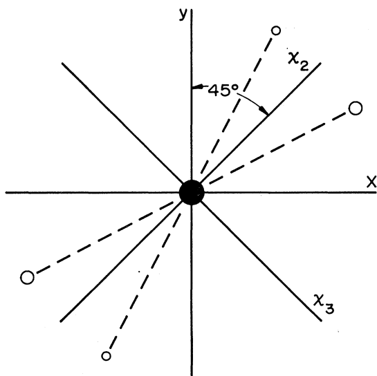
FIG. 1. Projection along z of environment of a thulium ion (filled circle) in a \text{Tm}-\text{AlO}_4-\text{Tm}\cdots chain running along the z axis, which is the \chi_1 axis for the susceptibility tensor for this thulium site. The \chi_2 and \chi_3 axes are oriented as shown. The large open circles are the bottom oxygens of the \text{AlO}_4 tetrahedron above the thulium ion, and the small open circles are the top oxygens of the \text{AlO}_4 below the thulium ion.
