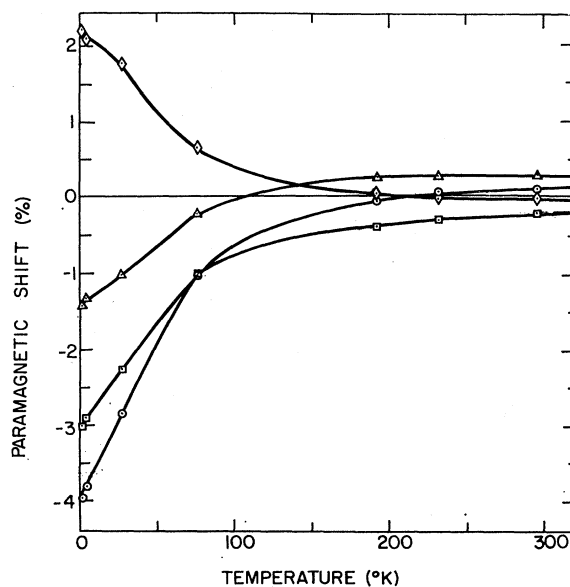
FIG. 4. Temperature dependence of the \text{Al}^{27} paramagnetic shifts \Delta H/H_0 . The a - and d -site shifts for H_0 parallel to the site axes are labeled \Delta and \circ , respectively, while the perpendicular shifts are labeled \diamond and \square .
