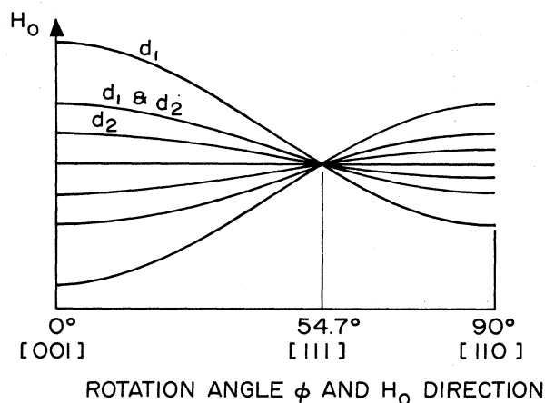
FIG. 3. General form of \text{Al}^{27} NMR spectra for rotation about [1\bar{1}0] axis. Paramagnetic shifts are ignored and only first-order quadrupolar splittings are included. Lines are labeled according to the site responsible for them.
