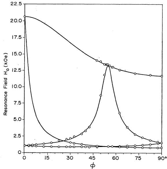
FIG. 2. Angular dependence of the \text{Tm}^{169} NMR fields \mathbf{H}_0 in the (110) plane for \nu=25,000 MHz and T=1.5^\circ\text{K} . The [100] and [110] directions are given by \phi=0^\circ and \phi=90^\circ , respectively. The three resonance fields for \mathbf{H}_0 along the \chi_1 , \chi_2 , and \chi_3 susceptibility tensor axes are 20.658, 0.750, and 11.644 kOe, respectively. The open circles are the measured NMR data and the solid lines are the calculated values.
