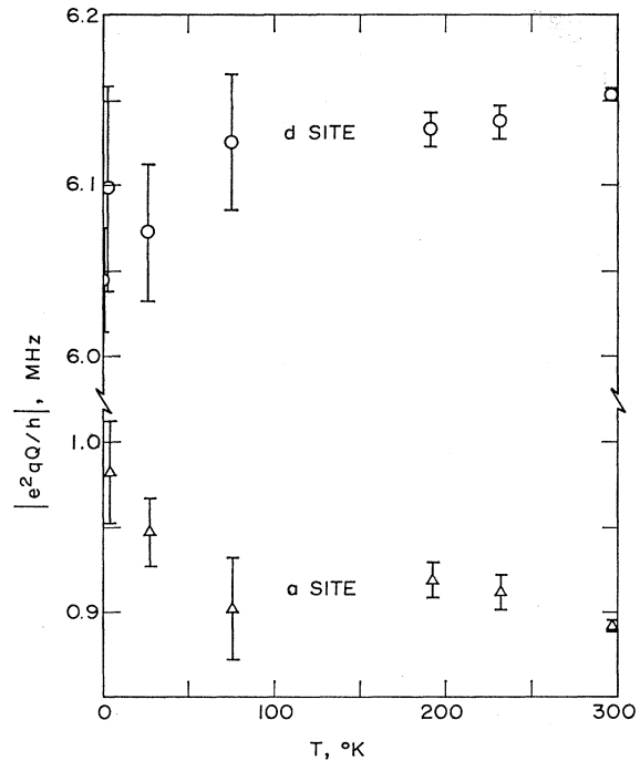
FIG. 6. Temperature dependence of \text{Al}^{27} quadrupolar coupling constants.
